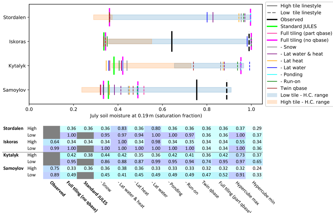
Figure 9. Average July soil moisture (2000–2016) at 0.19 m for the subtractive process-switching runs, where model processes are switched off individually starting from the base configuration of full tiling (no qbase) (thick pink). Solid lines show the high tile, and dashed lines show the low tile. Observations are shown in black, standard JULES is shown in green. The range across the Latin hypercube sampling runs (H.C. range) are shown by the boxes. The depths of the observations are as follows: for Samoylov, the rim was at 0.22 m and the centre was at 0.23 m, and for Iškoras the palsa and mire were both at 0.2 m.
