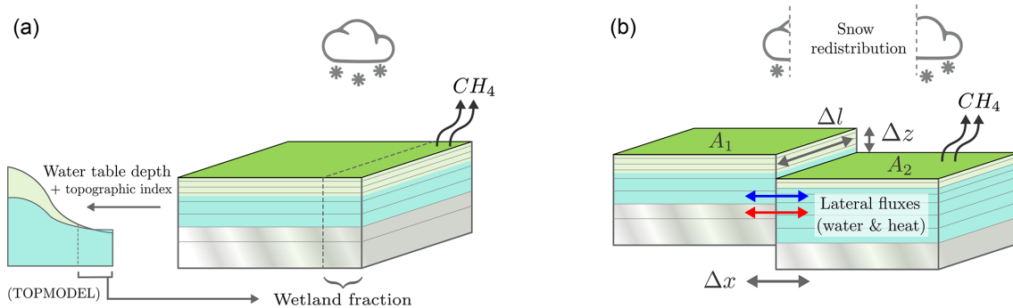
Figure 2. The implicit microtopography of standard JULES (a) vs. our explicit approach (b). In standard JULES (a), the grid cell consists of a single soil column representing the average values of soil temperature and carbon. These values are used to calculate a methane flux, which is then multiplied by a wetland fraction (diagnosed by TOPMODEL using the modelled water table depth and the grid cell topographic index). Our explicit approach (b) uses two soil tiles offset by an elevation difference to explicitly simulate areas differentiated by microtopographic processes. Model spatial parameters are shown in grey and are defined for individual sites in Table 2.
