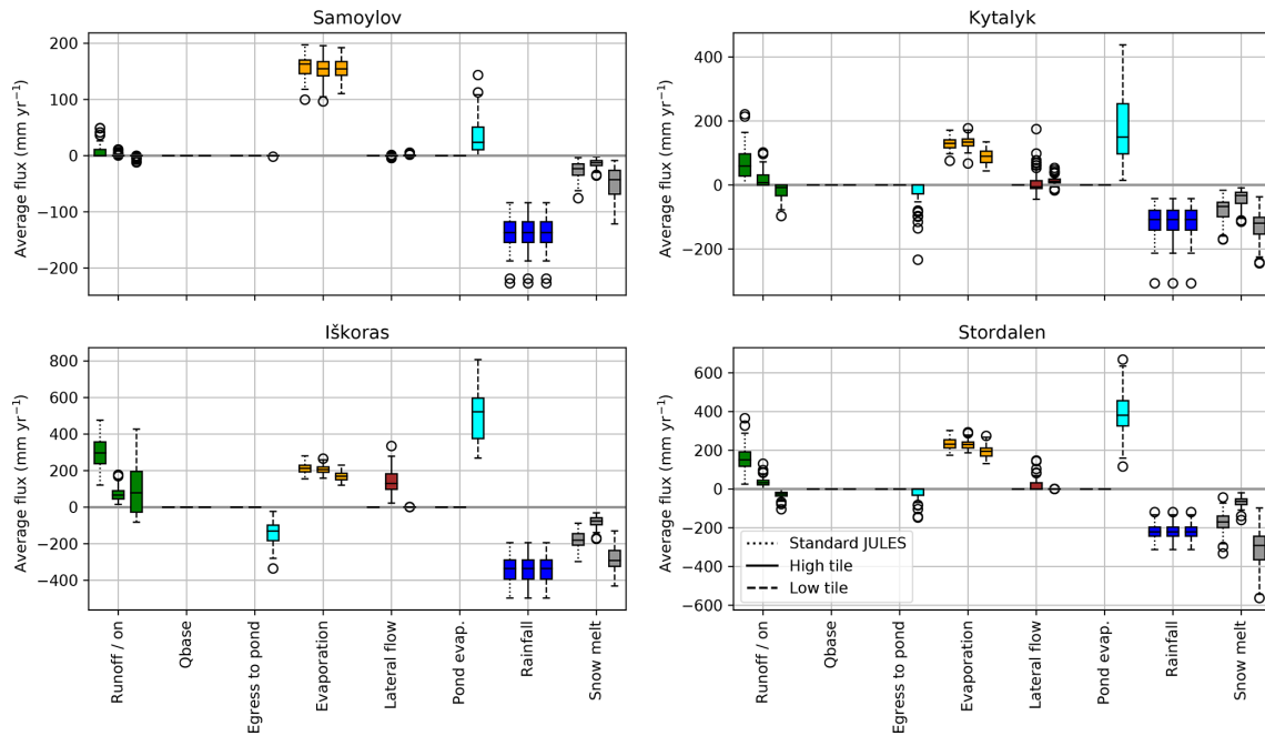
Figure 8. Boxplot of average yearly simulated moisture fluxes (1950–2016) for standard JULES and the two tiles for each site. Negative fluxes are incoming fluxes. Following the discussion in Sect. 3.2.1, this plot shows the configuration with qbase switched off.
