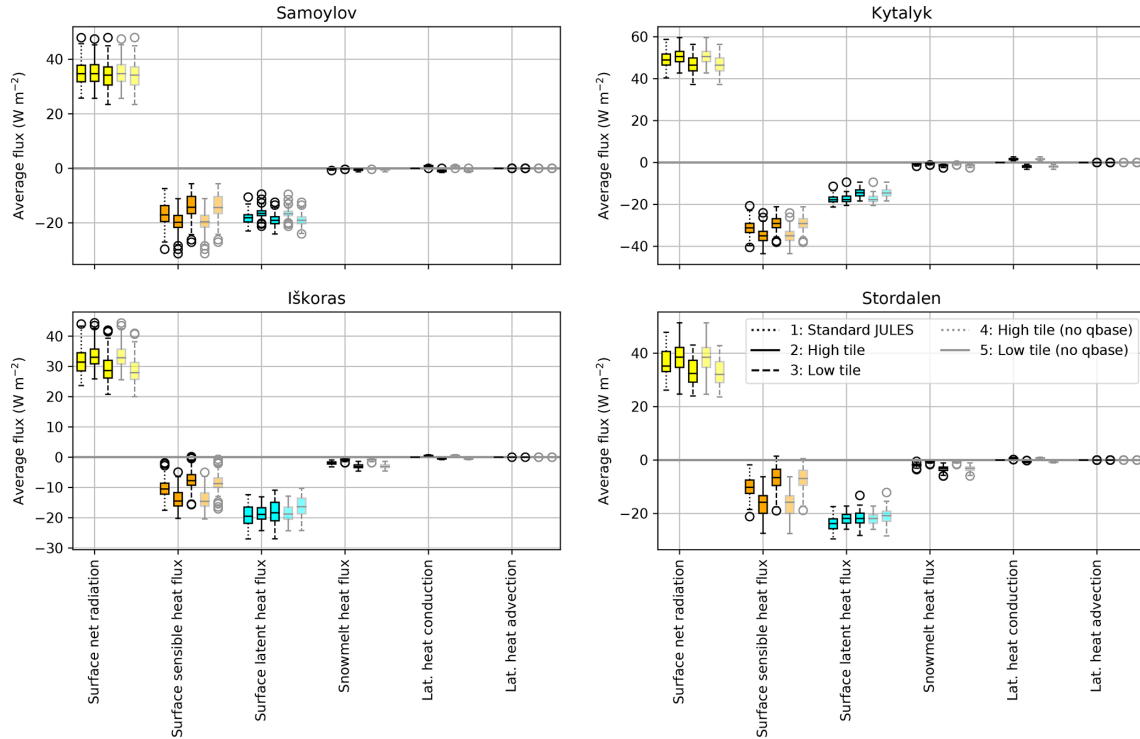
Figure B4. Average yearly simulated energy fluxes (1950–2016) for all sites with the qbase on configuration. Fluxes for the qbase off configuration are shown in grey for comparison.
