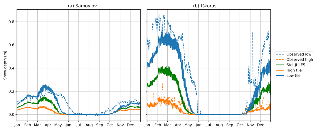
Figure 6. Climatology (2002–2016) of simulated vs. observed snow depths for Samoylov (a) and Iškoras (b), showing snow redistribution due to microtopography differentiating snow depths. Observed snow depths for Samoylov have been bias corrected using the signal during the snow-free season.
