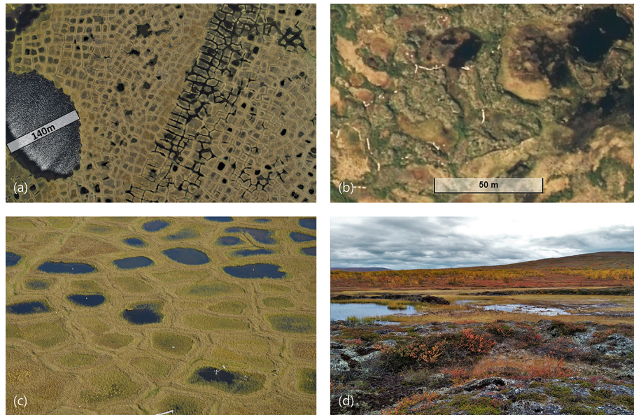
Figure 1. Ice wedge polygons at Samoylov (a, c, credit to Julia Boike for the images) and palsas and mire at Iškoras (b, © Kartverket, https://www.norgeskart.no/ ; d, credit to Noah D. Smith for the image) showing repetitive microtopography and some surface ponding. The observed low-centred polygons at Samoylov were on average 9.1 m in diameter and had rims 0.38 m above the centre. The observed palsa at Iškoras was 0.68 m above the mire. Some polygon rims can reach 1 m in height, while Palsas can reach larger elevations of around to 3 m.
