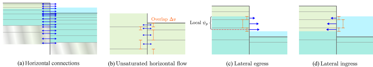
Figure 3. The lateral flow scheme. Fluxes are calculated horizontally for connections where layers overlap in the same manner as for the vertical fluxes in JULES (b). Fluxes are only permitted when they are into an unsaturated layer. Where high tile layers are above the low tile soil surface, flow can occur horizontally out of the soil (c) or from the pond to the soil (d).
