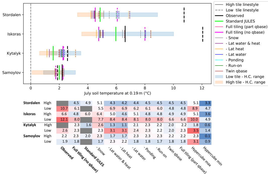
Figure 12. Average July soil temperature (2000–2016) at 0.19 m for the subtractive process-switching runs, where model processes are switched off individually starting from the base configuration of full tiling (no qbase) (thick pink). Solid lines show the high tile and dashed lines the low tile. The range across the Latin hypercube sampling runs (H.C. range) are shown by the boxes. The depths of the observations are as follows: for Samoylov, the rim was at 0.21 m, and the centre was at 0.2 m; for Kytalyk the rim was at 0.15 m, and the centre was at 0.25 m; for Iskoras, the palsa and mire were at 0.2 m; and for Stordalen the mire was at 0.25 m.
