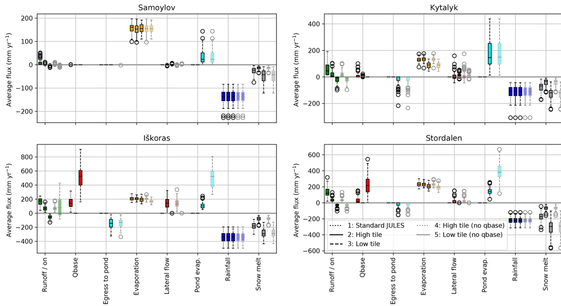
Figure B3. Average yearly simulated moisture fluxes for the period 1950–2016 for all sites with the qbase on configuration. Fluxes for the qbase off configuration (as in Fig. 8) are shown in grey for comparison.
