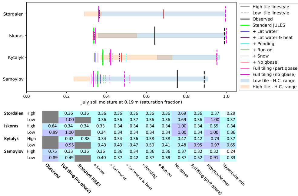
Figure B1. Average July soil moisture (2000–2016) at 0.19 m for the additive process-switching runs, where model processes are switched on one at a time starting from the base configuration of standard JULES (light green). The depths of the observations are as follows: for Samoylov, the rim was at 0.22 m and the centre was at 0.23 m, and for Iskoras the palsa and mire were both at 0.2 m.
