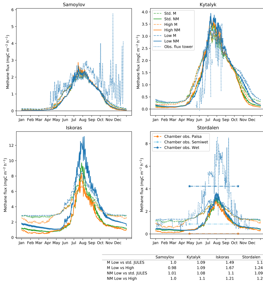
Figure 13. Climatology (2000–2016) of diagnosed methane fluxes calculated using modelled soil temperatures and observed soil carbon profiles, comparing fluxes from standard JULES and the low tile. Diagnosed methane fluxes for the high tile are shown for comparison only, as the drier soil would inhibit methane fluxes from these tiles. M is used to indicate the microbial methane model, and NM is used to indicate the non-microbial methane model. Methane chamber measurements for Stordalen are for 2002–2007 for the green season (days 119–288) and indicate the variability in methane fluxes due to hydrological conditions and thaw present at the site (Bäckstrand et al., 2010). Here, standard JULES has qbase switched on while tiled runs have qbase off.
