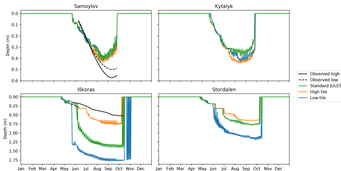
Figure 11. Climatologies (2002–2016) of modelled vs. observed thaw depths. Observed thaw depths for Iškoras were from 2019, Samoylov CALM thaw depths were from 2002–2016, grouped according to classes 1 and 3 and averaged using a third-degree polyfit across transects.
