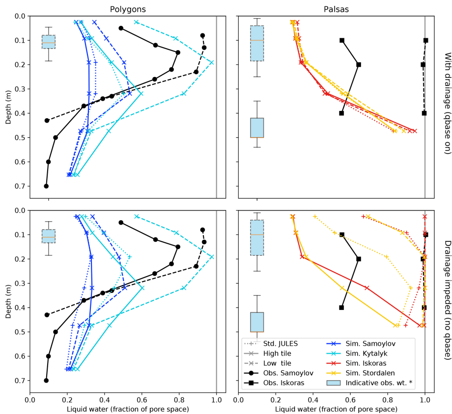
Figure 7. Average saturation profiles for July (2000–2016) showing the effect of tiling and also the importance of impeding mire drainage for palsa sites. Line colours show different sites while line styles differentiate high, low, and standard JULES. As points for simulations show the average saturation for the layer whose midpoint is at the depth shown, the simulated water table may be above a partially saturated point. Indicative observed water table depths for polygons are based on average July observed water table depths for a polygon centre (Boike et al., 2019). Indicative observed water table depths for palsas are from measurements of eight hollow points, not including ponded areas, and five palsa points in September 2007 (Klaminder et al., 2008). Water table depths for July from hollows in Işkoras were available but are not shown (Casper Tai Christiansen, Hanna Lee, unpublished data), as the range of values is contained within the range shown for Stordalen.
