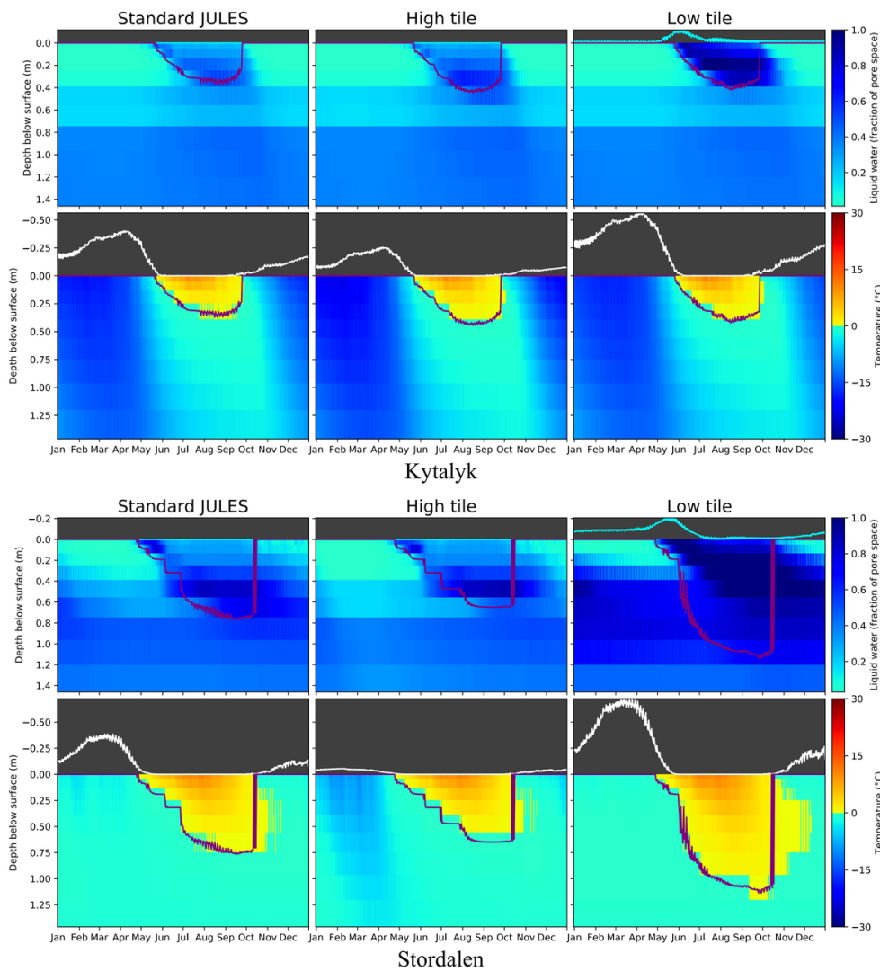
Figure B6. Climatologies (2002–2016) providing a comparison of observations with standard and tiled (no qbase) JULES for the polygon site Kytalyk and the palsa site Stordalen. The white line above the plots of soil temperature shows simulated snow depth, the cyan line above the plots of simulated soil moisture shows simulated pond depth, and the purple line shows thaw depth.
