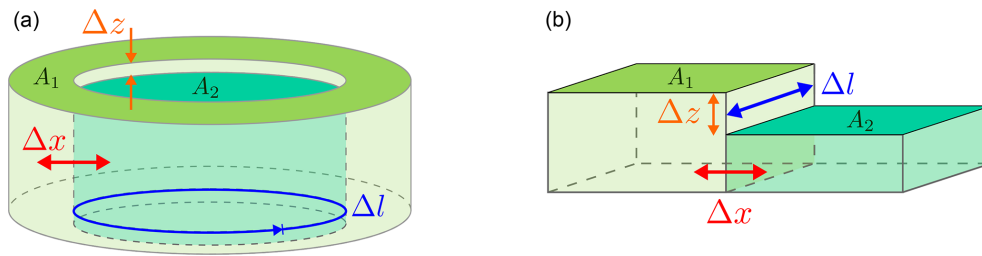
Figure 4. Geometries indicated by relationships between spatial model parameters for polygons (a) and palsa mires (b).
