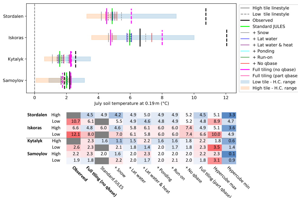
Figure B2. July soil temperature (2000–2016) at 0.19 m for the additive process-switching runs, where model processes are switched on one at a time starting from the base configuration of standard JULES (light green). The depths of the observations are as follows: for Samoylov, the rim was at 0.21 m, and the centre was at 0.2 m; for Kytalyk the rim was at 0.15 m, and the centre was at 0.25 m; for Iskoras, the palsa and mire were at 0.2 m; and for Stordalen the mire was at 0.25 m.
