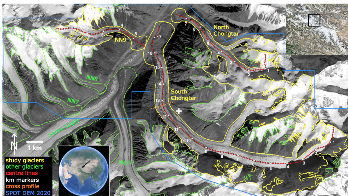
Figure 1. Overview of the study region showing the location of the Karakoram Mountains (inset, lower left) and of the study region (inset, upper right), outlines of the investigated glaciers (yellow) and other glaciers (green), centrelines (red), kilometre (km) markers (white), cross-profile line (orange), and extent of the SPOT 2020 DEM perimeter (blue). The white + near the centre marks the coordinates 35.9° N, 76.34° E. The satellite image in the background is the Landsat 8 panchromatic band acquired on 21 October 2020. Credits: Landsat – http://earthexplorer.usgs.gov (last access: June 2021); the two insets are screenshots from Google Earth (© Google Earth 2018).
