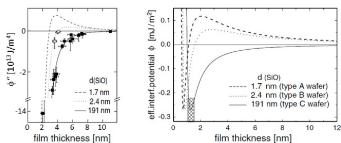
Fig. 9 Example of a reconstruction of the effective interface potential between a thin polystyrene film of the displayed film thickness and a Si wafer with variable SiO 2 -thickness d . Left: The second derivative of the effective interface potential as a function of film thickness. Data points display the observed spinodal wavelength \lambda of the dewetting polystyrene film. \phi''(h) and \lambda are connected via Eq. (4). Taken from Ref. [ 202].
