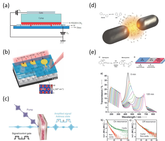
Fig. 8 Examples of recent experiments involving strong coupling. (a) An organic field-effect transistor coupled to the plasmon resonance from a periodic array in an aluminium layer. Taken from Ref. [ 174] (b) A gated device for manipulating Bloch polaritons generated in graphene encapsulated in hexagonal boron nitride using a plasmonic array in SiO 2 . Taken from Ref. [ 164] according to the Creative Commons license 175 (c) An organic polariton transistor. Taken from Ref. [ 157] (d) Suppression of photoisomerization by coupling to plasmonic modes between metallic nanoparticles. Taken from Ref. [ 176] according to the Creative Commons license 175 (e) Modification of photoisomerization rate of spiropyran-myocyanine by encapsulation in a Fabry–Pérot cavity. Taken from Ref. [ 177].
