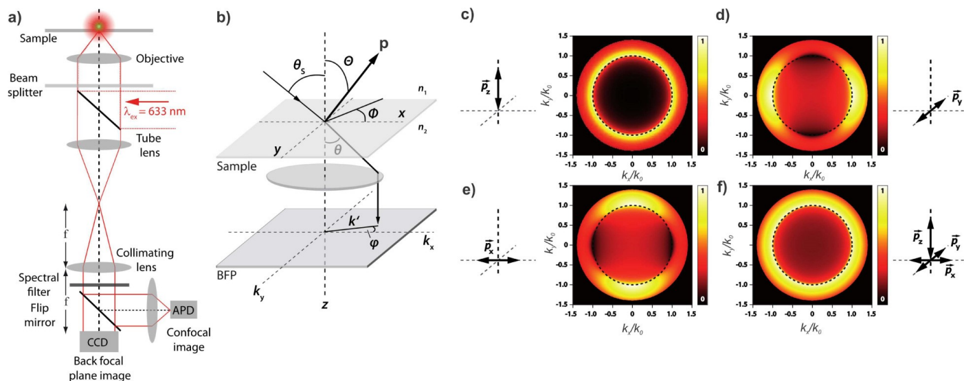
Fig. 11 (a) Example of a setup for back focal plane (BFP) imaging and spectroscopy. (b) Schematic diagram illustrating the mapping of dipoles from a sample onto the BFP. (c)-(f) Numerical calculations of the BFP intensity patterns for differently oriented dipoles. Figure unchanged taken from Ref. [ 241] according to the Creative Commons license 175
