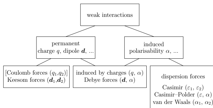
Fig. 2 Systematic overview of weak interactions (restricted to electric interactions) according to the type of interacting objects due to permanent (static) charges q , dipole moments \mathbf{d} , and higher-order of static multipoles, and due to induced (dynamical) dipole-polarisabilities \alpha , quadrupole-polarisabilities and higher-orders. Combining two single-particle properties and analysing the resulting interaction, one finds different forces depending on the combination of permanent-permanent, permanent-induced and induced-induced.
