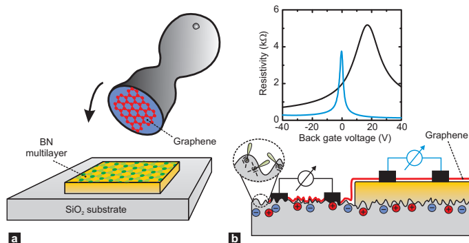
Fig. 6 Supporting graphene on hexagonal boron nitride (BN) substrates. a, Schematic showing how the graphene is transferred onto multilayer BN, which is supported on a SiO 2 substrate, with a stamping technique. b, A single piece of graphene (red) is supported by a SiO 2 substrate (left) and a flat BN multilayer (right). The corrugations, dangling bonds (inside a dashed circle) and charge inhomogeneities that are inherent to SiO 2 surfaces shift and broaden the resistivity peak of the graphene (black line in plot) relative to that of graphene on BN (blue line). Figure taken from Ref. [ 54].
