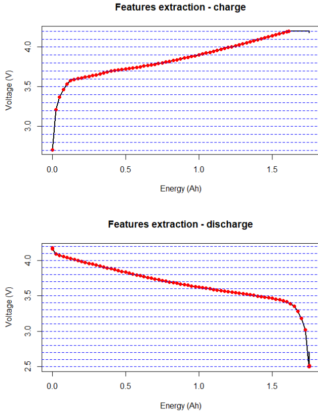
Figure 5. Energy throughput (Ah) across selected voltage ranges are calculated and used as explanatory variables
