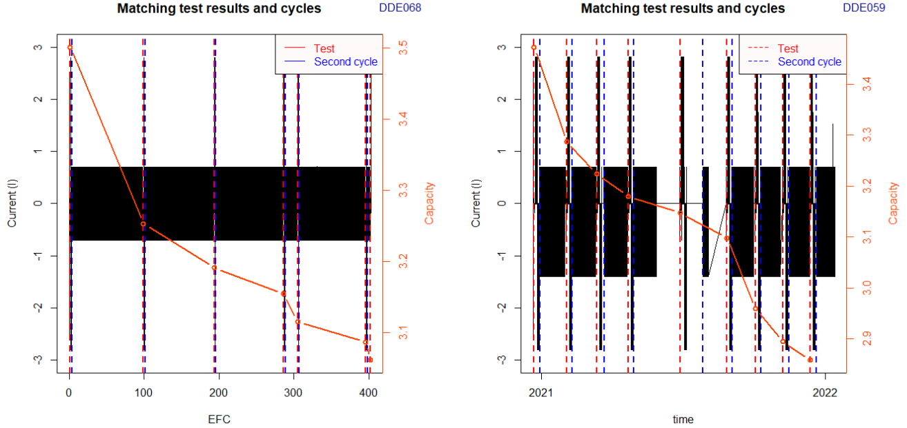
Figure 4. The extracted charge and discharge cycles in the raw time series have been matched with results from capacity measurements. In terms of EFC (left) and in terms of time (right)
