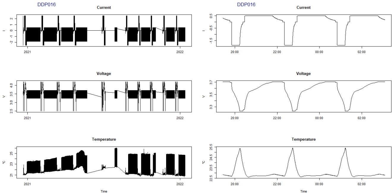
Figure 2. Example of measured time series from the cell cycling; currents (top), voltages (middle) and temperature (bottom); full time series (left) and zooming in on one of the periods with regular cycling (right)
