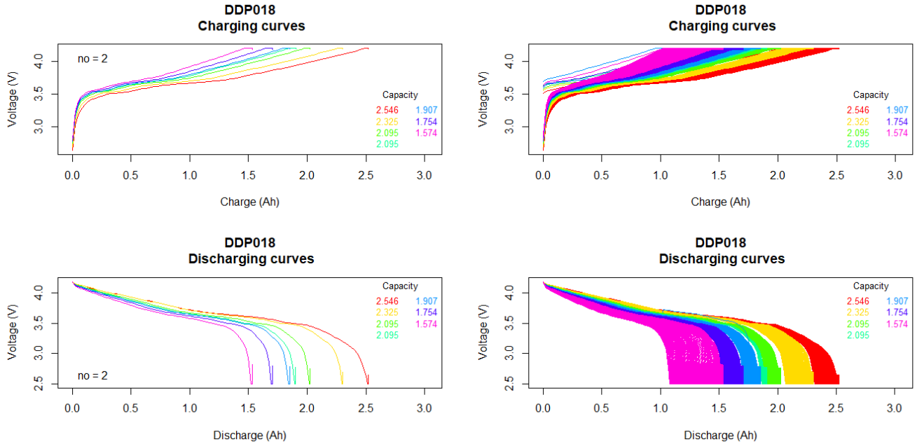
Figure 3. Extracted charge and discharge curves from the raw time series for an arbitrary cell. Only the second curves after each test (left) and all curves (right)
