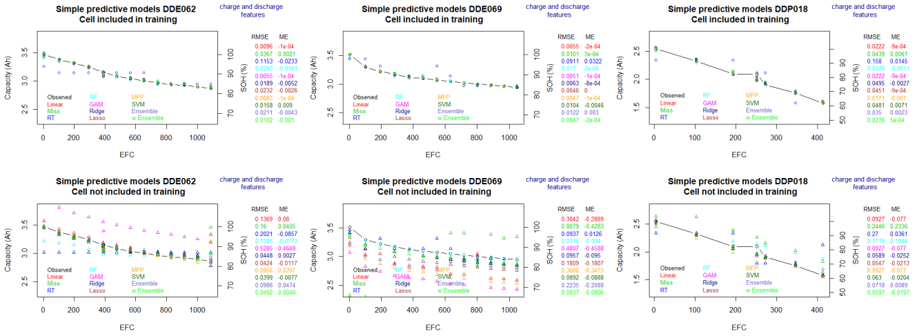
Figure 7. Data-driven predictions based on snapshot features with reasonable accuracy for some models and poor for others
