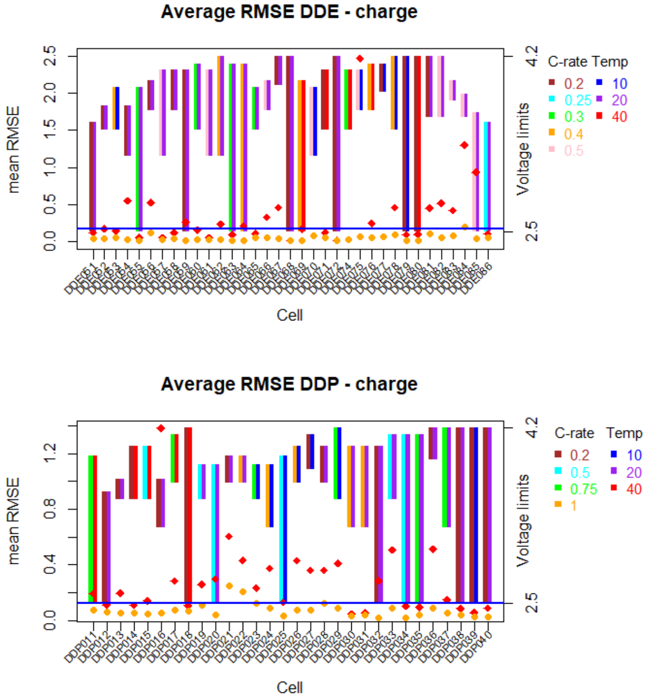
Figure 9. Average RMSE and test parameters for each cell
