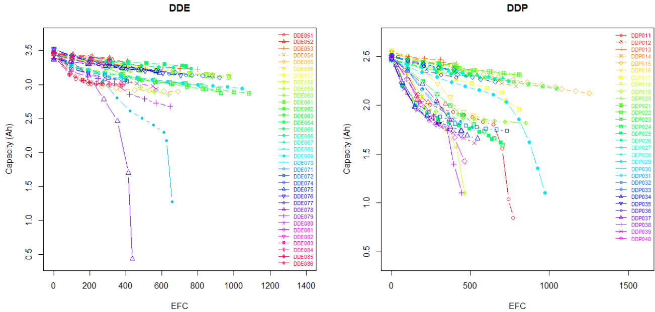
Figure 1. Measured capacity as a function of equivalent full cycles; DDE and DDP cells
