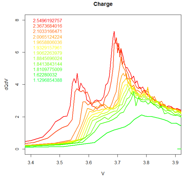
Figure 10. Example of derivative curves, dQdV
