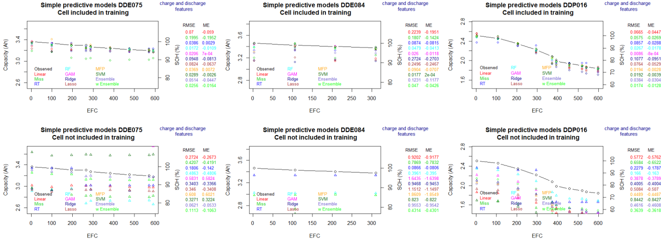
Figure 8. Data-driven predictions based on snapshot features with poor accuracy for most models
