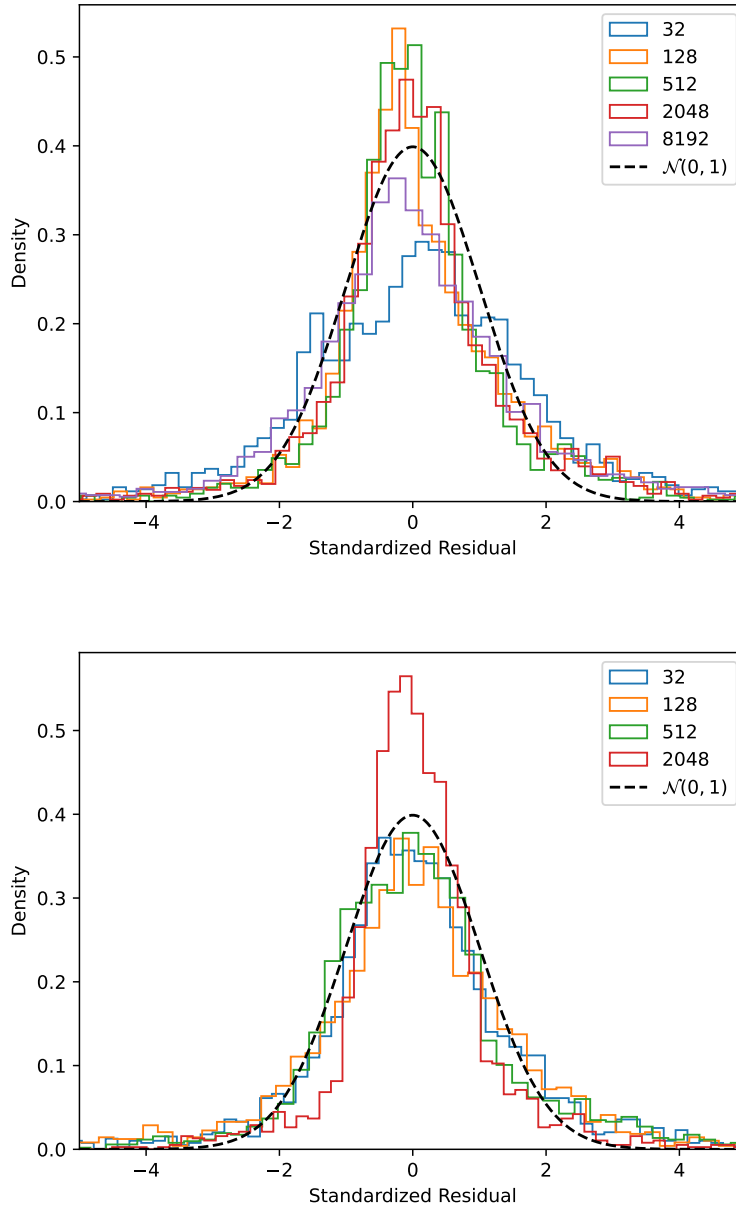
Figure 8.12: The figure shows the standardized residuals of models with an architecture 5-n-1 with \tanh(x) as the hidden layer activation. The models were trained with 1000 warm-up steps (20% burn-in and 80% adaptation), drawing 1000 neural networks with 10 steps between each drawn sample. We used 2500 pretraining epochs with a batch size of 32 using the ADAM optimizer. The figure on top shows results of models trained with the HMC sampler where we fixed the number of Leapfrog steps to L = 512 . The figure on the bottom shows the results of models trained with NUTS using a maximum of L = 4096 Leapfrog steps. The colors indicate the number of hidden layers nodes n are used. The black dotted line shows the standard Normal distribution drawn in.
