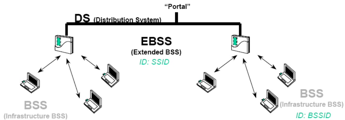
Figure 2.5: Illustration of a distribution system with one Extended BSS and two connected BSS
