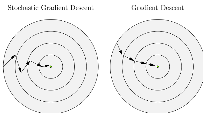
Figure 2.4: Comparison between SGD and gradient descent. The green dot in the middle represents the optimum.
