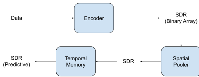
Figure 2.18: A typical HTM pipeline. A common next-step could be to use a classifier to convert the predictive SDR into a classification.
