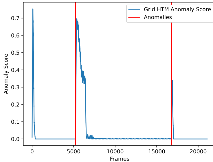
Figure 4.6: Results when using Grid HTM
