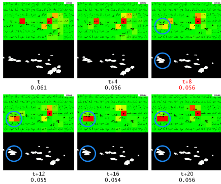
Figure 12: Anomaly output during the repeating frame, the start of the frame repeat is marked with red text. The blue circle highlights the object of interest.
