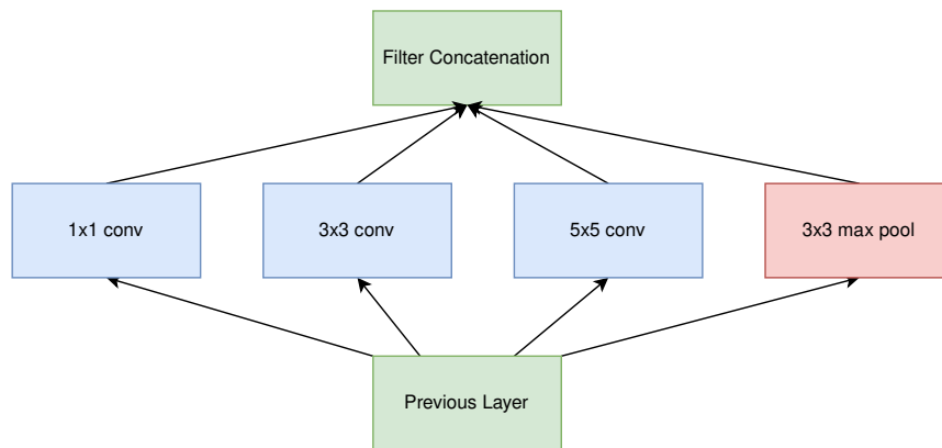
Figure 2.26: How the Inception [89] architecture uses multiple filters at once.
