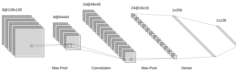
Figure 2.5: A typical CNN architecture used for classification.
