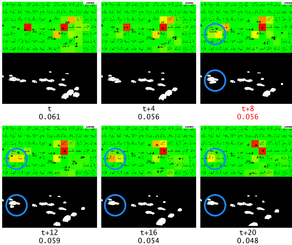
Figure 4.13: Anomaly output when there is no frame repeating, where it should have repeated is marked in red. The blue circle highlights the object of interest.
