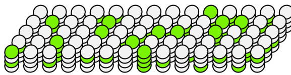
Figure 2.22: Visualization of the TM, with number of cells equal 4. Some columns are bursting.
