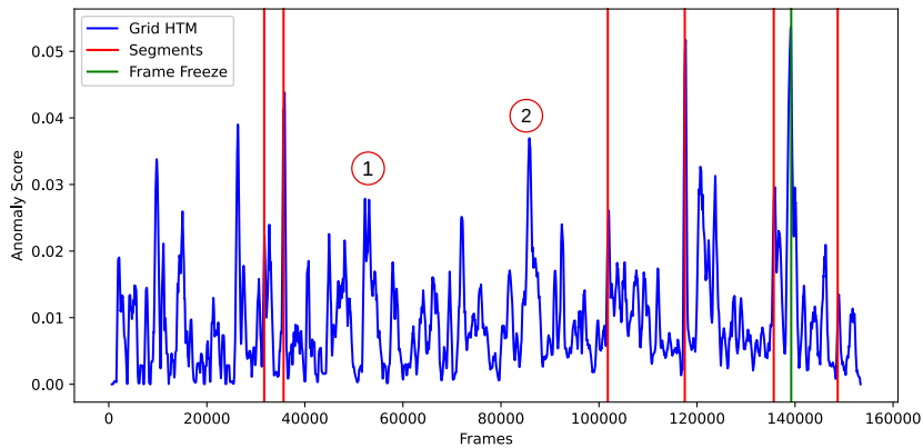
Figure 4.15: Points of interests in the anomaly score output.
