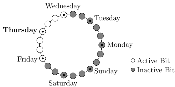
Figure 2.15: Visualization of a cyclical date encoding, which is currently encoding Thursday. Note that also Wednesday and Friday are included in the encoding of Thursday in order to emphasize that Wednesday and Friday are both equally distanced from Thursday.
