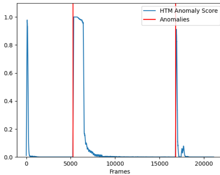
Figure 4.3: Bouncing ball with boosting enabled.
