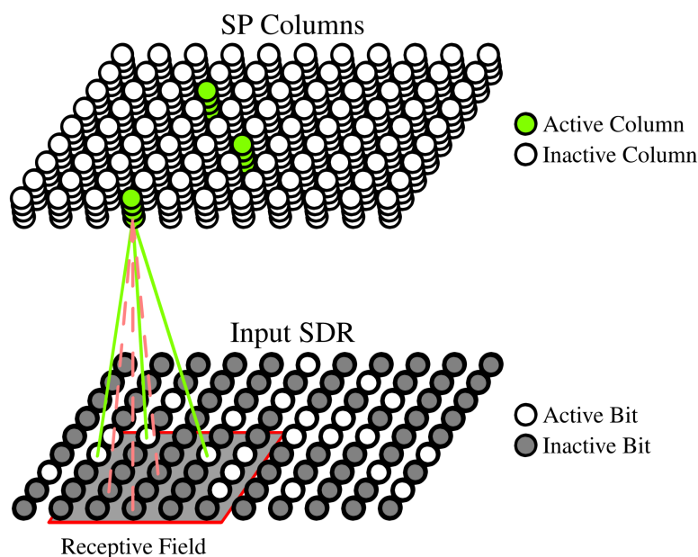
Figure 2.20: Visualization of the SP and the potential pool of one of its columns.
