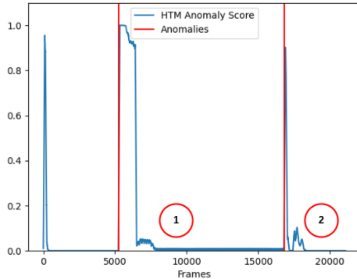
Figure 4.2: The anomaly score in the bouncing ball experiment.
