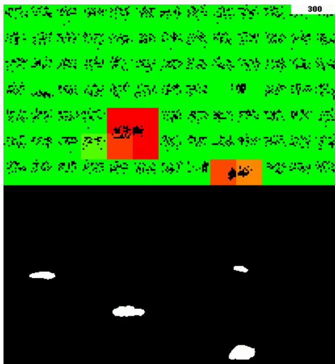
Figure 3.7: Example Grid HTM output and the corresponding input. The color represents the anomaly score for each of the cells, where red means high anomaly score and green means zero anomaly score. Two of the cars are marked as anomalous because they are moving, which is something Grid HTM has not seen before during its 300 frame long lifetime.
