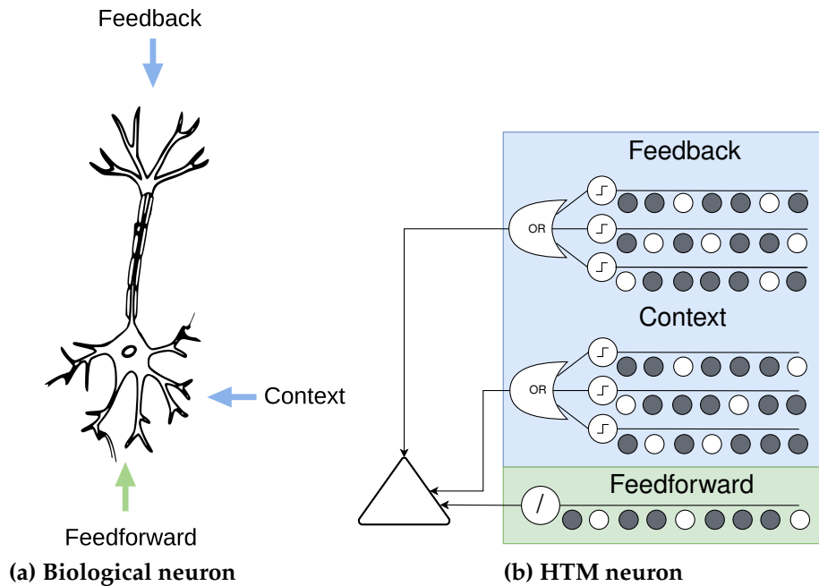
Figure 2.19: Biological neuron and HTM neuron, the colors show which part the Spatial Pooler (SP) and the Temporal Memory (TM) covers.
