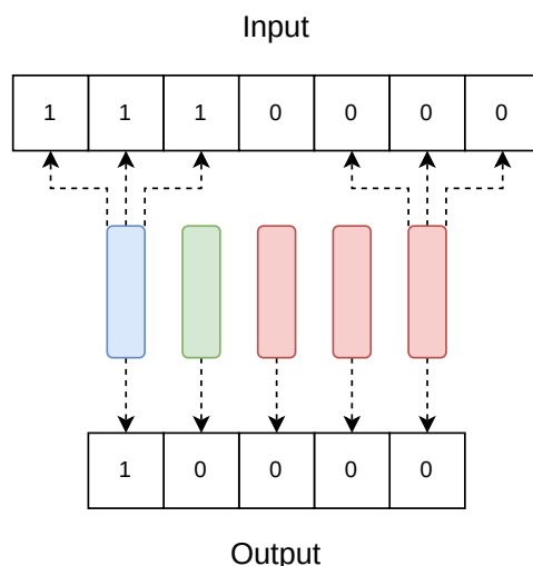
Figure 2.21: This figure illustrates how a spatial pooler works. All connections are above the stimulus threshold. The receptive field is 3 bits wide for each column. Overlap score threshold is 1, and n = 1 . Red means inactive, green means active, and blue means active and selected.
