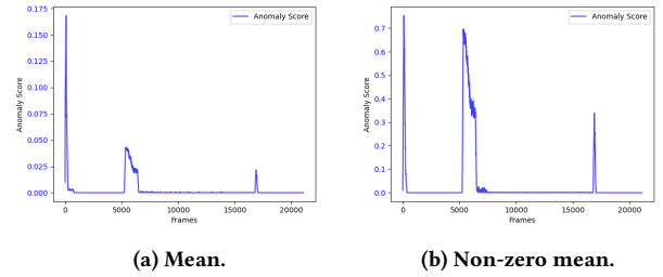
Figure 4: Aggregation functions performance on clean data.
