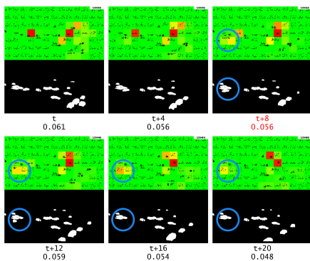
Figure 13: Anomaly output when there is no frame repeating, where it should have repeated is marked in red. The blue circle highlights the object of interest.
