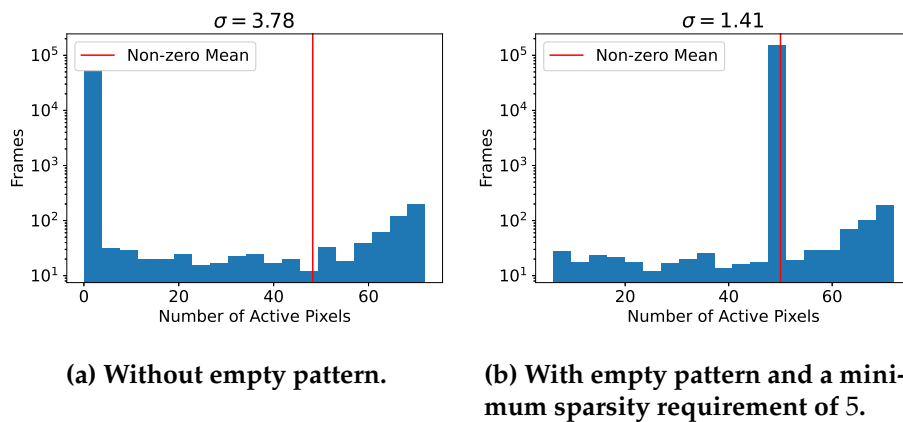
Figure 3.6: Distribution of number of active pixels within a cell of size 12 \times 12 .
