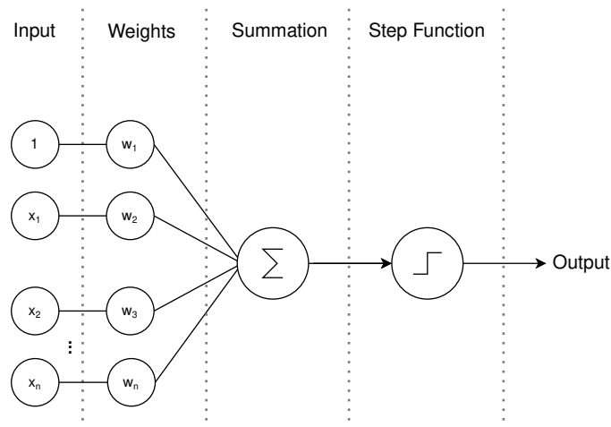
Figure 2.1: The original perceptron.
