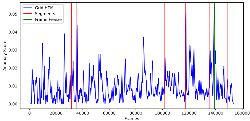
Figure 4.9: Anomaly score output from Grid HTM.
