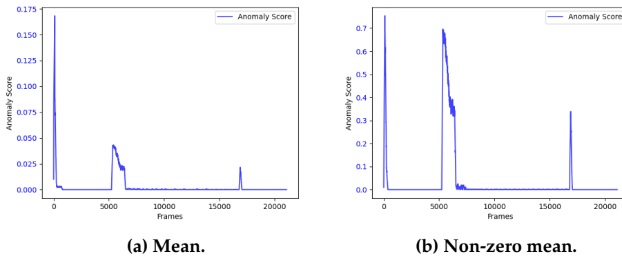
Figure 3.5: How the two aggregation functions perform on the same clean data. The graphs show their respective anomaly score output.
