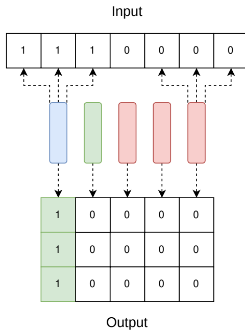
Figure 2.23: Expanded SP example with TM component where the number of cells is set to 3. The leftmost column is bursting (all 3 cells activated in green) due to the active SP output and due to containing no predictive cells.
