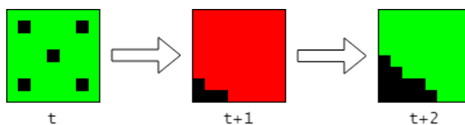
Figure 3.8: High anomaly score when an empty cell (represented with an empty pattern with a sparsity value of 5) changes to being not empty, as something enters the cell.
