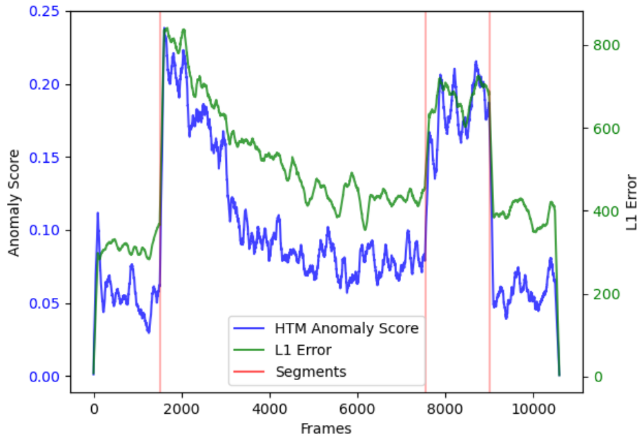
Figure 4.19: Results on a stationary sperm video.
