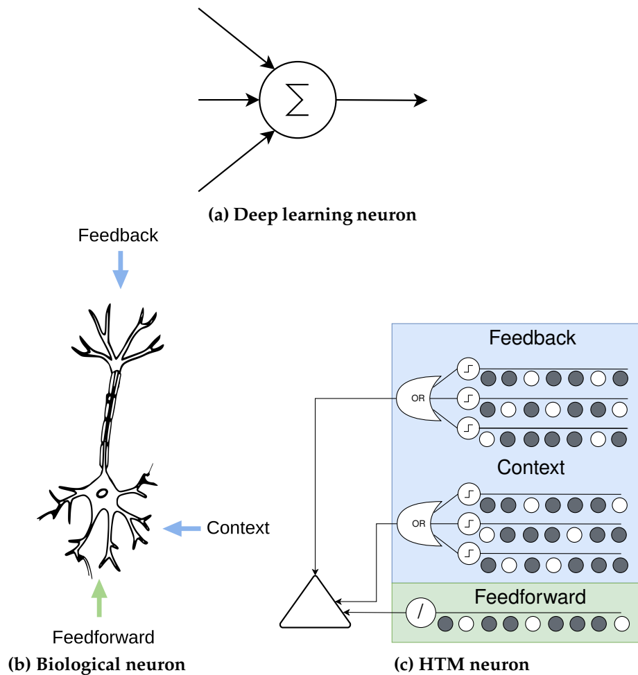
Figure 2.11: Comparison of neurons: Traditional Machine Learning (A), Biological Neuron (B), HTM Neuron (C).
