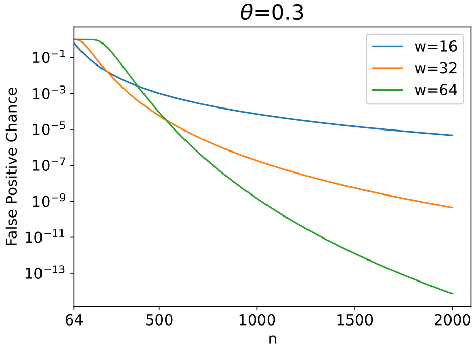
Figure 2.14: False positive chance of two SDRs with identical properties, with a 30% overlap threshold.
