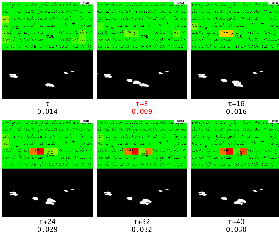
Figure 4.10: The first segment anomaly, which is marked with red text, and the corresponding changes detected by Grid HTM.
