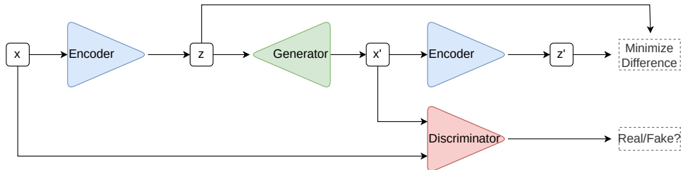
Figure 2.9: GANomaly [60], a variation of GAN for Anomaly detection.
