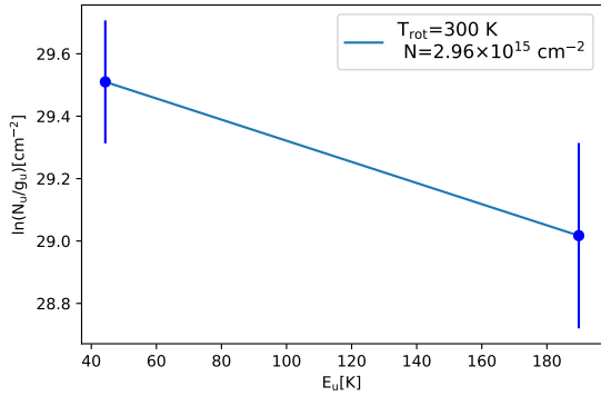
Fig. 6. Population diagram of observed AIF rotational lines towards R Leo. The data point with E_u = 44 K is the mean of the first three observations that are listed in Table 2 (see Sect. 3.2 for explanations).
