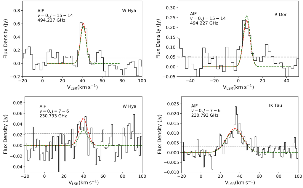
Fig. C.1. ALMA observations of AIF lines towards IK Tau, R Dor, and W Hya (Black solid lines) overlaid with LTE model results using T_{\text{rot}} = 145 K (red dashed lines) and T_{\text{rot}} = 300 K (green dashed lines) that are detailed in Sect. 3.3. The line rest frequencies and transition are stated in each panel. The AIF ( v=0, J=7-6 ) line emission at 230.7938 GHz can potentially be blended with ^{50}\text{TiO}_2 line at 230.7931 GHz. The grey dashed lines show the rms level.
