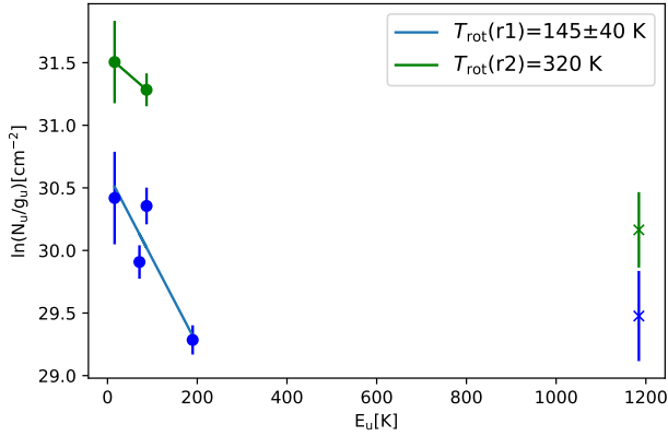
Fig. 2. Population diagram of observed AIF rotational transitions towards o Ceti that are listed in Table 2. Blue points correspond to flux densities that are extracted from region 1 and green points correspond to those from region 2 (see Sect. 3.1 for explanations). The vibrationally excited v = 1 lines in both regions are also shown by x symbols, but they were not considered in the calculations of the rotational temperatures. The vertical error bars are calculated from the uncertainties of the integrated fluxes (uncertainty from the Gaussian fitting plus 10% of the total flux from the calibration of the data) and are considered in the fitting process.
