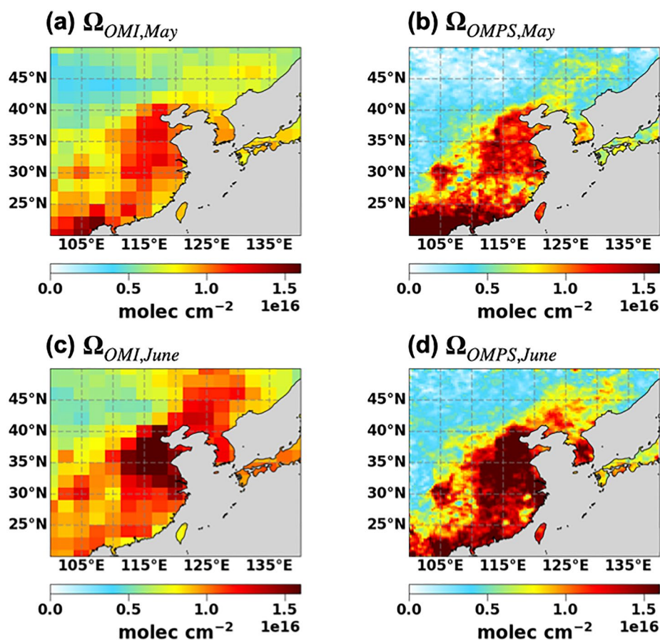
Figure 2. The (a, c) OMI and (b, d) OMPS CH 2 O VCDs. The OMI CH 2 O VCDs are oversampled at 2^\circ \times 2.5^\circ resolution for (a) May 2014–2016 and (c) June 2014–2016. The OMPS CH 2 O VCDs are oversampled at 0.25^\circ \times 0.3125^\circ resolution for (b) May 2016 and (d) June 2016. The units are molec cm -2 . Ocean data is not used for the inversion because of higher noise, lower concentrations, and small influence from continental VOC emissions.
