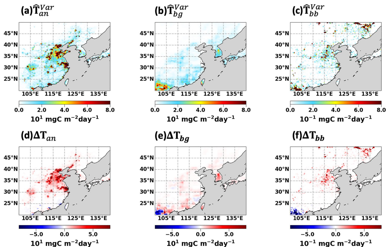
Figure 10. Top: the hybrid a posteriori total VOC emissions at 0.25^\circ \times 0.3125^\circ resolution during the KORUS-AQ campaign period from (a) anthropogenic ( \hat{T}_{an} ), (b) biogenic ( \hat{T}_{bg} ), and (c) biomass burning ( \hat{T}_{bb} ) sectors. Bottom: the emission changes from the a priori total VOC emissions for (d) anthropogenic ( \Delta T_{an} ), (e) biogenic ( \Delta T_{bg} ), and (f) biomass burning ( \Delta T_{bb} ) sectors. Units are \text{Gg C day}^{-1} .
