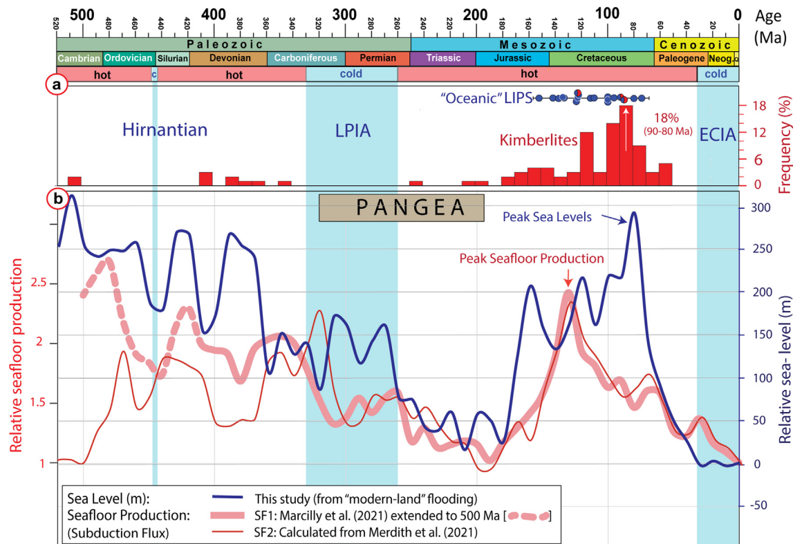
Fig. 8. (a) Time-scale, greenhouse (hot) vs. icehouse (cold) (See Fig. 1 caption for additional details), kimberlite frequencies for the past 520 Myrs (10 Myr bins), and preserved “oceanic” large igneous provinces (LIPs). The blue dots represent oceanic LIPs and shared blue/red dots represent continental and oceanic LIPs. (b) “Modern-land” sea level calculated from flooding maps (this study) compared to two proxies for relative seafloor production calculated from the subduction flux of full-plate models: SF1 from Marcilly et al. (2021) extended from 410 to 500 Ma.; SF2 calculated from the full-plate model of Merdith et al. (2021). (For interpretation of the references to color in this figure legend, the reader is referred to the web version of this article.)
