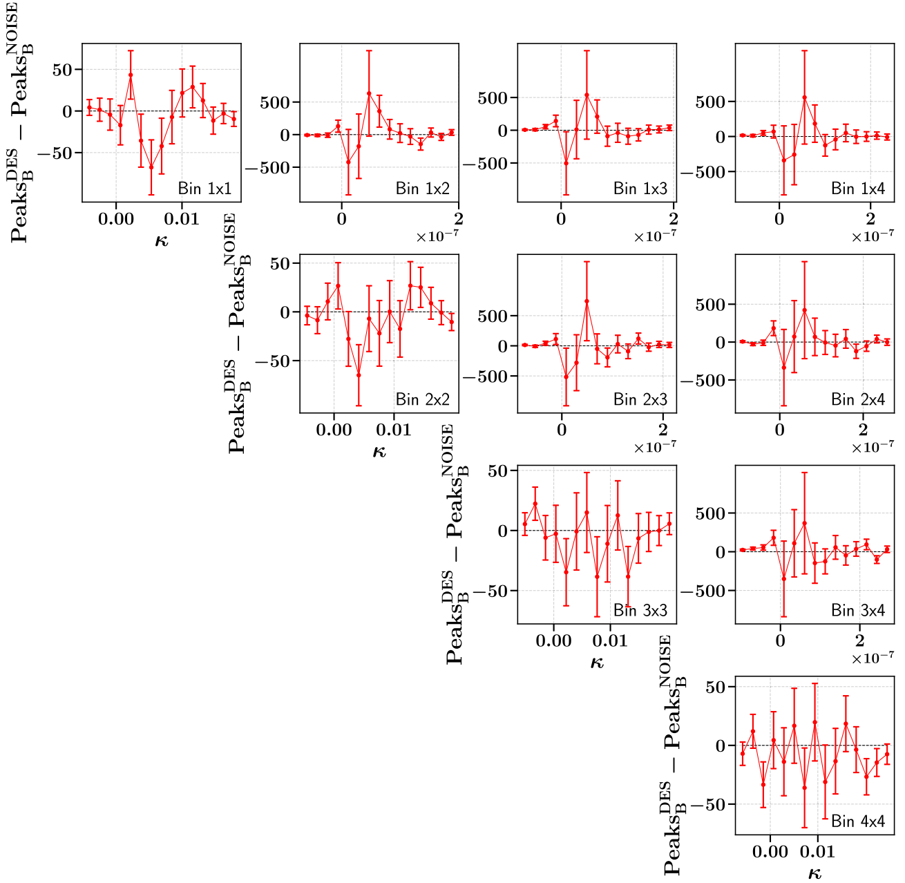
Figure G2. The noise-subtracted DES Y3 peak count B-modes for a selected smoothing scale of \text{FWHM} = 21.1 arcmin. The noise signal was inferred using simulations with only a shape noise component but no cosmological signal. Using the smoothing scales \text{FWHM} \in [7.9, 31.6] arcmin we find \chi^2/\text{dof} = 1.14 and p = 31 per cent.
