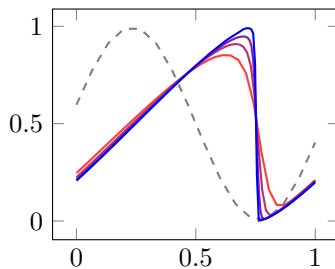
Figure 8: Experiment 5. Second-order numerical approximations for the nonlocal model with \delta = 3\Delta x with \Delta x = 1/32 , \Delta x = 1/64 , and \Delta x = 1/128 (increasingly darker red, p = 0 ) and for the local conservation law with \Delta x = 1/128 (blue) and \lambda = 0.8 , T = 0.5 , and u(x, 0) = u_0^1(x) .
