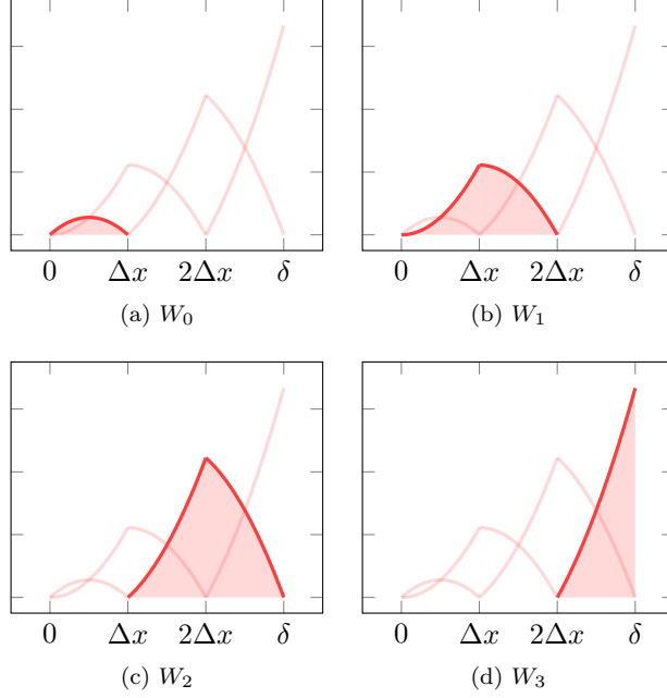
Figure 1: Weights for \delta = 3\Delta x and \omega_\delta(h) = \frac{2}{\delta^2}h . The weights correspond to the highlighted areas.
