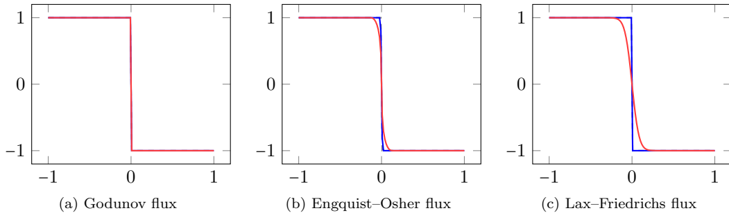
Figure 6: Experiment 4. Second-order numerical approximations for the local conservation law and the nonlocal model (in blue and red respectively) with \Delta x = 2/128 , \lambda = 0.8 , \delta = 0.125 , p = 0 , T = 1 , and u(x, 0) = u_0^4(x) .
