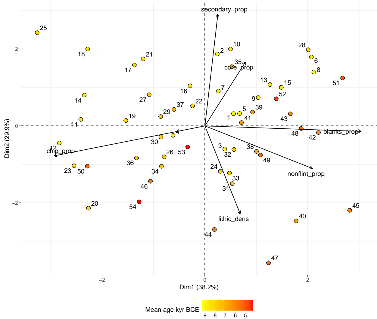
Figure 6: PCA biplot resulting from analysing variables that have been related to mobility patterns. Note that details on the transformation of the variables has been left out of the plot for clarity, but follow those given in Figure 5.
