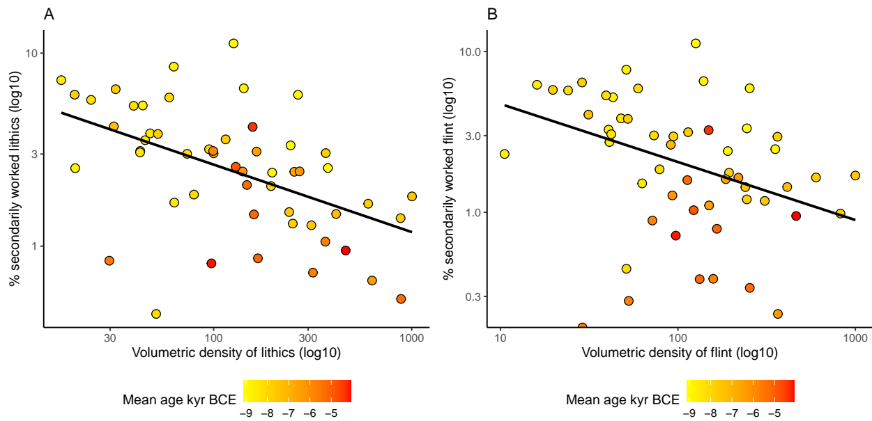
Figure 8: Relative frequency of secondarily worked lithics plotted against the volumetric density of artefacts for A) All lithics ( r = -0.5 ), B) Flint ( r = -0.4 ). The logarithm is taken to base 10 on all axes.
