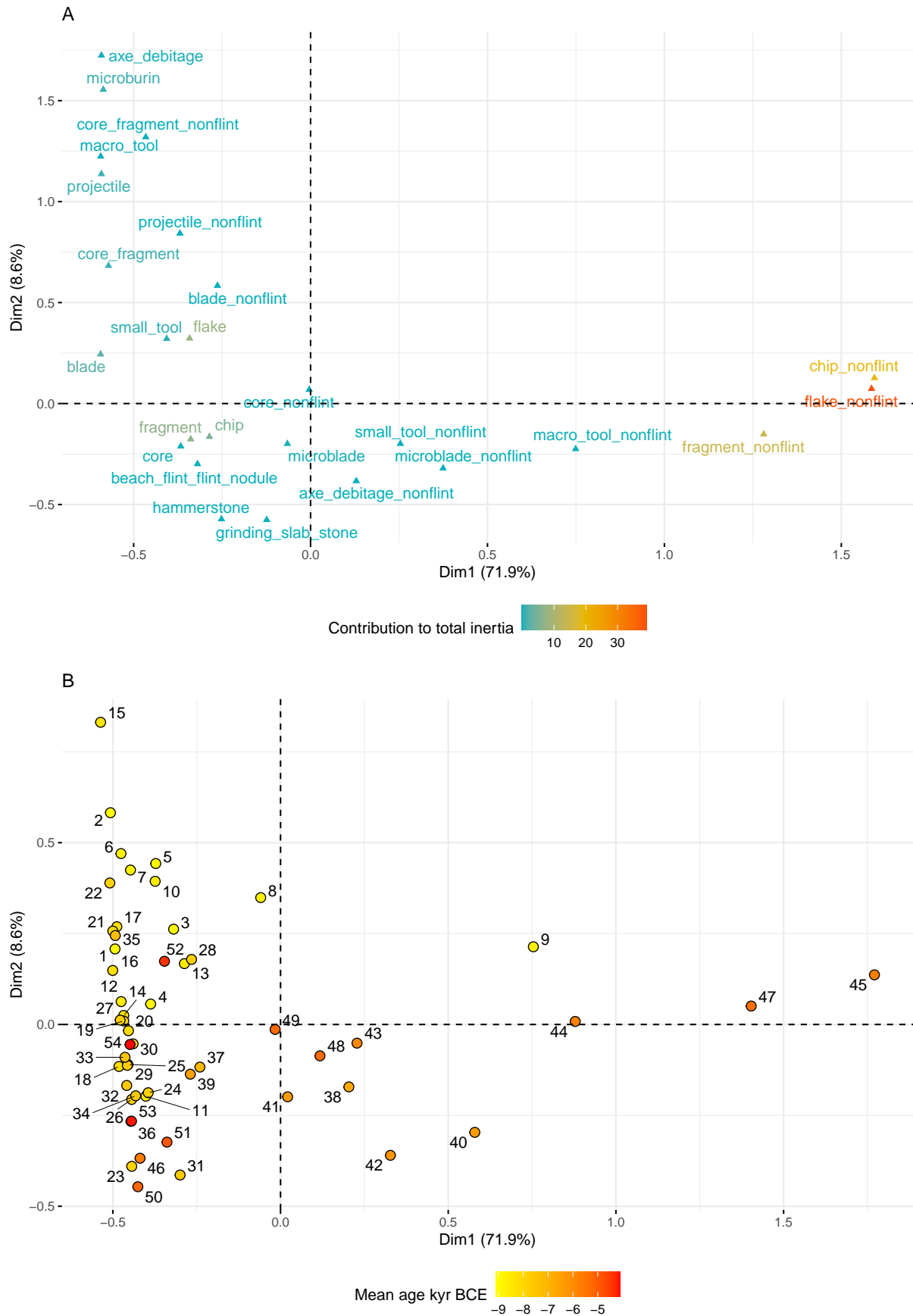
Figure 3: Correspondence analysis using the artefact count data. A) Column plot (variables), B) Row plot (sites). Points close together are more similar. By evaluating how the variables are distributed on the column plot it is possible to say how these define the two axes, in turn making it possible to relate the distribution of the sites in the row plot to the variables. As these are symmetrical plots, only general statements concerning the interrelation between the rows and the columns across the two plots can be made.
