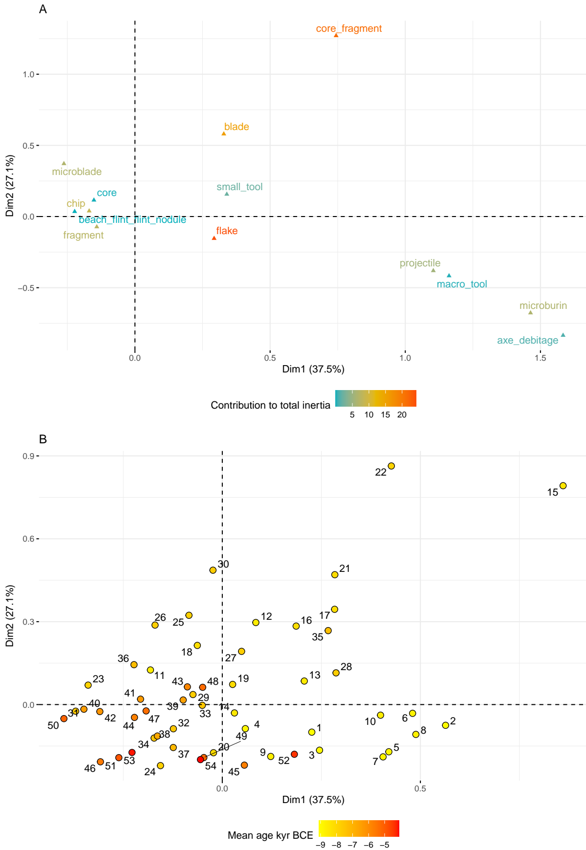
Figure 4: Correspondence analysis using the flint data. A) Column plot, B) Row plot.
