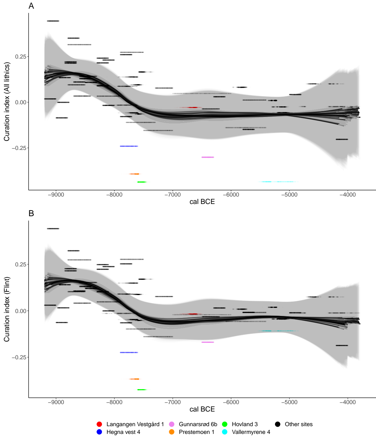
Figure 9: Temporal variation in the curation index for A) All lithics, and B) Flint. The temporal uncertainty is handled by means of a simulation approach where the site ages are drawn from their respective age determination probability density functions given in Figure 1B. A LOESS curve has been fit to the distribution for each of the 1000 simulation runs. Each simulation run is plotted with some transparency. Sites mentioned in the text are given colour.
