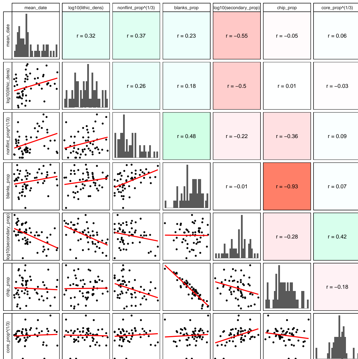
Figure 5: Correlation matrix showing transformation of skewed variables for the PCA. The mean age of the sites has also been included to visualise overall temporal trends. Cells below the diagonal display the bivariate distributions with a fitted OLS-regression. The cells above the diagonal display and are coloured by the corresponding Pearson's correlation coefficient.
