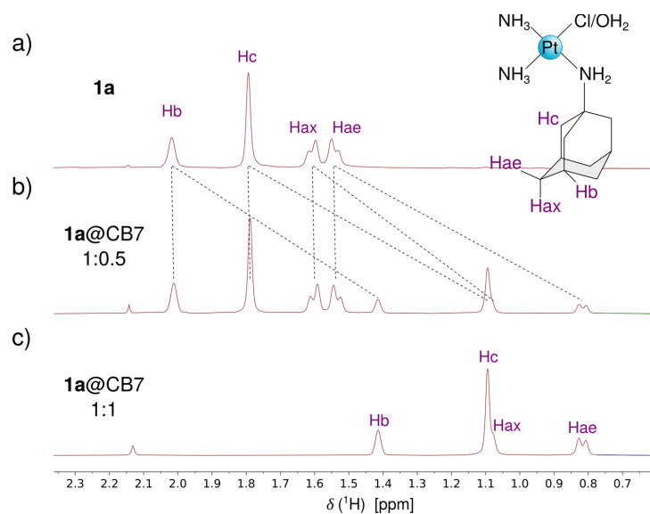
Figure 7. Adamantyl region of the 1 H NMR spectra of (a) 1a , (b) 1a with 0.5 equiv of CB7, and (c) 1a with one equivalent of CB7 in D 2 O at 298 K. Note that the NMR signals of encapsulated/bound Ad in panels (b) and (c) correspond to the hydrolyzed form of compound 1a ( vide infra ).
