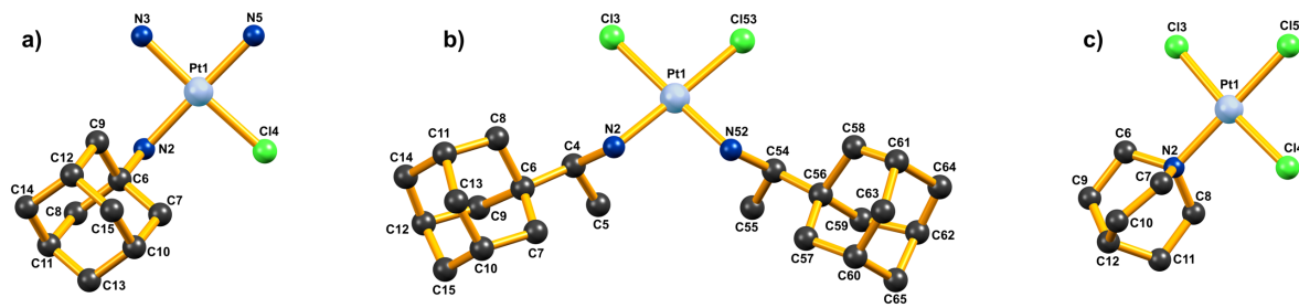
Figure 4. Molecular structure of (a) complex cation of 1a , (b) compound 5b , and (c) complex anion of 7d determined by X-ray diffraction analysis. Counter ions and solvent molecules are omitted for clarity.
