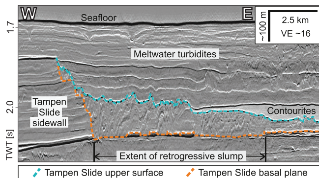
Figure 8. Seismic profile crossing a small volume ( \sim 12 \text{ km}^3 ) retrogressive slump on the western sidewall of the Tampen Slide. Note the blocky character of the slump deposits. Location of this figure is shown in Figure 3. VE: Vertical Exaggeration. Data from AMS17 Vol. B, and courtesy of TGS.
