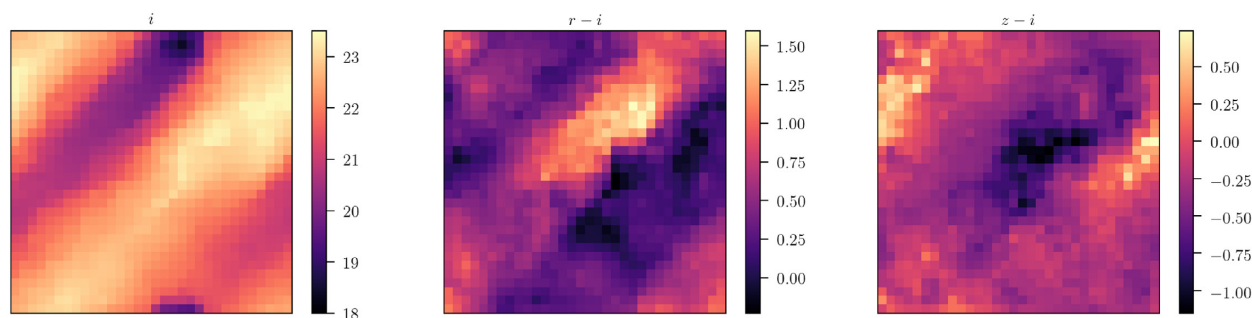
Figure A1. Visualization of the wide self-organizing map. Shown here are the mean i -band magnitude (left-hand panel), the mean r - i colour (middle panel), and the mean z - i colour (right-hand panel) of each cell in the wide SOM. The implementation of SOMs used in our analysis generates a toroidal map; in other words, the left and right edges of each map correspond to the same region of colour–magnitude space, as do the upper and lower edges.
