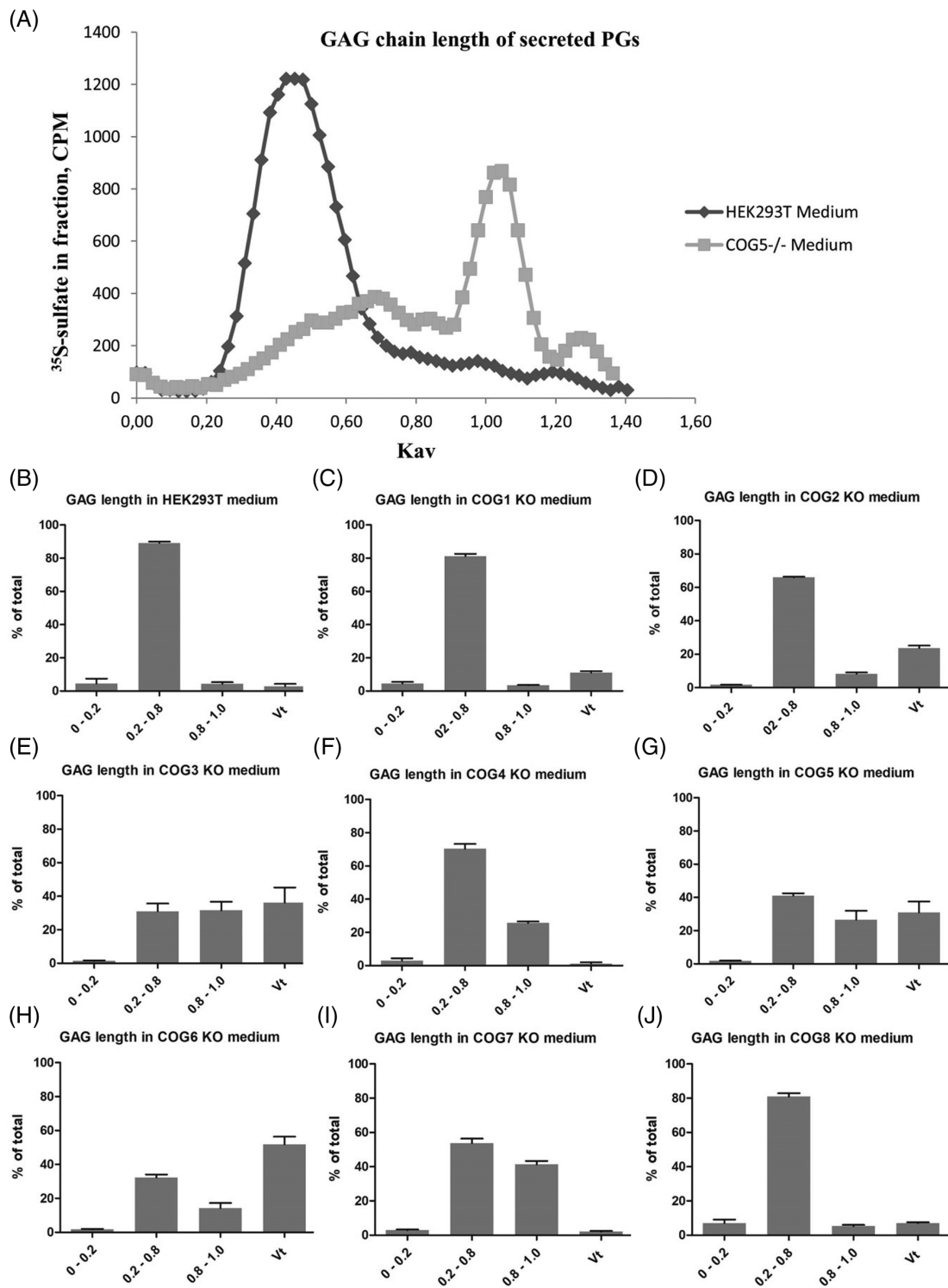
FIGURE 4 Gel filtration analysis of GAG chain length of secreted PGs. Medium samples eluted from Sephadex G50-fine columns were subjected to alkaline treatment (see Section 2) to detach GAG chains from their protein cores. The samples were added the V_o and V_t markers Blue Dextran and \text{K}_2\text{CrO}_4 , respectively, for V_o and K_{av} calculations, and then applied to Sepharose CL-6B columns to compare the chain lengths of GAGs synthesized by HEK293T cells and COG subunit deficient cell lines. Panel A shows two examples (HEK293T control and COG5) runs. The panels show the size distribution of GAG chains in at least three samples for each cell line. The fractionation range of Sepharose CL-6B being 10 000 to 1 000 000 (for dextrans). 0 to 0.2 are the longer chains, 0.2 to 0.8 are intermediate chains, while 0.8 to 1.0 are shorter chains. In the V_t , are very short chains with full access to all of the column material, of less than (approximately) 20 disaccharides
