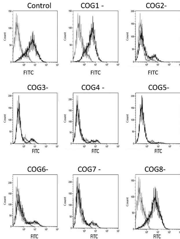
FIGURE 6 Flow cytometry with cell surface bound anti HS-antibody. HEK293T cells and COG subunit deficient cell lines were suspended in PBS and incubated with the 10E4 anti-HS antibody for 30 min at 4°C before staining with goat anti-mouse IgM FITC. Controls are incubated with goat anti-mouse FITC, only. Cells were analyzed with a FACSsort flow cytometer. Flow data collection was carried out with the program CellQuest 3.3 and the data generated using Kaluza Flow Cytometry analysis v 1.2. A total of 20 000 or more cells gated as viable were analyzed per sample. The figure shows data for wild type HEK293T cells (control) and the cell lines deficient in individual COG subunits 1 to 8
