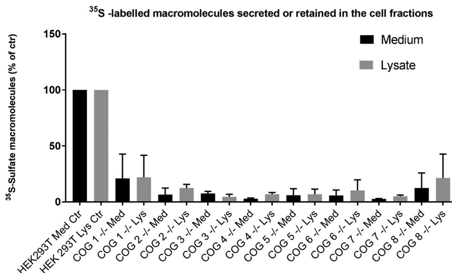
FIGURE 1 Synthesis and secretion of sulfate labeled macromolecules in wild type and COG subunit KO HEK293T cells. HEK293T wild type and cell lines depleted of individual COG subunits were incubated for 24 h in the presence of 0.2 mCi/ml ^{35}\text{S} -sulfate in sulfate-depleted medium. The media and cell fractions were processed as described in Section 2 methods, and the content of sulfated macromolecules was quantified by scintillation counting and is expressed as % of that of wild type HEK293T cells. The figure is based on four experiments with three parallels in each
