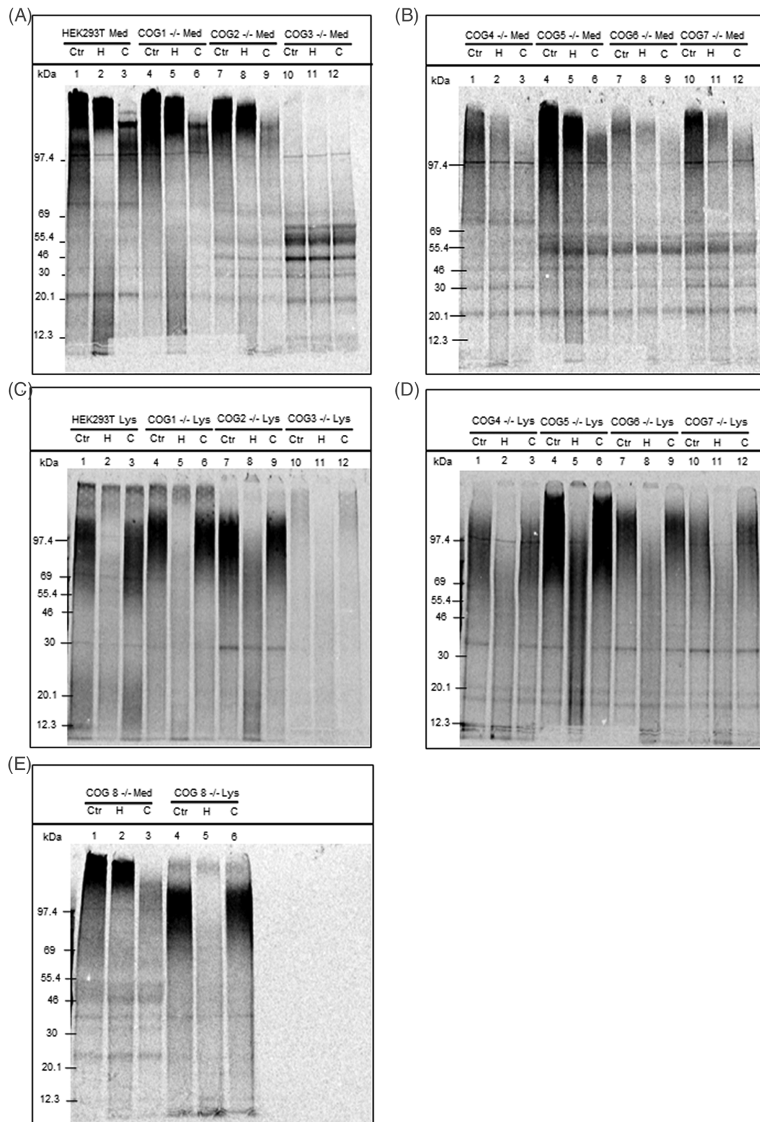
FIGURE 3 SDS-PAGE analysis of synthesis and secretion of sulfated macromolecules in wild type and COG subunit KO HEK293T cells. The eluates from Sephadex G-50 fine gel filtration chromatography columns were concentrated by freeze drying to contain approximately 15 to 20 000 cpm each in SDS-PAGE sample buffer. Parallel aliquots of each sample were subjected to no treatment (Cnt) or to treatment with cABC to degrade CS/DS (C) or hep to degrade HS and heparin (H) prior to SDS-PAGE (4%-12% gradient gels). Medium samples in panels A and B and cell lysate samples in panels C and D. Samples from COG8 deficient cells (both medium and cell lysate) in panel E
