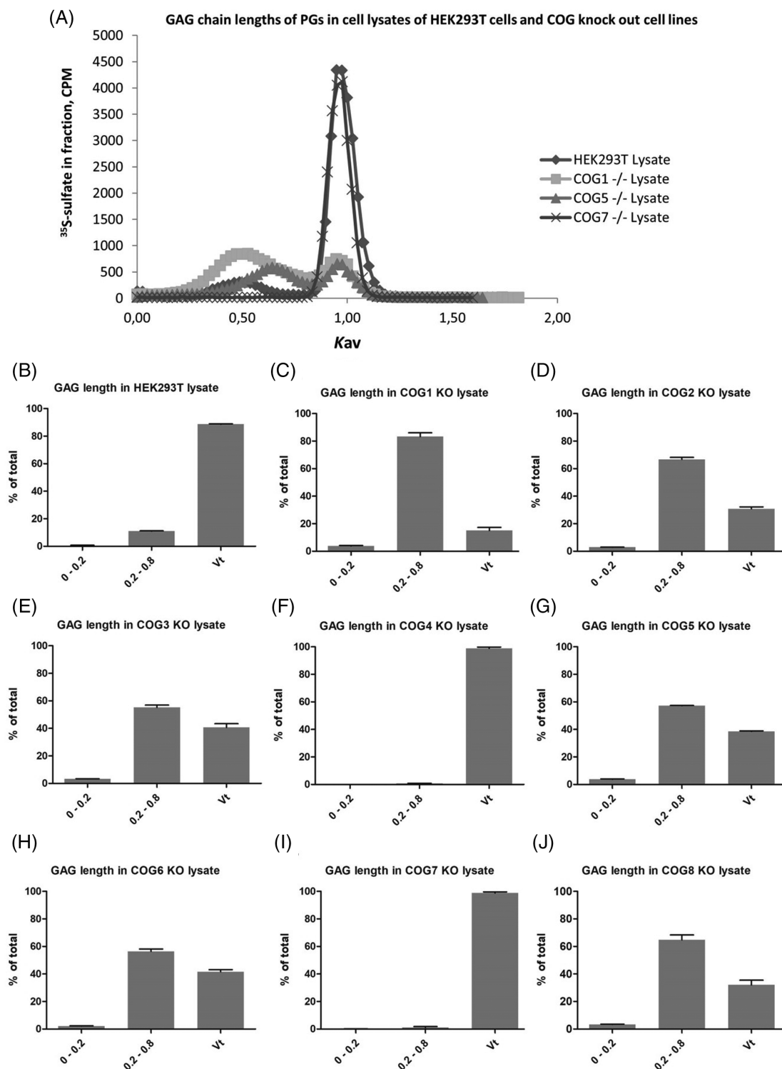
FIGURE 5 Gel filtration analysis of GAG chain length of cell-associated PGs. Cell lysate samples eluted from Sephadex G50-fine columns were subjected to alkaline treatment (see Section 2) to detach GAG chains from their protein cores. The samples were added the V_o and V_t markers Blue Dextran and K_2CrO_4 , respectively, for V_e and K_{av} calculations, and then applied to Sepharose CL-6B columns to compare the chain lengths of GAGs synthesized by HEK293T cells and COG subunit deficient cell lines. Panel A shows two examples (HEK293T control and COG5) runs. The panels show the size distribution of GAG chains in at least three samples for each cell line. The fractionation range of Sepharose CL-6B being 10 000 to 1 000 000 (for dextrans). 0 to 0.2 are the longer chains, 0.2 to 0.8 are intermediate chains. In the V_t , are very short chains with full access to all of the column material, of less than (approximately) 20 disaccharides
