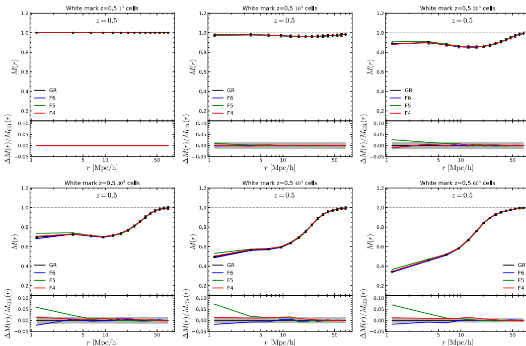
Figure 33. (Color Online) The marked correlation functions (mCF) with the White mark with (\rho_*, p) = (4, 10) , for different numbers of cells used to calculate the density field.
