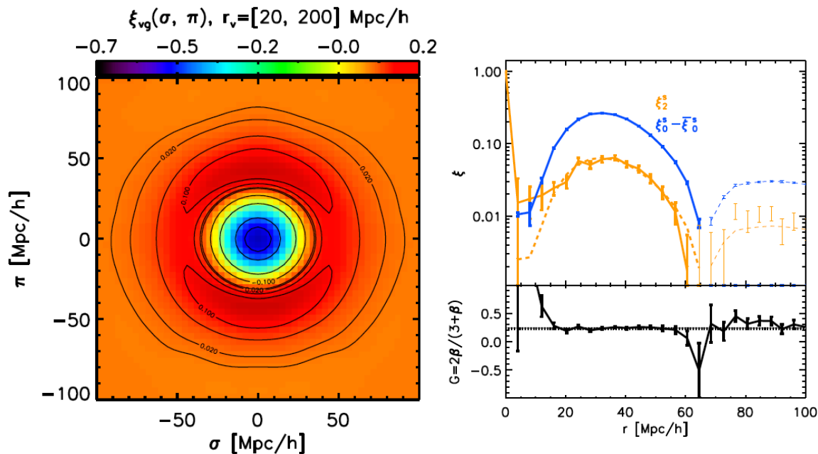
Figure 11. Left: the void-galaxy correlation function in redshift space for the GR model for voids identified by ZOBOV with the HOD galaxies in 5 boxes of the 1024h^{-1}\text{Mpc} -aside simulation. Voids with effective radius r_v > 20h^{-1}\text{Mpc} are used. Right: the upper panel shows the monopole (blue) and quadrupole (orange) moments of the redshift-space correlation function. Thin lines indicate the absolute values of negative parts. The lower panel shows the ratio of the quadrupole versus monopole. The black curve is from taking all measurements of voids along three different major axes of the simulation box, with the error bars showing the error on the mean. The dotted line is the true answer for the growth rate parameter G given by the cosmology and galaxy bias. The black shaded region shows the 1\sigma range around the best-fit value.
