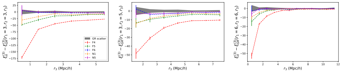
Figure 21. The 3-point correlation function difference between GR and several modified gravity scenarios. Left: a triangular configuration with r_1 = r_2 = 3 h^{-1}\text{Mpc} . Center: with r_1 = 3 h^{-1}\text{Mpc} and r_2 = 5 h^{-1}\text{Mpc} . Right: r_1 = r_2 = 6 h^{-1}\text{Mpc} . The shaded regions are the standard deviations of the five realizations of the HOD catalogs for GR. All results are for z = 0.5 .
