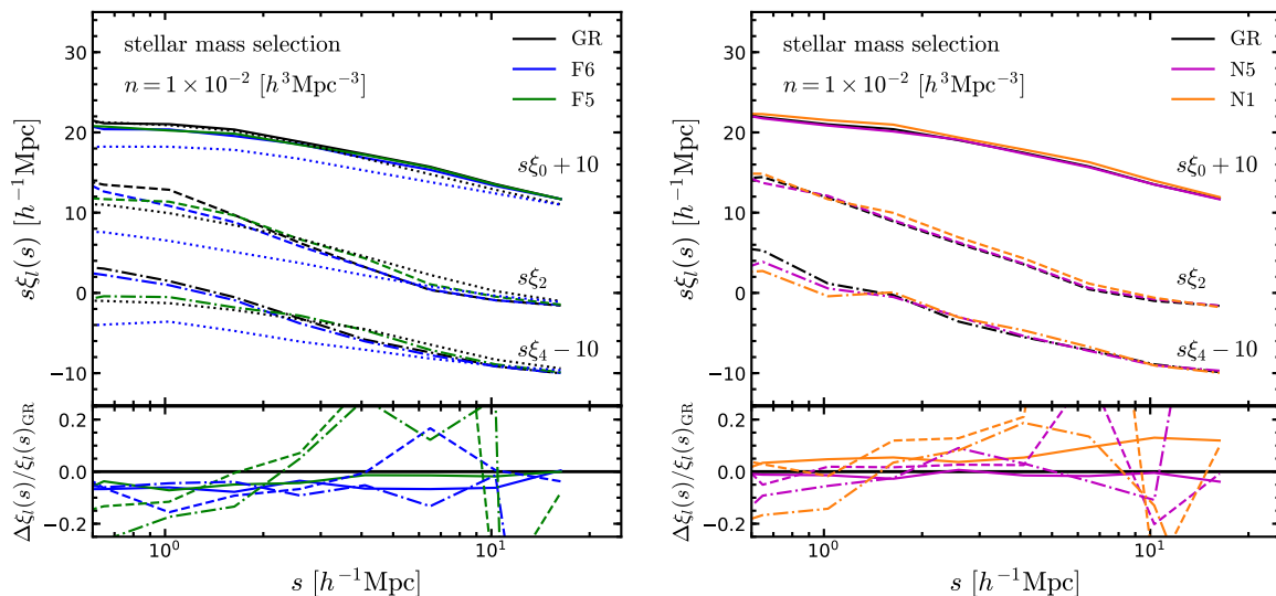
Figure 10. Small-scale redshift space galaxy clustering measured from the full-hydrodynamical SHYBONE simulations [36, 37] for the F6 and F5 models ( left panel ), and the N5 and N1 models ( right panel ). In the left panel we additionally show the measurements from the SHAM catalog (dotted lines) for comparison. The lower subpanels show the relative difference of the measurements from the MG full-physics simulations with respect to their GR counterpart.
