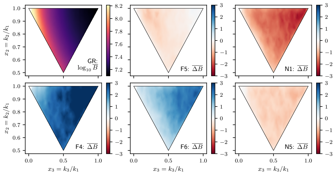
Figure 23. Configuration dependence of the real-space bispectrum, obtained by integrating the raw measurements over k_1 (see eq. (3.28)) between k_1 = 0.3 h/\text{Mpc} and 0.75 h/\text{Mpc} . Configurations outside of the triangular area are forbidden according to the closure condition and the top left, top right and bottom corners correspond to squeezed, equilateral and folded configurations, respectively.
