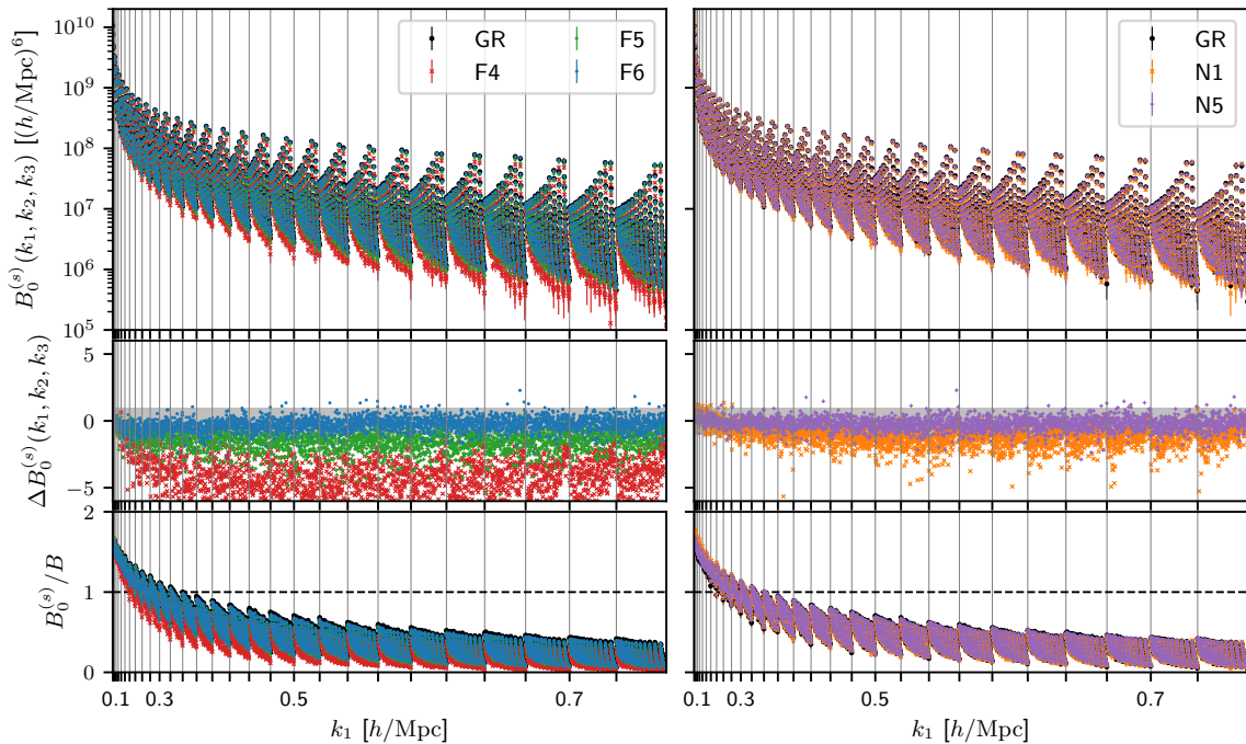
Figure 24. Measurements of the bispectrum monopole in redshift-space. The panels in the upper two rows are the same as those in figure 22, while the bottom panels show the ratio between the redshift-space monopole and the real-space bispectrum.
