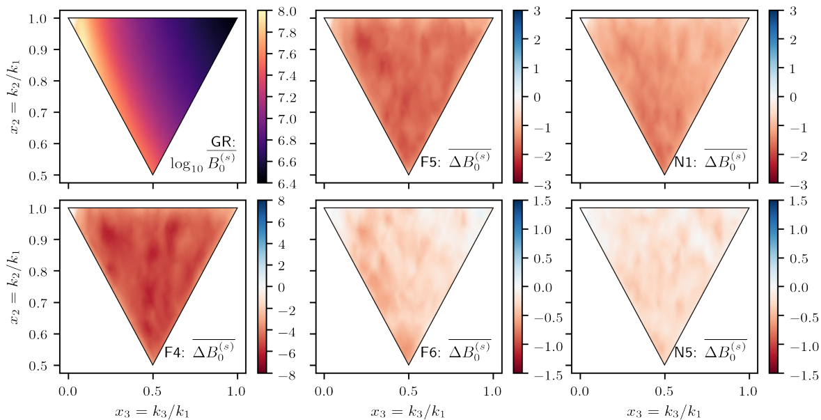
Figure 36. (Color Online) Configuration dependence of the monopole of the redshift space bispectrum.
