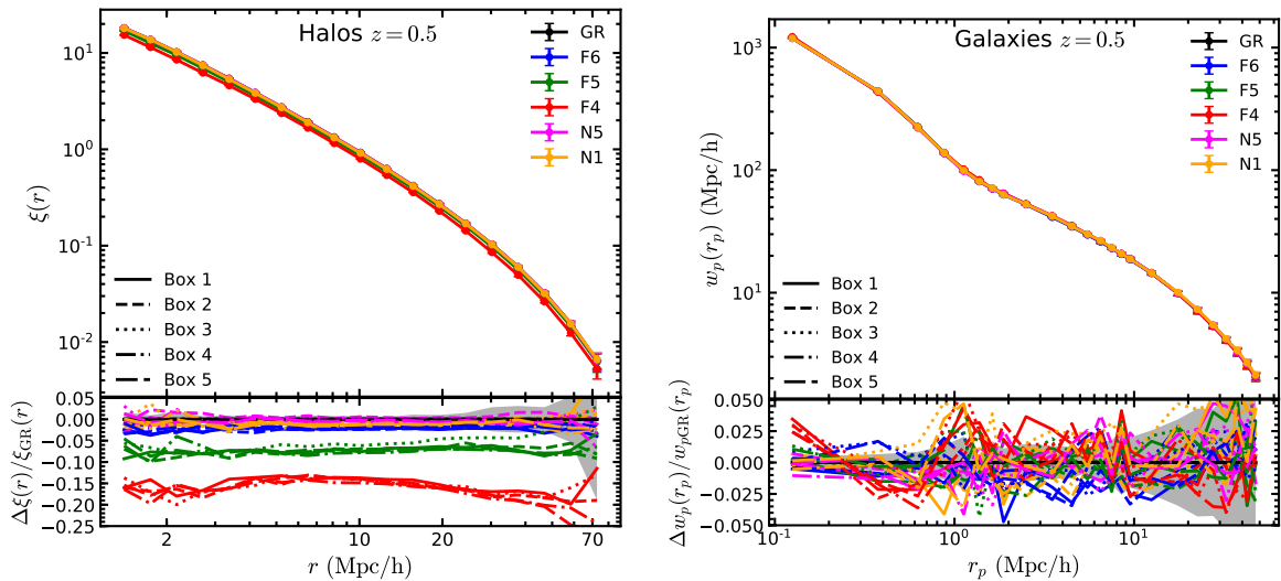
Figure 4. (Color Online) Left panels: the 3D halo two-point correlation functions, \xi_{hh}(r) , for the six models, averaged over all five realizations, as a function of halo separation r (upper panel) and the relative differences with respect to \Lambda CDM (lower panel; the five simulation realizations are shown individually using different line styles as in figure 1). Note that only halos more massive than 10^{13}h^{-1}M_{\odot} are used, so that the halo number densities are different in the different models. Right panels: the same as the left panels, but for the projected correlation functions of HOD galaxies, w_p(r_p) . All results are at z = 0.5 . The error bars in the top panels and the shaded regions in the bottom panels are the standard deviation of 5 \Lambda CDM realizations.
