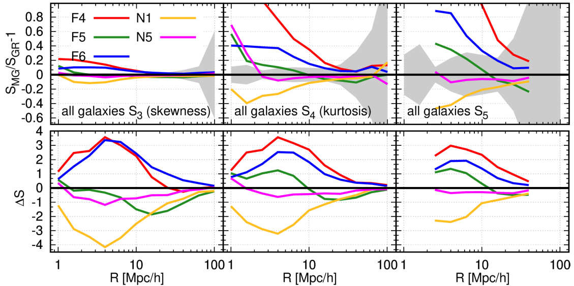
Figure 26. Top row: the relative differences of the skewness (left panel), kurtosis (central panel) and hyperskewness (right panel) taken with respect to the fiducial GR case. The shaded regions mark the error round the ratio of ensemble averages. Bottom row: the equivalent error-weighted differences, \Delta S , similarly defined as in eq. (3.27), for each statistics.
