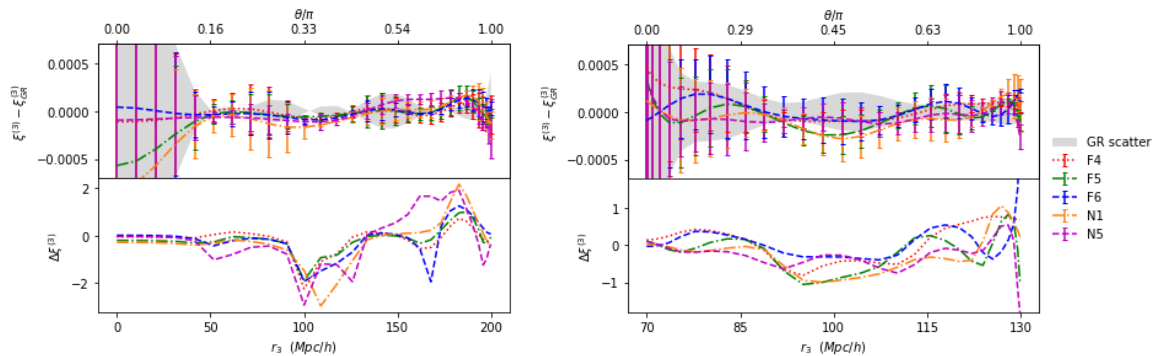
Figure 20. Full 3PCFs for r_1 = 100h^{-1}\text{Mpc} and r_2 = r_1 (Left) or r_2 = 30h^{-1}\text{Mpc} (Right). The top panels show differences of the MG 3PCF with respect to GR as a function of the third triangle side r_3 , or equivalently, the opening angle \theta_{12} between r_1 and r_2 . The bottom panels show the model differences using the analog of the variable \Delta\sigma\xi_\ell^{(3)} but for the full 3PCF. We use the first \ell < 10 multipole moments in figure 19 to construct the complete 3PCF.
