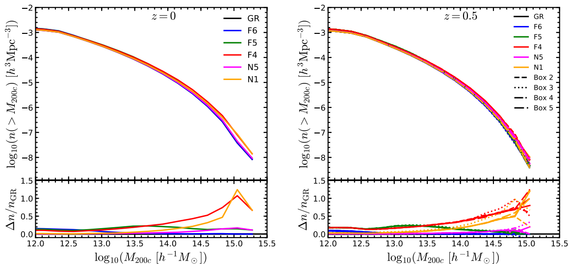
Figure 2. (Color Online) The cumulative halo mass function for the various models simulated here, at z = 0.0 (left panel) and z = 0.5 (right panel). The bottom panels show the relative difference between the various modified gravity models and \Lambda CDM. For the z = 0.5 plot we have used all 5 realizations, and it shows that the model differences are not sensitive to the specific realization. For the z = 0 plot we only used Box 1. The line colors and styles are the same as in figure 1.
