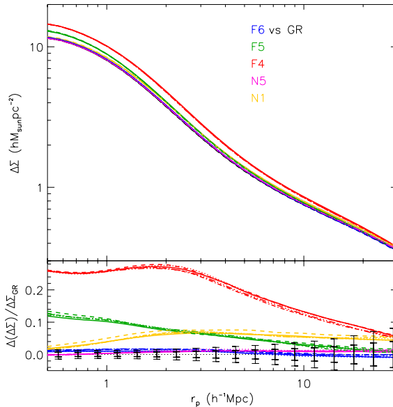
Figure 31. (Color Online) The excess surface mass density profiles, \Delta\Sigma , measured at z = 0.5 , for the six models studied here: GR (black), F6 (blue), F5 (green), F4 (red), N5 (magenta) and N1 (orange). The lower sub-panel shows the relative differences with respect to GR, where the black horizontal dotted line is zero, and the thick and thin error bars indicate respectively the statistic uncertainties in an optimistic and a pessimistic case, in which an LSST-like imaging survey has 6,000 and 1,500 sq. deg. overlap with a DESI-like survey. We have used different lines styles to represent the five realisations, instead of showing their mean, to highlight the small scatter across the different realizations.
