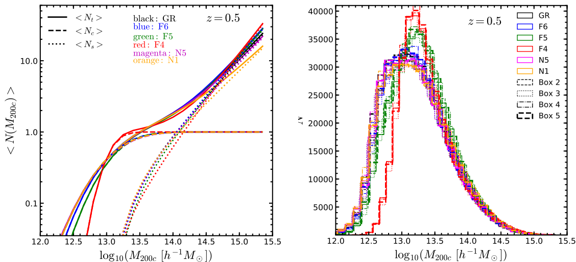
Figure 3. (Color Online) Left panel: the mean galaxy number as a function of host halo mass for central (dashed), satellite (dotted) and all (solid) galaxies for \Lambda CDM and the five MG models. The figure is made using eq. (2.16) with the tuned HOD parameters (cf. table 2) for the individual models. Right panel: histograms of galaxy numbers as a function of the host halo mass for all models and all realizations; this is essentially the product of the mean occupancy number (as shown in the left panel) and the halo mass function. The line colors and styles in the right panel are the same as in figure 1. All results are at z = 0.5 .
