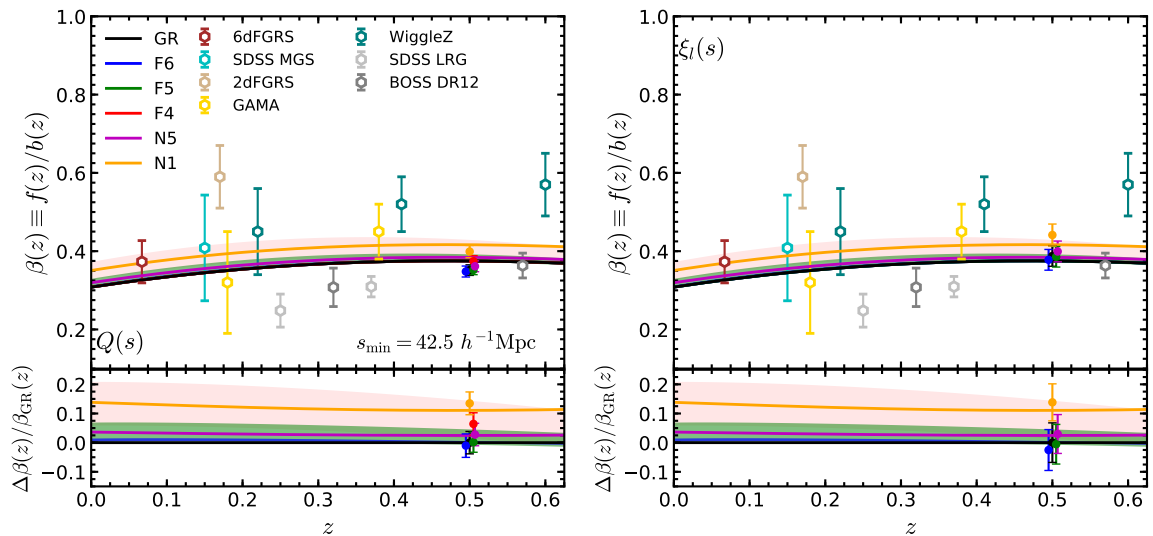
Figure 7. Evolution of \beta as a function of redshift. The curves show the theoretical predictions for the gravity models as shown in the legend, for f(R) gravity models the theoretical predictions are shown as a shaded region for wavenumbers 0.01 \leq k/[h \text{ Mpc}^{-1}] \leq 0.1 . Open coloured symbols correspond to current constraints from observational galaxy survey data: 6dFGRS [116], SDSS MGS [117], 2dFGRS [118], GAMA [119], Wiggle Z [120], SDSS LRG [121] and BOSS DR12 [122]. Filled symbols, at z = 0.5 , denote the \beta estimates obtained from the simulations using the summary statistics— Left panel : Q(s) eq. (3.7) using linear theory; Right panel : \xi_l(s) eq. (3.6) using non-linear theory with s_{\min} = 42.5 h^{-1} \text{Mpc} at z = 0.5 . The lower subpanels show the relative difference between the modified gravity models and GR. Error bars correspond to the 1\sigma confidence level.
