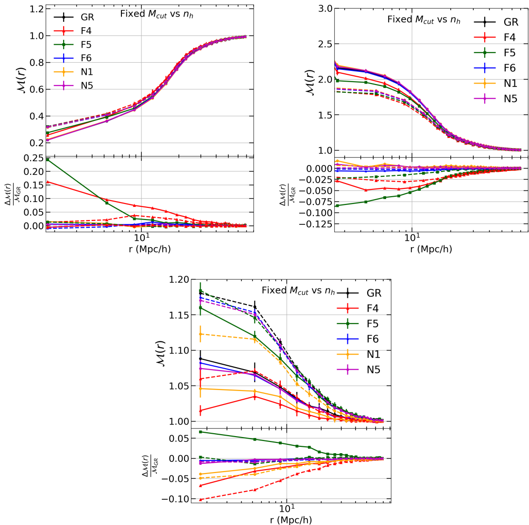
Figure 34. (Color Online) A comparison of the marked correlation statistic obtained for dark matter halo samples designed with a fixed number density (dashed lines), as compared against the prediction using samples with a fixed mass cut (solid lines) equivalent to the original results of figures 12 (Upper Left), 13 (Upper Right) and 15 (Bottom) of the main paper. All results are in real space.
