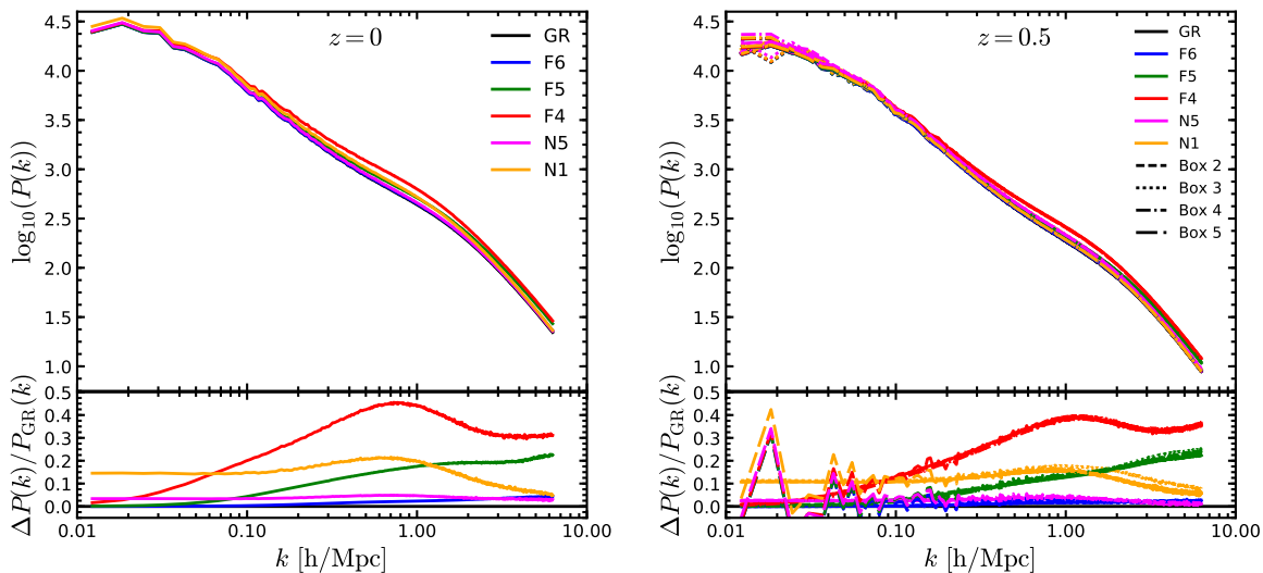
Figure 1. (Color Online) The matter power spectra of the different models compared in this work (upper panels) and their relative differences of the modified gravity models with respect to \Lambda CDM (lower panels). Left panels: results at z = 0 . Right panels: results at z = 0.5 , for all five boxes. This plot sets the convention of line styles that will be used in the rest of this paper: black, blue, green, red, magenta and orange respectively represent GR, F6, F5, F4, N5 and N1, while solid, dashed, dotted, dash-dotted and long-dash-dotted lines represent results from Boxes 1, 2, 3, 4 and 5. This convention will be used in other plots unless otherwise stated. Note that for z = 0 we only show the results for Box 1, while for z = 0.5 we show all five boxes — the upper panel shows the average P(k) from these boxes, while in the lower panel we plot individual curves of \Delta P/P_{\text{GR}} for the five boxes, in order to show the agreement between the different realizations. All power spectra have been measured using the publicly-available code POWMES [78]
