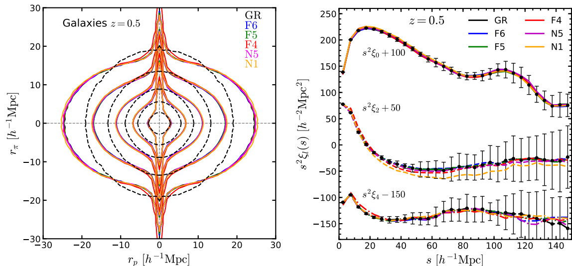
Figure 6. Left panel: the two dimensional galaxy correlation function \xi(r_p, r_\pi) measured from our mock catalogues at z = 0.5 as a function of separation across ( r_p ) and along ( r_\pi ) the line-of-sight. Contours show lines of constant \xi(r_p, r_\pi) at \xi(r_p, r_\pi) = 5, 2, 1, 0.5, 0.25 . The correlation functions correspond to the average of fifteen measurements obtained by projecting five realizations over the three LOS directions. The black dashed contours correspond to the real-space measurements of the correlation function at the same values of its counterpart in redshift-space, for simplicity we show the GR case only for these contours. Right panel: monopole, quadrupole and hexadecapole moments of the correlation function, eq. (3.6), for our six gravity models at z = 0.5 . The moments have been shifted by a factor of 100, 50 and -150 for better visualization. The error bars correspond to the standard deviation over fifteen GR measurements. Different colour line correspond to different gravity model as specified in the legend.
