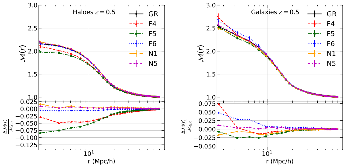
Figure 13. (Color Online) Comparison of the tracer-number-density marked correlation statistic for dark matter haloes (left) and galaxies (right) for the case of up-weighting high density regions ( \rho_* = 1, p = -1 ), for GR (black), f(R) with |f_{R0}| = 10^{-4} (red), |f_{R0}| = 10^{-5} (green), |f_{R0}| = 10^{-6} (blue) and nDGP with r_c H_0 = 1 (orange), r_c H_0 = 5 (magenta). The curves correspond to the averages over the 5 realizations. The bottom panels show the fractional deviation \Delta\mathcal{M}/\mathcal{M} = \mathcal{M}_{\text{MG}}/\mathcal{M}_{\text{GR}} - 1 for each MG model. The error bars correspond to the standard deviations over the 5 boxes.
