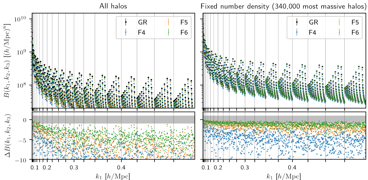
Figure 35. (Colour Online) Real-space bispectrum measured from halo catalogs using either all identified halos in the simulation box (left panels), or the 340,000 most massive ones (right panels).
