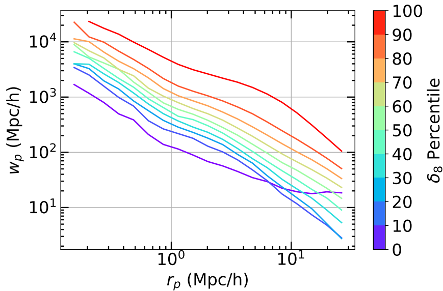
Figure 17. The projected correlation function, w_p(r_p) , estimated for GR HOD catalogues at redshift z = 0.5 . The different colored line show the w_p for over-density ( \delta_8 ) percentiles indicated by the colorbar. At small scale ( r_p < 5 h^{-1}\text{Mpc} ) the clustering amplitude increases with \delta_8 monotonically. At larger scale the clustering amplitude shows non-monotonic behavior with \delta_8 as expected [206].
