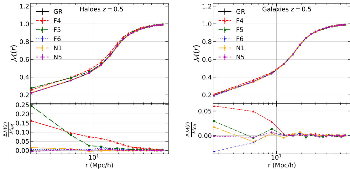
Figure 12. (Color Online) The tracer-number-density marked correlation statistic for halos (left) and galaxies (right) with \rho_* = 4, p = 10 , for GR (black), f(R) with |f_{R0}| = 10^{-4} (red), |f_{R0}| = 10^{-5} (green), |f_{R0}| = 10^{-6} (blue) and nDGP with r_c H_0 = 1 (orange), r_c H_0 = 5 (magenta). The curves correspond to the averages over the 5 realizations of HOD catalogs, while the bottom panels are the fractional deviation \Delta\mathcal{M}/\mathcal{M} = \mathcal{M}_{\text{MG}}/\mathcal{M}_{\text{GR}} - 1 for each MG model. The error bars correspond to the standard deviations over the 5 boxes. The results shown are all in real space.
