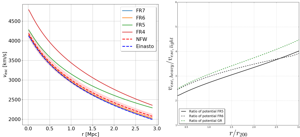
Figure 29. (Color Online) Left: the expected radial escape velocity profile for a stacked high mass ( 10^{15}M_{\odot} ) cluster with \sim 5000 member galaxies. The shaded region includes nominal 5% error from the weak-lensing inference of the gravitational potential. Right: the same as in the left panel, but shows the ratio between the high mass and low mass clusters escape velocities. This probe utilizes the ratio for two reasons: (1) we expect the inner \sim 0.5 Mpc of high mass clusters to look like GR, which sets a lever-arm for the detection of f(R) signals in lower mass systems; (2) this removes a primary systematic, the under-sampling which suppresses the true escape edge. Note that the color schemes are different in the two panels, as indicated in the legends.
