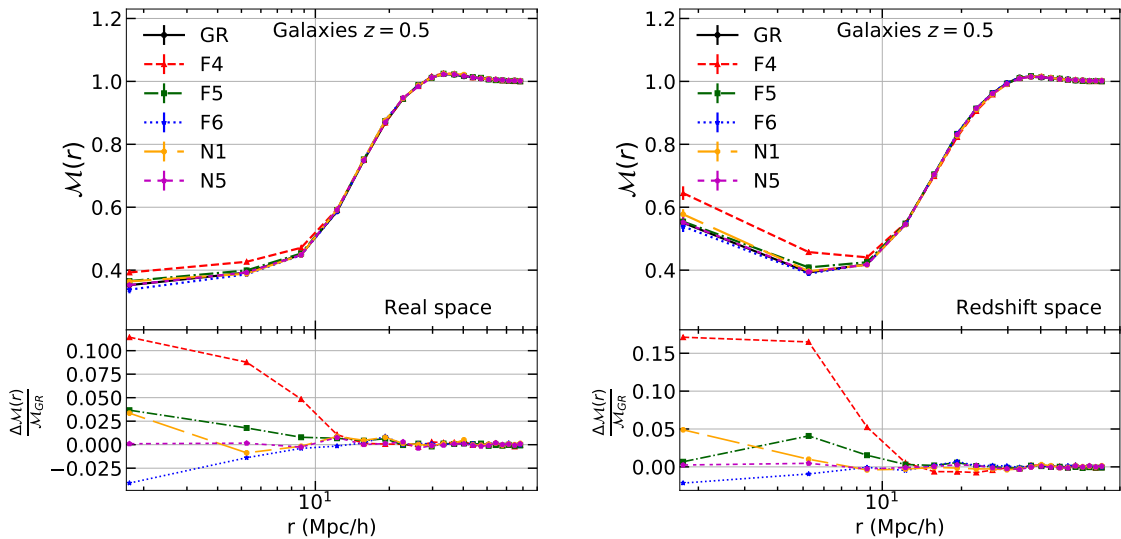
Figure 14. (Color Online) Comparison of the galaxy-number-density marked correlation statistic for galaxies with \rho_* = 4, p = 10 , for GR (black), f(R) with |f_{R0}| = 10^{-4} (red), |f_{R0}| = 10^{-5} (green), |f_{R0}| = 10^{-6} (blue) and nDGP with r_c H_0 = 1 (orange), r_c H_0 = 5 (magenta) when using SPH spline kernel interpolation for density estimate in real space (left) and redshift space (right). The curves correspond to the averages over the 5 realizations (in redshift space we consider 3 directions of each realization as independent samples), while the bottom panels show the fractional deviation \Delta\mathcal{M}/\mathcal{M} = \mathcal{M}_{\text{MG}}/\mathcal{M}_{\text{GR}} - 1 for each MG model. The error bars correspond to the standard deviations over the 5 boxes.
