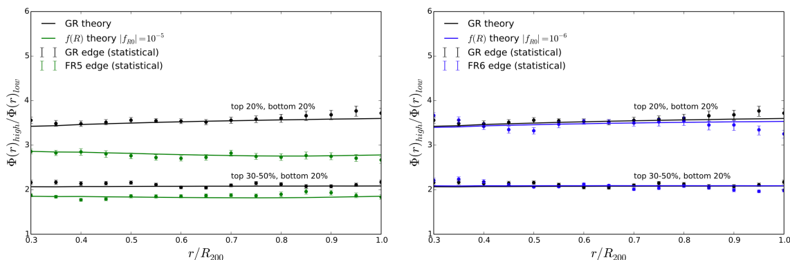
Figure 30. The z = 0 gravitational potential ratio between high and low mass bins (of 20 halos) for GR (black), and the F5 ( left ) (green) and F6 ( right ) parametrization of modified gravity (blue). The points are the averages of the square of the measured radial escape velocities using the simulation particles for each bin in radius and mass. The errors are 1\sigma on the mean from boot-strap re-sampling. The solid lines represent the theoretical predictions using the NFW density parameter. The separation between GR and f(R) potential ratios increases with increasing separation in the mass bins and we show two different mass binning schemes in each panel where the percentages denote the percentiles of cluster masses we keep in the sample. Note the large difference between the GR and F5 ratios at either mass binning scheme. Note the precise and accurate agreement between the theory and the measured escape profile (or \Phi ) profile ratios. These figures justify our use of only theory in making predictions without the need for additional simulations at differing levels of f_{R0} .
