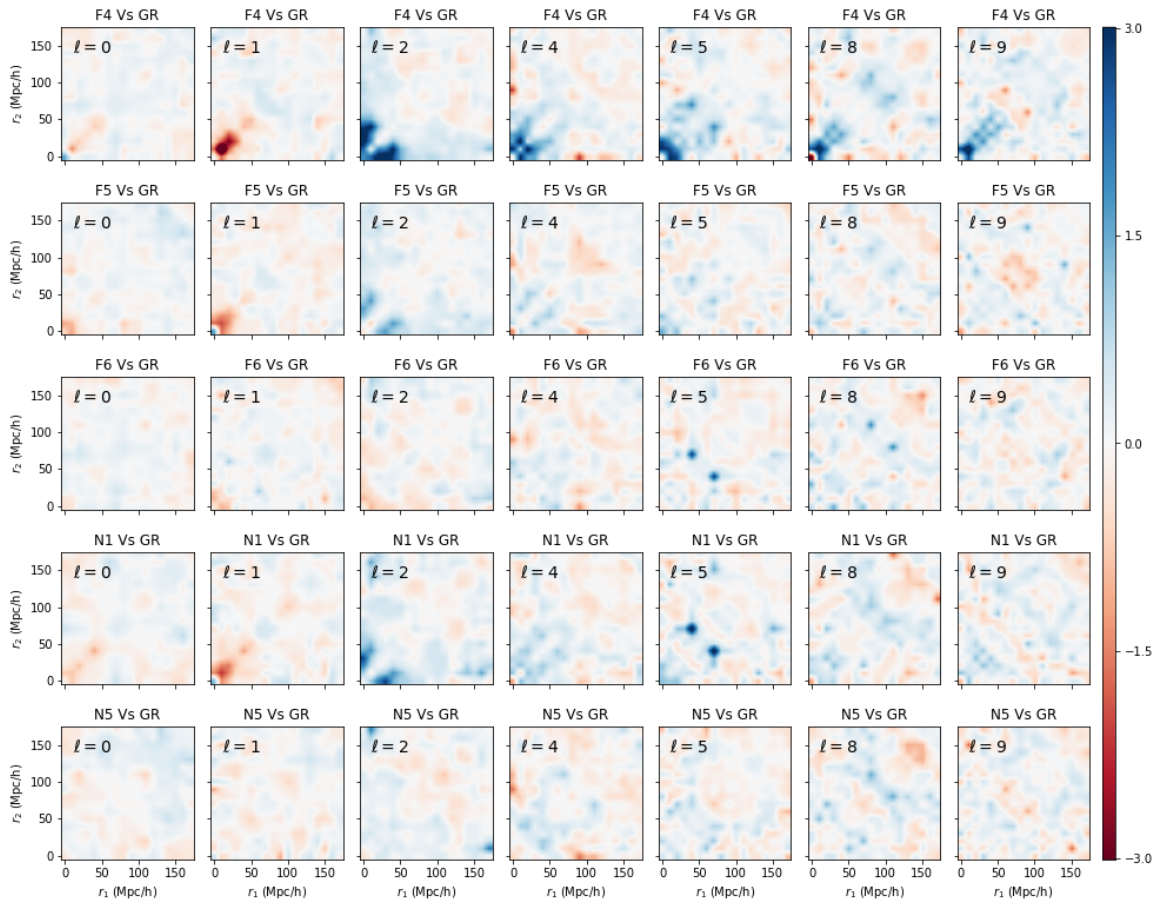
Figure 19. 3PCF comparison of the models using the variable \Delta_{\sigma}^{(3)}\xi_{\ell} defined in eq. (3.25) and the multipole decomposition. Saturated regions may reach values beyond the colorbar shown. We use 18 bins of 10h^{-1}\text{Mpc} each for the triangle sides.
