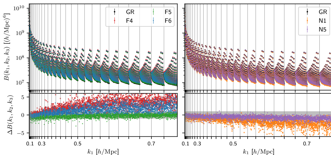
Figure 22. Upper panels: real-space bispectrum measurements for f(R) models (left) and nDGP models (right) compared to GR. Each data point corresponds to one of the 2825 triangle configurations, ordered according to when they appear in the measurement loop. Vertical lines are spaced by the bin width \Delta k \approx 0.025 h/\text{Mpc} and indicate the value of k_1 , i.e., the largest triangle side. Lower panels: difference between modified gravity models and GR quantified in terms of the variable \Delta B given in eq. (3.27). The grey band marks the 1\text{-}\sigma area where deviations are compatible with the combined standard deviation of GR and a given modified gravity model.
