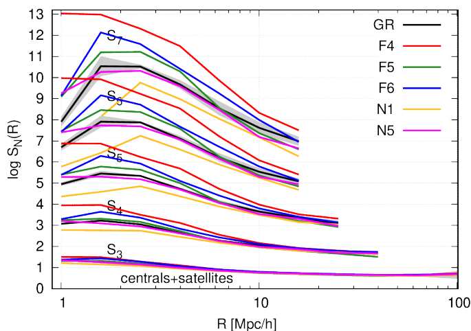
Figure 25. The hierarchy of galaxy clustering reduced cumulants S_n 's for all models. The shaded regions represent 1\sigma scatters around the GR ensemble mean. The groups of lines from the bottom ( S_3 or skewness) to the top ( S_7 ) correspond to increasing cumulant order.
