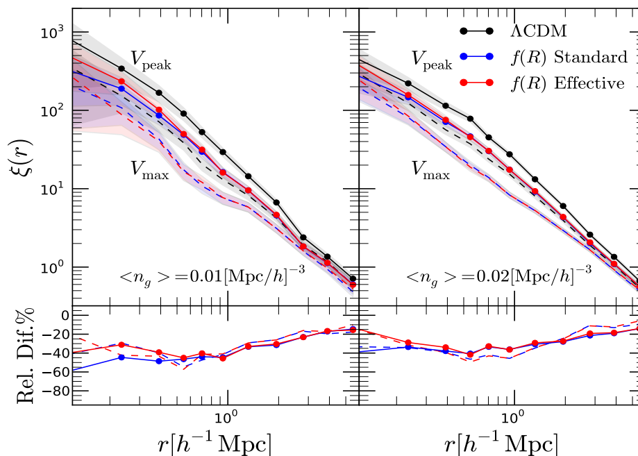
Figure 9. The predicted three-dimensional two-point galaxy correlation functions from the SHAM model (upper panels). The shaded regions represent the 1\sigma Poisson errors. The lower panels show the fractional differences between the f(R) model and \Lambda\text{CDM} . The left panels show the results for a galaxy density \langle n_g \rangle = 0.01 [h^{-1}\text{Mpc}]^{-3} and the right panels are for \langle n_g \rangle = 0.02 [h^{-1}\text{Mpc}]^{-3} . For comparison, the dashed lines show the results obtained using the current maximum circular velocity v_{\text{max}} . The plot is reproduced from ref. [132]
