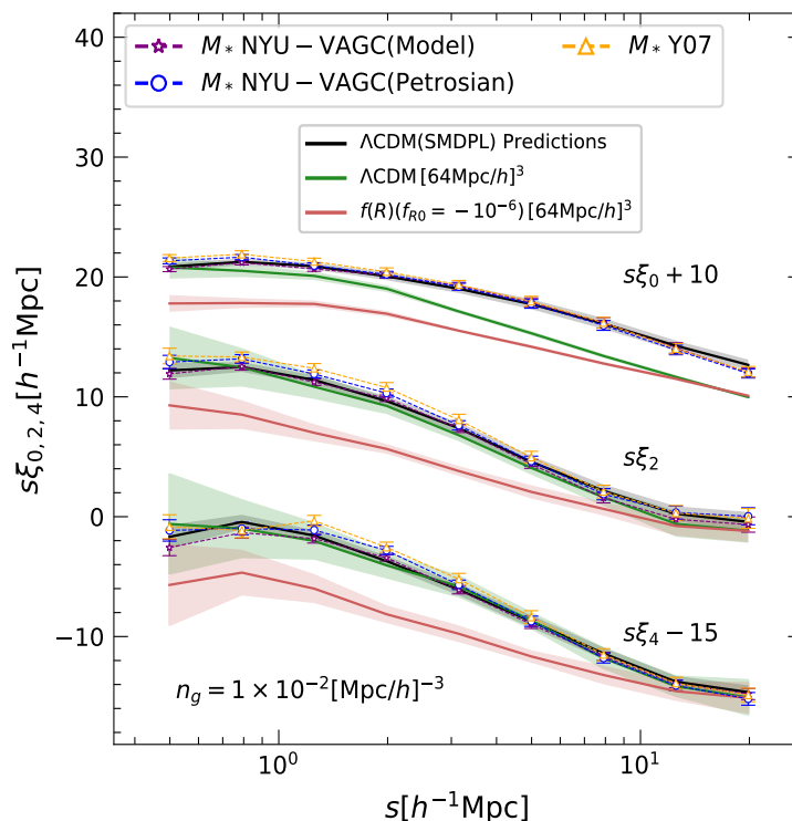
Figure 8. A comparison of RSD measurements using three different stellar mass models: a template-fit method adopted in the NYU catalog with the SDSS model magnitude (stars with dashed line), the same template-fit method but with the SDSS Petrosian magnitude (circles with dashed lines), and a single-color method (triangles with dashed lines). Different stellar mass models give rise to convergent results. The error-bars in the above plot are estimated using a jackknife re-sampling technique with 133 realizations. Here the error-bars represent 3\sigma statistical error. The predicted RSD multipoles (monopole \xi_0 , quadrupole \xi_2 and hexadecapole \xi_4 ) in \Lambda CDM from SHAM mock are in good agreement with observations. Note that the SHAM mock is based on the SMDPL simulation [133] and has the same geometry as the real data. The plot is reproduced from [97]. The green and red lines show the predicted RSD multipoles for \Lambda CDM and f(R) gravity using a suite of simulations with 64 [h^{-1}\text{Mpc}]^3 box size. The shaded regions give the 1\sigma uncertainty around the expectation value, derived from 500 realizations with line-of-sight along different directions of the simulation box. Despite the deficit of power in the monopole due to the small box size of the simulations, the higher order multipoles, such as quadrupole \xi_2 and hexadecapole \xi_4 , show significant differences, indicating that even a model like F6 can be testable given the accuracy of the clustering measurement of DESI.
