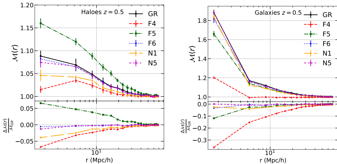
Figure 15. Gravitational potential marked correlation function with \Phi_* = -5.295 and \sigma_\Phi = 0.1 at z = 0.5 for halos (left panel) and galaxies (right panel). The curves correspond to the averages over the 5 realizations. Different colors and line styles correspond to different models as labeled. The lower panels show the relative difference between the MG models and GR, and the error bars correspond to the standard deviation over the 5 realizations.
