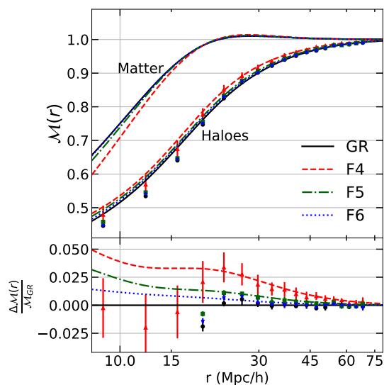
Figure 16. The Zel’dovich-approximation prediction of the marked correlation function eq. (3.14) with \rho_* = 4 and p = 10 , for models F4 (shown in dashed red curves), F5 (dot-dashed green), F6 (dotted blue), and GR (solid black) at redshift z = 0.5 . The data points are the simulation results taken from figure 12: black data points with error bars are for GR, blue for F6, green for F5, and red for F4. The lower panel shows the relative differences in the marked correlation function for tracers (and the data) with respect to the Zel’dovich approximation in GR.
