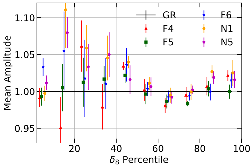
Figure 18. The mean amplitude as a function of over-density ( \delta_8 ). The different MG models are shown with different colors, and the 1\text{-}\sigma errors are computed as the error on the mean of the 5 HOD catalogs. The F4, F5, and N1 models show large \chi^2 values and should be detectable at better than 3\sigma significance but F6 and N5 are very close to GR and do not show any statistically significant difference. Note the points representing different models at same over-density are slightly shifted horizontally to avoid clutter and increase visibility.
