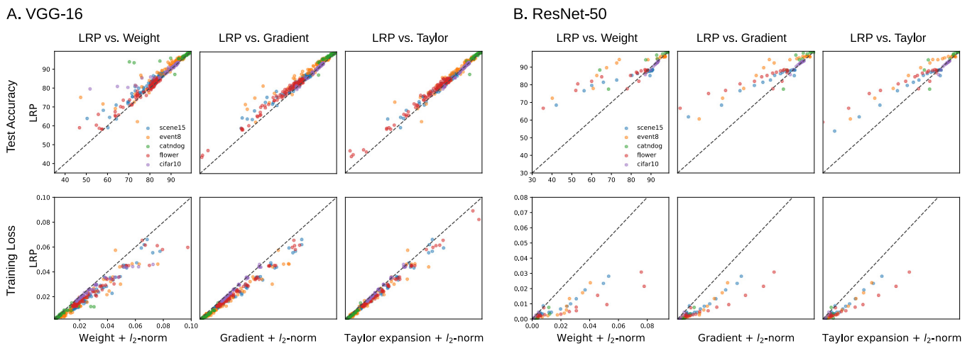
Fig. 6. Performance comparison of the proposed method (i.e., LRP) and other criteria on VGG-16 and ResNet-50 with five datasets. Each point in the scatter plot corresponds to the performance at a specific pruning rate of two criteria, where the vertical axis shows the performance of our LRP criterion and the horizontal axis the performance of a single other criterion (compare to Fig. 5 that displays the same data for more than two criteria). The black dashed line shows the set of points where models pruned by one of the compared criteria would exhibit identical performance to LRP. For accuracy, higher values are better. For loss, lower values are better.
