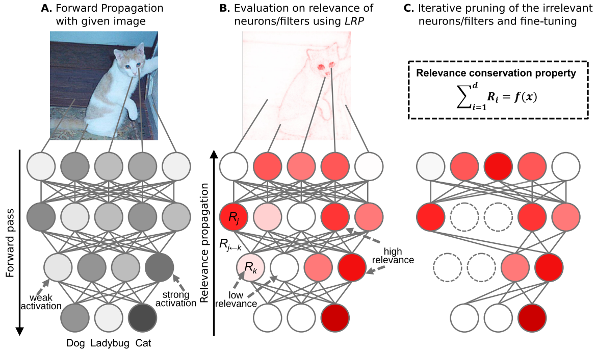
Fig. 1. Illustration of the LRP-based sequential process for pruning. A. Forward propagation of a given image (i.e. here, of a cat) through a pre-trained model. B. Evaluation on relevance for weights/filters using LRP. C. Iterative pruning by eliminating the least relevant units (depicted by circles) and fine-tuning if necessary. The units can be individual neurons, filters, or other arbitrary grouping of parameters, depending on the model architecture.
