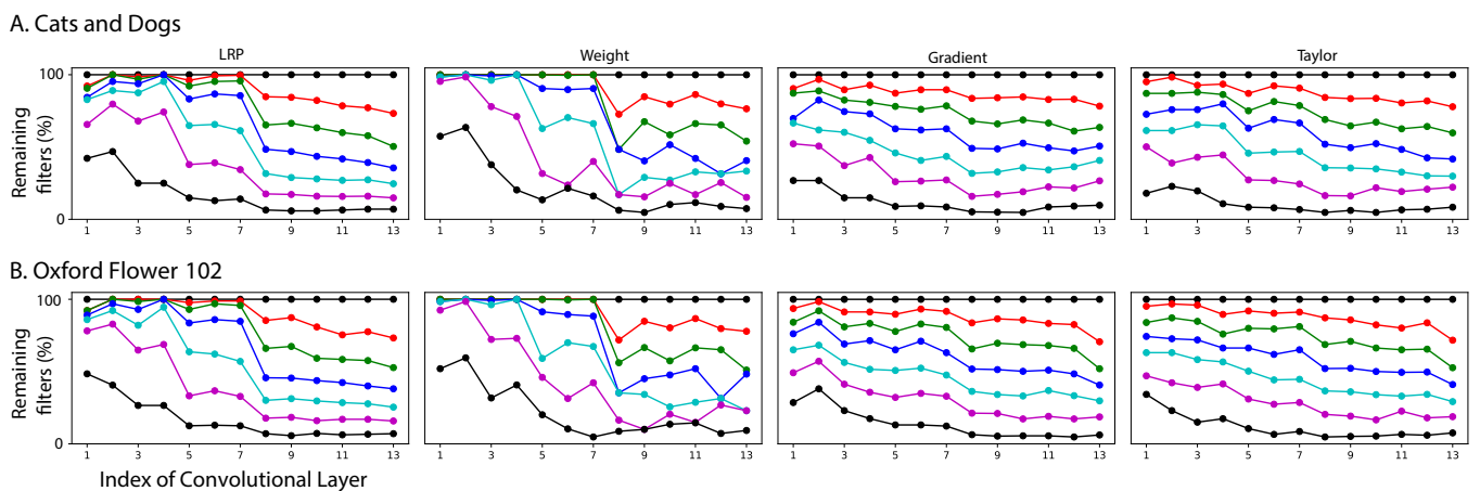
Fig. 7. An observation of per-layer pruning performed w.r.t the different evaluated criteria on VGG-16 and two datasets. Each colored line corresponds to a specific (global) ratio of filters pruned from the network (black (top) : 0%, red : 15%, green : 30%, blue : 45%, violet : 75% and black (bottom) 90%). The dots on each line identify the ratio of pruning applied to specific convolutional layers, given a global ratio of pruning, depending on the pruning criterion. (For interpretation of the references to colour in this figure legend, the reader is referred to the web version of this article.)
