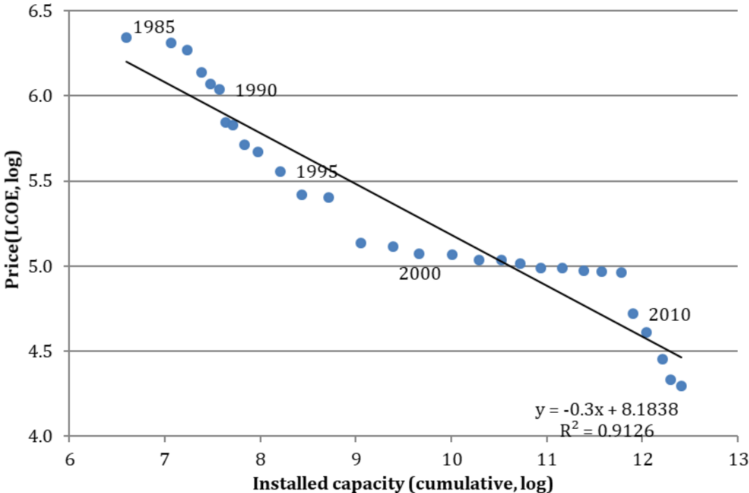
Figure 4. Cost of generating electricity from wind power (per MWh)
