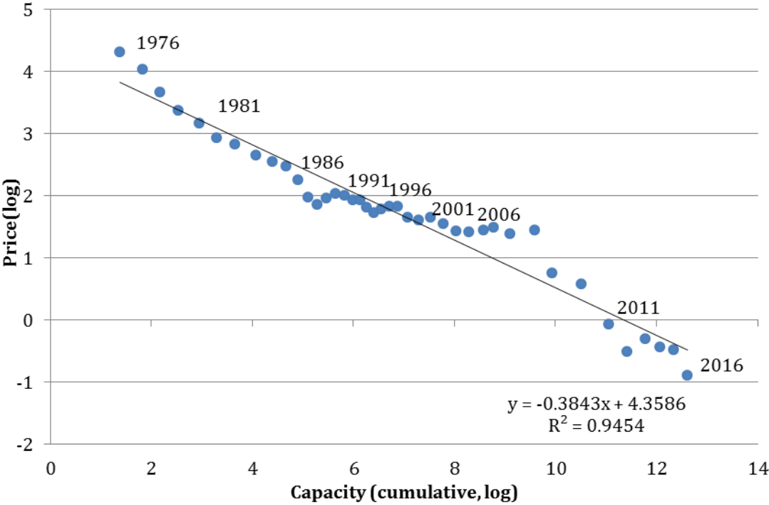
Figure 3. Solar energy: Price of a PV-module (per watt)
