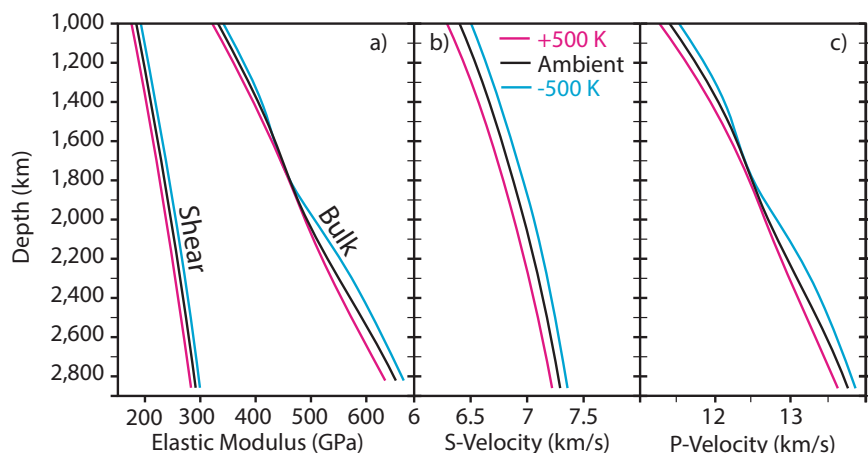
Fig. 2 Depth dependence of elastic moduli and seismic velocities for pyrolite composition listed in Table 1 15 . a Shear and bulk moduli. The anomalous behaviour of the bulk modulus, K^{II} ( K = -V(dP/dV) , where V is volume and P is pressure) is due to the iron octahedron volume collapse during the spin-state change 4 associated with the spin crossover. As previously shown 11 , the pressure onset, the pressure range of the HS-LS crossover, and associated anomalies in K are temperature dependent (same legend all panels). The shear modulus, G , ( G = \tau/\gamma , where \tau is the shear stress and \gamma is the shear strain) is not significantly affected by the octahedron volume reduction and increases monotonically with increasing pressure and decreasing temperature. b S-wave ( V_s = \sqrt{G/\rho} ) and c P-wave ( V_p = \sqrt{(K + 4/3G)/\rho} ) velocity for pyrolite at different temperatures. The average mantle temperature profile (black) is calculated by setting the starting temperature to 1873 K at 660 km, and integrating the adiabatic temperature gradient 15 through the lower mantle. The blue/magenta curves were calculated using the same technique, but decreasing/increasing the temperature at 660 km by \pm 500 K. In the mixed-spin region, the softening of K^{II} causes a reduction in P-wave velocity sensitivity to isobaric temperature variations 14 , while the S-wave velocity remains sensitive to such temperature variations. Consequently, the expected seismic signal of iron-bearing Fp in the lower mantle consists of a disruption of vertically coherent thermal structures in P-velocities, whereas a coherent thermal structure is apparent in the S-velocities 12,14 . Additional compositions shown in Supplementary Fig. 1 demonstrate the calculated seismic velocities dependence on Fp proportion.
