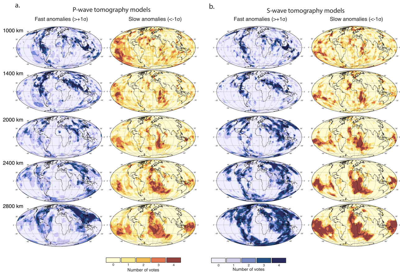
Fig. 5 Vote maps of mantle tomography models. Variable depth vote maps for fast ( >+1\sigma from the mean), and slow ( <-1\sigma from the mean) mantle for all a 4 P-wave and b 4 S-wave tomography models (see Methods) considered here. In general, lower mantle vote maps of fast velocity regions reveal subducted slabs, and slow maps reveal plumes and antipodal large low shear wave velocity provinces (LLSVPs). In this map view, the P-wave model vote maps appear less coherent than the S-wave model vote maps in the fast velocity regions of the mid-mantle. Colour gradients from ref. 73 .
