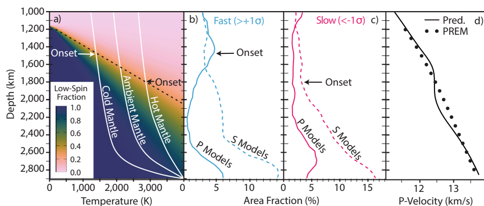
Fig. 1 Comparison of mineral physics predictions and seismological observations of the Fe spin crossover in Fp. a The depth-temperature distribution of low-spin Fe and three schematic mantle geotherms. The onset of the mixed-spin region occurs at shallower depths for relatively colder temperatures and at greater depths and over a broader range at higher temperatures. Surface area of fast ( b ) and slow ( c ) velocities in the lower mantle imaged by unanimous consensus (4/4 models) corresponding to the vote maps shown in Figs. 5 and 6. A divergence in the seismic signal between P-wave models relative to S-wave models is revealed below the respective "onset" depths of ~1400 and 1800 km. d The calculated profile of P-wave velocities for pyrolite 15 (see Supplementary Fig. 9) reveals a significant departure suggesting that the signature of the spin crossover is not a globally averaged feature. See Methods. Colour gradients from ref. 73.
