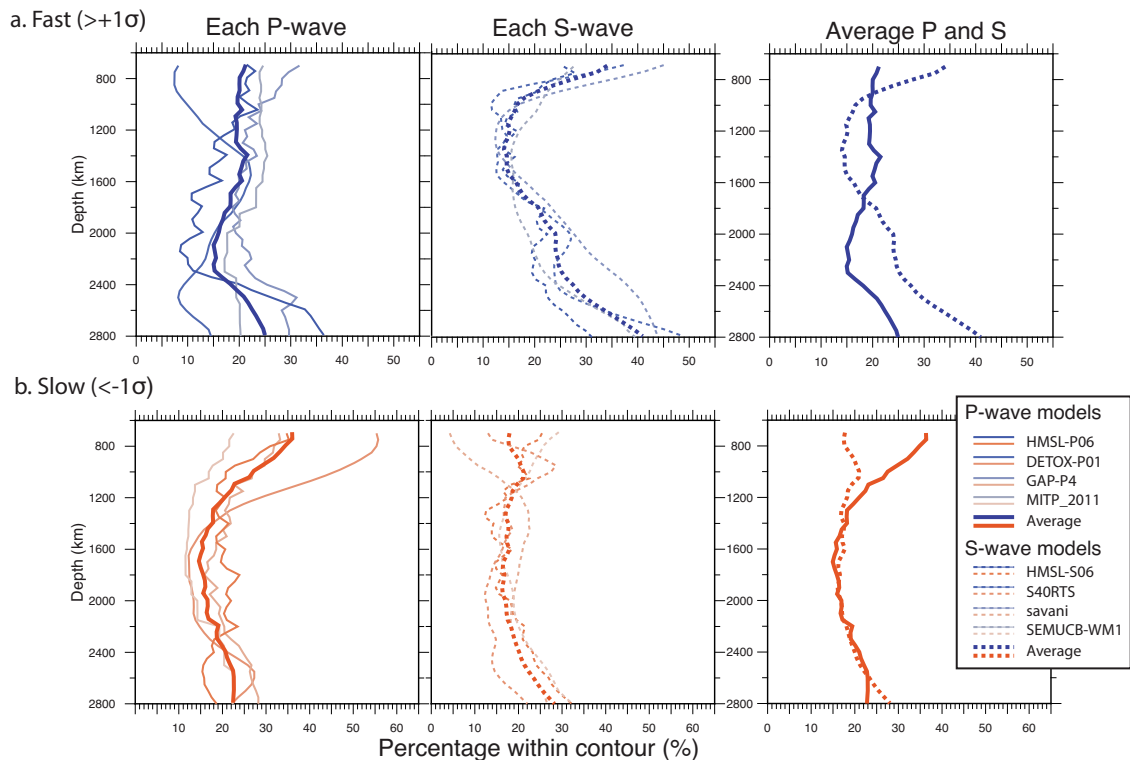
Fig. 4 Changes in surface area for the individual tomography models. Depth-dependent changes in surface area for the a fast ( >+1\sigma from the mean), and b slow ( <-1\sigma from the mean) regions, as applied to each of the 4 P-wave, and 4 S-wave tomography models. The individual model names and details are shown in Supplementary Figs. 2–3. The bold lines are the average of each panel, which are extracted and shown in the rightmost panels. This procedure is similar to that shown in Fig. 1b, c except without the vote map analysis.
