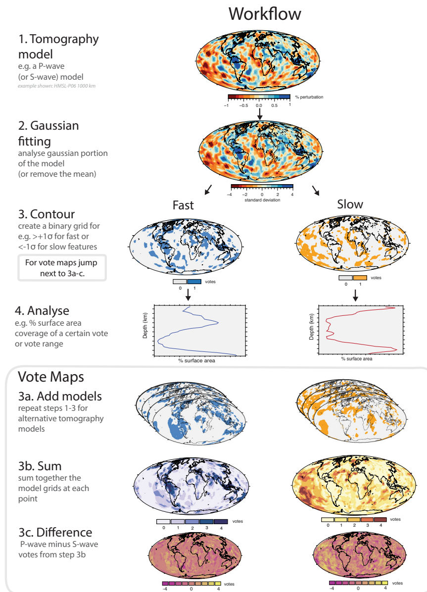
Fig. 3 Workflow used in this paper. Step 1: select tomography model. Step 2: a gaussian fitting procedure is applied (see Methods). Step 3: a contour metric is chosen e.g. fast ( >+1\sigma from the mean), and slow ( <-1\sigma from the mean) and binary grids are created. Step 4: surface area coverage of the contour is extracted across the lower mantle. For the vote map methodology additional steps are applied between Steps 3 and 4. Step 3a: binary grids from additional tomography models are created as per Steps 1-3. Step 3b: at each grid point the constituent models (here 4 models) are summed. Step 3c: difference vote maps can be generated, for example by subtracting the S-wave votes from the P-wave votes.
