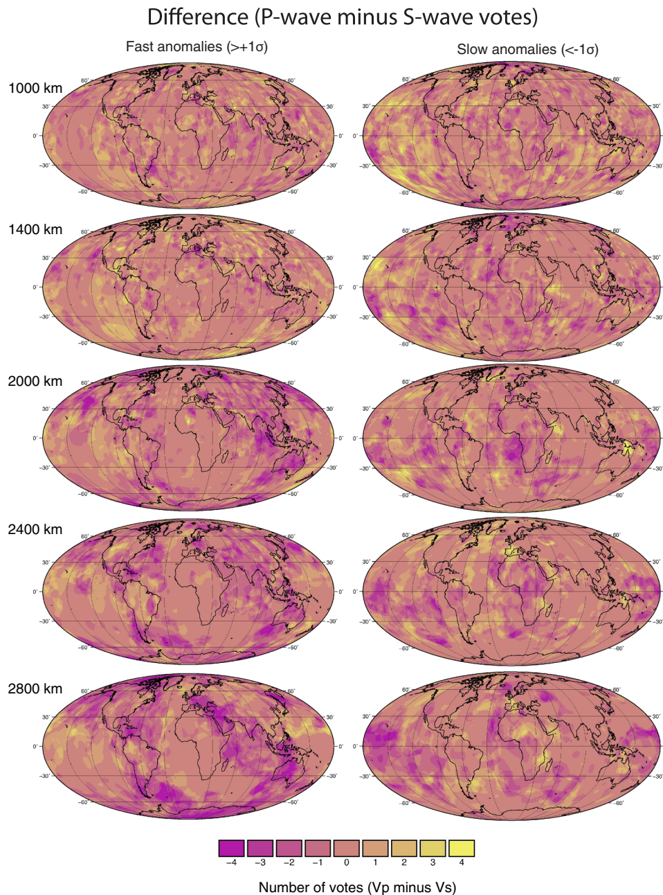
Fig. 7 Difference maps between P-wave and S-wave models. Difference maps for the fast (left panels) and slow (right panels) vote maps constructed by subtracting the S-wave model votes (constructed with 4 models) from P-wave model votes (constructed with 4 models). Yellow areas indicate high votes (i.e. the identification of robust features) in P-wave models but not S-wave models, darker purple areas indicate high votes for S-wave models relative to P-wave models, and central colours indicate regions of mutual agreement.
