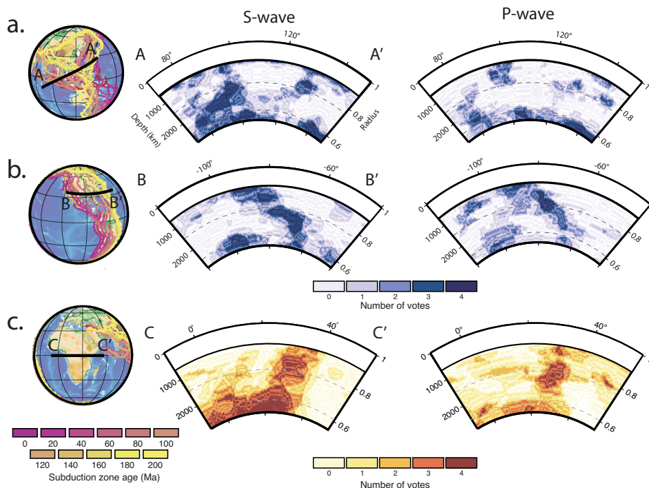
Fig. 6 Vertical cross-sections through the vote maps. All four S-wave models (left) and four P-wave models (right) are used for profiles through (a) SE Asia and (b) the Farallon slab regions (vote maps for fast velocities), and (c) the African-Afar large low shear wave velocity province (LLSVP) and plume region (vote maps for slow velocities). Location maps are overlain with palaeo-subduction zones between 0 and 200 Ma as extracted from a global plate reconstruction 77 . Panels (a) and (b) identify vertically coherent fast regions that are common to S-wave models in the mid-mantle indicating the presence of subducted slabs whereas the slab signal is weak amongst P-wave models. This is more clear in the fast rather than (c) slow regions because at higher temperatures the HS-LS crossover shifts to greater depths where the seismic signal is dominated by the LLSVPs, and also occurs over a broader depth range.
