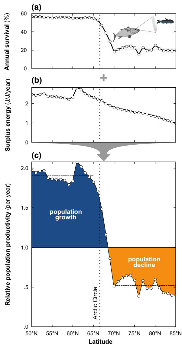
FIGURE 2 Arctic waters are population sinks for diel vertically migrating (DVM) mesopelagic fishes. (a) Our model predicts that annual survival and (b) surplus energy decrease poleward, (c) resulting in a negative population growth at latitudes above the Arctic Circle. Dashed lines indicate the mean across 50–65° and 70–85°N. The spike in surplus energy and population growth around 60°N is explained by cooler deep waters (see Figure 1c) and therefore lower metabolic demands in the Norwegian Sea basin (see Figure 1d)
