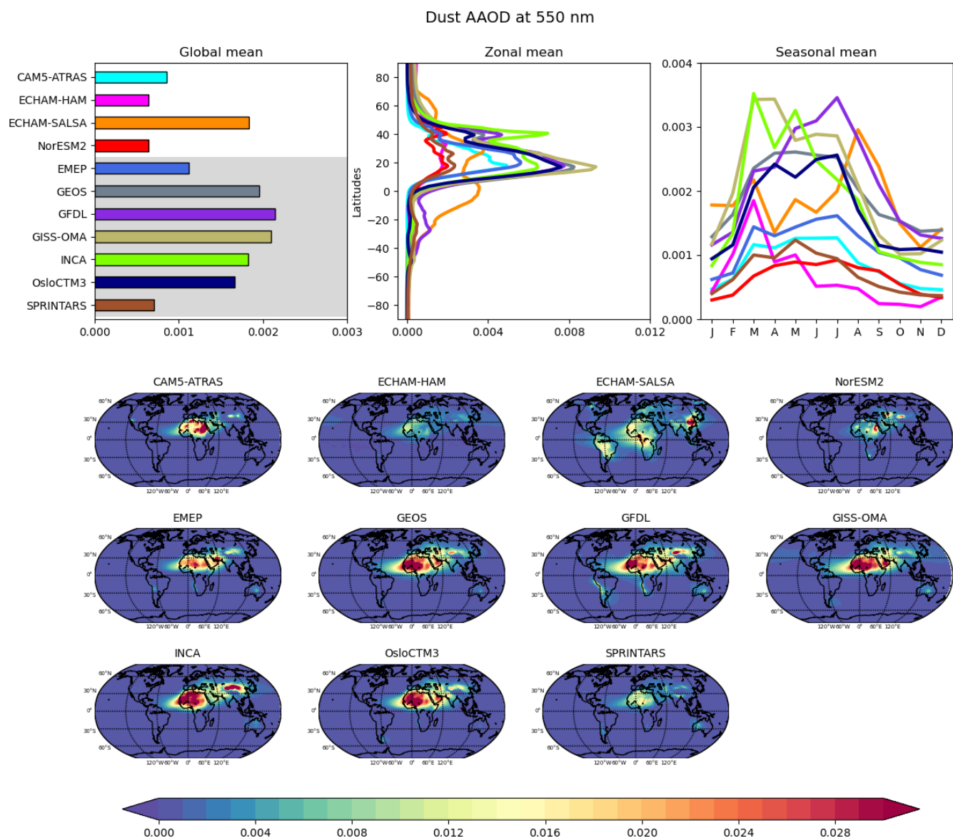
Figure 7. Dust AAOD at \lambda = 550 nm from the models, with annual global mean, annual zonal mean, the global seasonal cycle, and annual mean spatial distributions. The models with grey shading have externally mixed dust.
