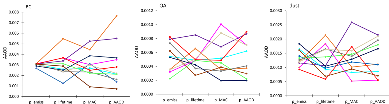
Figure 9. Partial sensitivity of AAOD to variation in emission, lifetime, and MAC for BC, OA, and dust for each model. The sensitivities are calculated by dividing the variable in each model by the AeroCom model mean multiplied with the AAOD AeroCom model mean.
