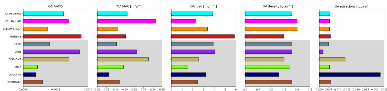
Figure 6. Global mean OA AAOD, OA MAC ( \text{m}^2 \text{g}^{-1} ), OA mass load ( \text{mg m}^{-2} ), OA density ( \text{g cm}^{-3} ), and OA refractive index (imaginary) at 550 nm. The models with grey shading have externally mixed OA. Values for each bar are given in the Supplement (Table S4).
