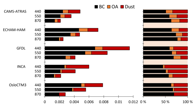
Figure 10. Global mean AAOD at \lambda = 440, 550, and 870 nm for each model split into BC (black), OA (orange), and dust (red), with absolute values on the left and relative values on the right.
