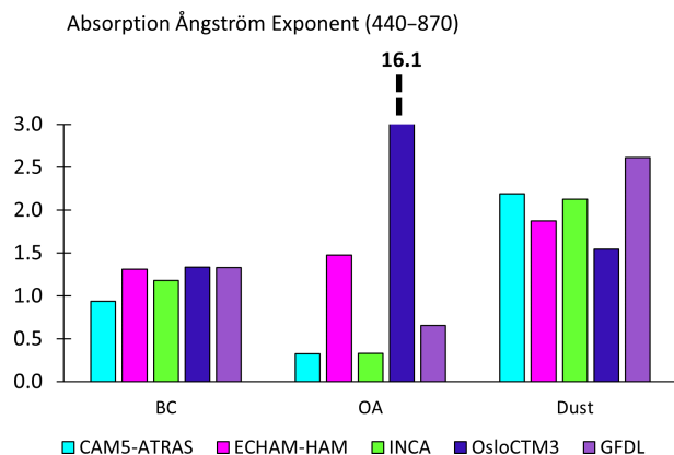
Figure 11. Global mean aerosol absorption Angstrom exponent, based on total AAOD at \lambda = 440 and \lambda = 870 nm, split into BC, OA, and dust.
