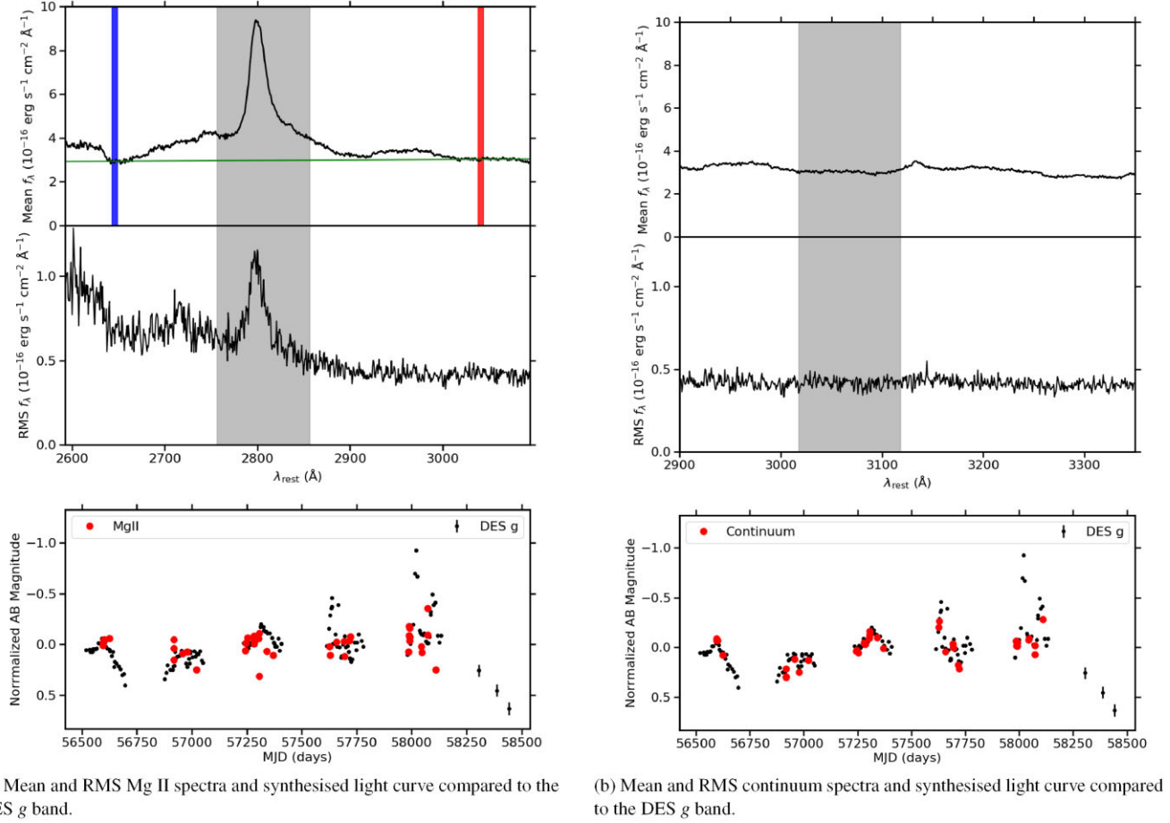
Figure 11. Top panel: The regions of OzDES spectra used to create the synthesised light curves (grey shaded regions). The Mg II line is continuum subtracted by fitting a line for the approximate continuum (green line) between points on either side of the emission line region (the blue and red shaded regions). Middle panel: RMS Spectra. Lower panel: Synthesised light curves created from spectra compared to the DES photometric light curves.
