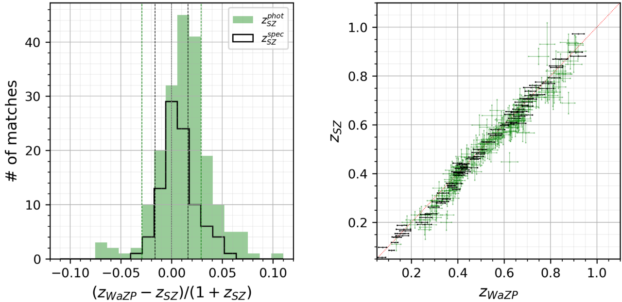
Figure 14. Distribution of redshift separations (left-hand panel) and relation between the redshifts (right-hand panel) of WaZP-SZ matched clusters split into spectroscopic and photometric redshift samples.
