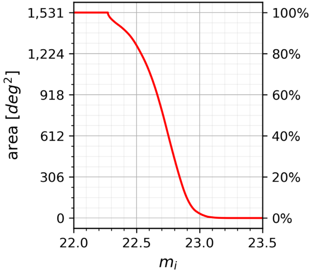
Figure 1. The effective area coverage of DES-Y1 as a function of the limiting magnitude in the i -band.
