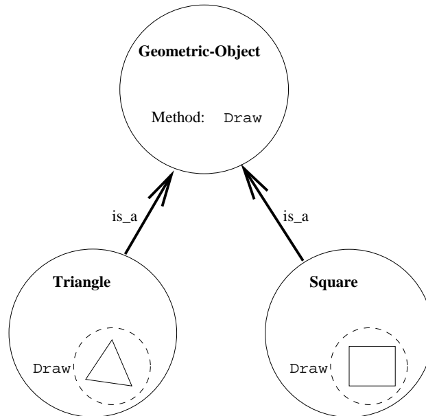
Figure A.1: Dynamic binding - the correct Draw method will be decided at run-time.
