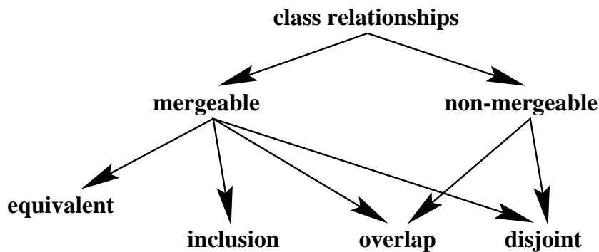
Figure 4.2: Classification
