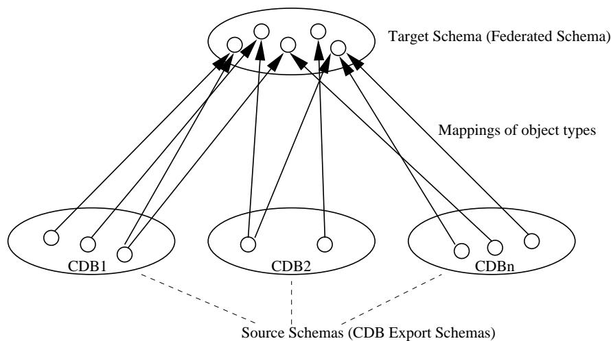
Figure 6.1: The idea of mapping ODL schemas.
