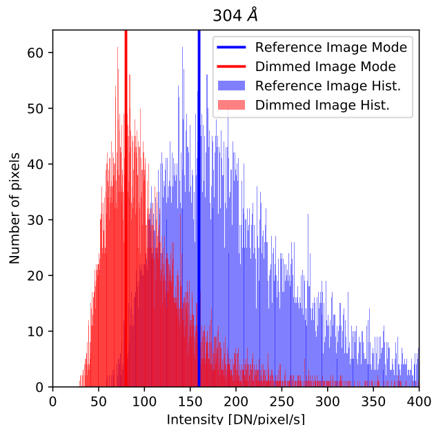
Fig. 4. Histograms of the pixel values for the 304 Å channel. In blue we show the histogram for the reference image, and in red the histogram for the dimmed image. The y-axis is the number of pixels, and the x-axis is the pixel intensity [DN/pixel/s]. The modes are marked with blue and red lines for the reference and dimmed images, respectively.
