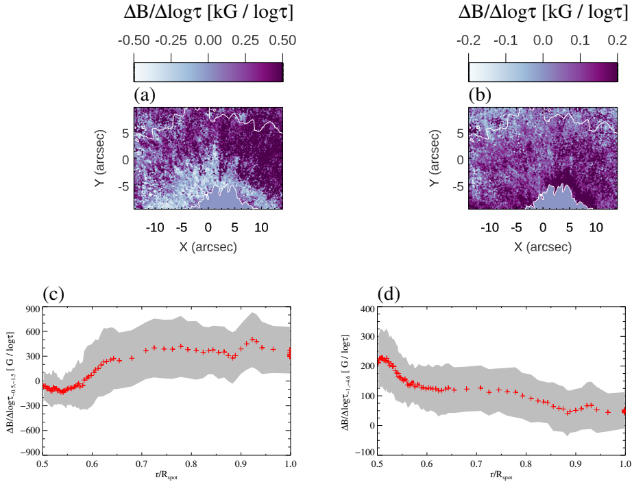
Figure 2. Top panels: Maps of the vertical gradient of the magnetic field strength considering two atmospheric heights in the photosphere (left panel) and two heights representative of the photosphere and chromosphere (right panel). Bottom panels: Variation of the vertical gradient as a function of r/R_{spot} for the subarray A displayed in the top panels.
