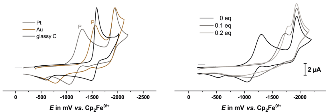
Figure 9. Left: cyclic voltammograms of 8 in DMF/ n Bu 4 PF 6 at v = 0.1 V/s at r.t with a platinum (Pt), a gold (Au), or a glassy carbon (glassy C) electrode. Right: voltammograms with a platinum electrode in the presence of 0, 0.1 or 0.2 equivalents of 2,2,6,6-tetramethylpiperidine base.
