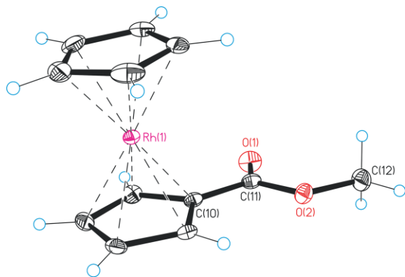
Figure 5. Molecular structure of 11 with thermal ellipsoids at a 50 % probability, counterion PF 6 omitted for clarity. Selected bond lengths [Å]: C(10)–C(11) = 1.480(3), C(11)–O(1) = 1.201(2), C(11)–O(2) = 1.327(2), O(2)–C(12) = 1.449(2).
