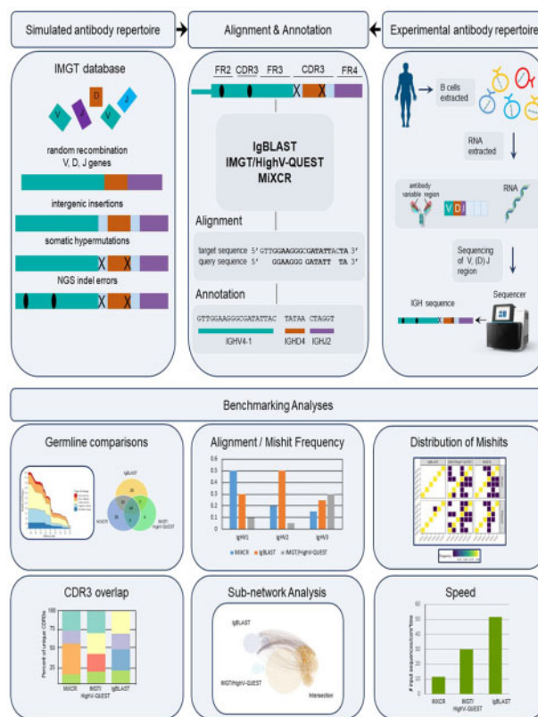
Fig. 1. Schematic of immuneinformatic benchmarking analysis. Top, Left side: Antibody repertoire data were simulated in silico using IgSimulator. Right side: Experimental antibody repertoire data was collected from publically available datasets. Top, Middle: Alignment and annotation of simulated and experimental sequences were performed with the immunoinformatic tools: IgBLAST, IMGT/HighV-QUEST and MiXCR. Bottom: Downstream analysis of the results compared: (i) the germline databases (ii) alignment (iii) frequency of mismatches of the V, D and J gene annotations (iv) unique CDR3 overlap (v) sub-network analysis and (vi) speed of analysis
