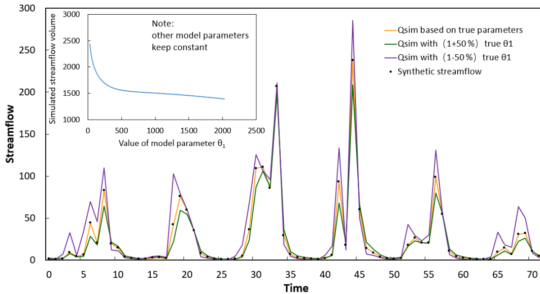
Figure 2. Example of the impacts on model simulation due to the different shifts in model parameter \theta_1 (that denotes the catchment water storage capacity). Qsim refers to the simulated streamflow.
