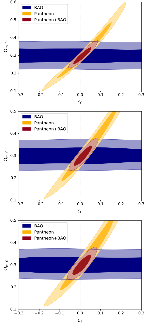
Fig. 1. 2D contours on \Omega_{m,0} , \epsilon_0 and \epsilon_1 , using currently available data for BAO (blue), SnIa (yellow) and the combination of the two (red). These results refer to the constant ( top panel ) and binned ( central and bottom panels ) \epsilon(z) cases.
