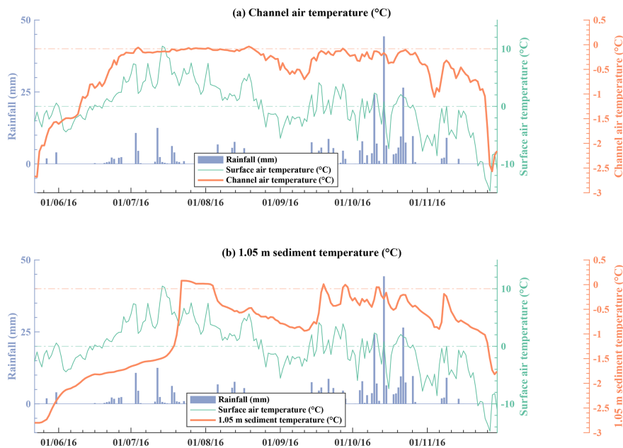
Figure 6. Daily subglacial temperatures compared to weather conditions at Larsbreen in 2016. (a) Time series of subglacial channel air temperature, modeled surface air temperatures and modeled rainfall. (b) Time series of subglacial sediment temperature, modeled surface air temperature and modeled rainfall.
