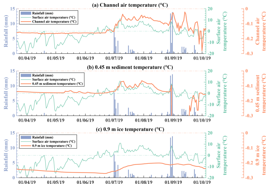
Figure 8. Subglacial temperatures at location Subglacial 1. (a) Time series of daily mean channel air temperature, modeled surface air temperature and modeled rainfall. (b) Time series of daily mean 0.45 m depth sediment temperature, modeled surface air temperature and modeled rainfall. (c) Time series of daily mean 0.9 m depth ice temperature, modeled surface air temperature and modeled rainfall.
