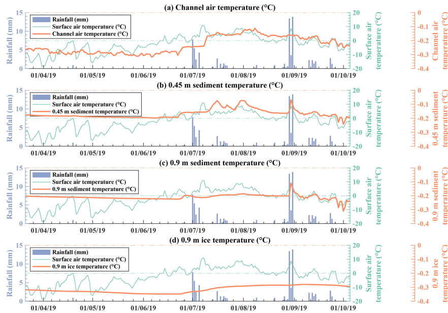
Figure 9. Subglacial temperatures at location Subglacial 2. (a) Time series of daily mean channel air temperature, modeled surface air temperature and modeled rainfall. (b) Time series of daily mean 0.45 m depth sediment temperature, modeled surface air temperature and modeled rainfall. (c) Time series of daily mean 0.9 m depth sediment temperature, modeled surface air temperature and modeled rainfall. (d) Time series of daily mean 0.9 m depth ice temperature, modeled surface air temperature and modeled rainfall.
