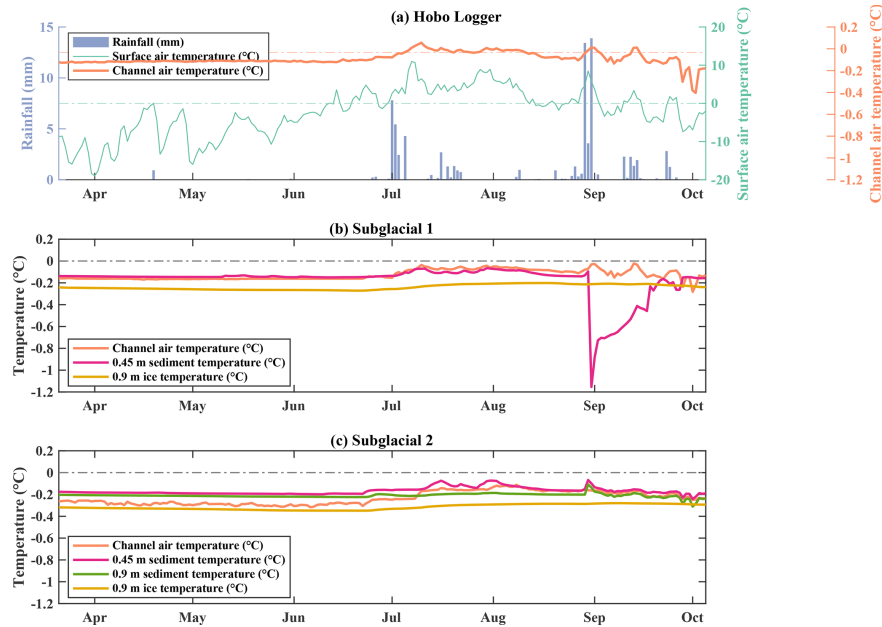
Figure 7. Observed subglacial daily mean temperatures at Tellbreen during 2019. Panel (a) Time series of subglacial channel air temperature at Hobo location compared to modeled surface air temperature and modeled rainfall. (b) Channel air, 0.45 m depth sediment and 0.9 m depth ice temperature at location Subglacial 1 next to the source of the running water. (c) Channel air, 0.45 m depth sediment, 0.9 m depth sediment and 0.9 m depth ice temperature at location Subglacial 2 at the end of the drainage system.
