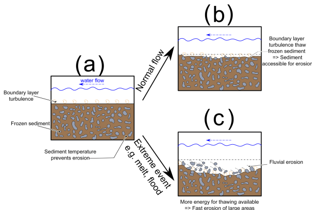
Figure 12. Proposed thermo-mechanical erosion mechanism at the bottom of subglacial channels of cold-based glaciers. (a) Temperatures below freezing prevent the water from eroding material in case of low flow. (b) During summer and normal flow rates boundary layer turbulence thaws the surface layer of the sediment and exposes it to mechanical erosion. (c) Exceptional high flow velocities and available thermal energy cause a rapid sediment thaw, exposing larger areas of the ground to mechanical erosion, and clasts get transported away due to high flow velocities, leading to high erosion rates.
