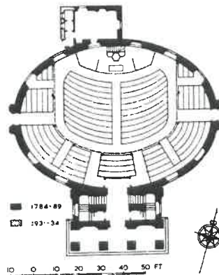
Abb. 66 St. Andrews in Edinburgh/Schottland, 1785
