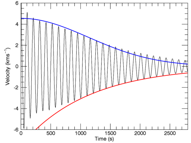
Fig. 7. Velocity at the centre of the flux tube cross-section indicating the damping rate of the kink mode. Two damping profiles are also displayed. Upper: Gaussian (blue) profile. Lower: exponential (red) profile.
