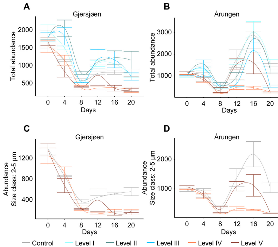
Fig. 5. Temporal changes in total abundances of phytoplankton compared to those belonging to size class (2–5 μm) from lake Gjersjøen (A, C) and lake Årungen (B, D) across treatments (colour coded). Treatment levels I–III, though not shown for the selected size class (2–5 μm) were close to the control. The vertical axes very not scaled and reflect differences between the lakes. Locally estimated scatterplot smoothing (LOESS) was fitted to the data points to generate line plots. The error bars indicate standard error.
