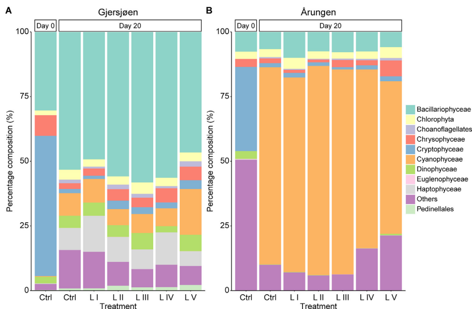
Fig. 6. Relative proportion of major phytoplankton classes identified in (A) Gjersjøen (mesotrophic lake) and (B) Årungen (eutrophic lake) showing: (i) changes in the controls that occurred between the start (day 0) and the end of the experiment (day 20) and (ii) the effects of on PPCPs treatments relative to the control at the end of the experiment (day 20).
