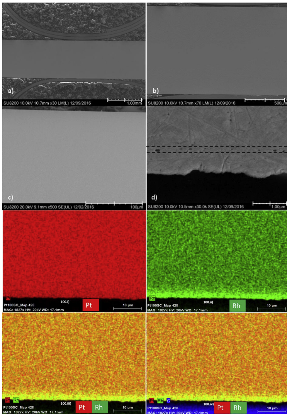
Fig. 5. (top) SEM micrographs of Pt(100) (a–d) coated with 300 nm of Rh and alloyed at 1273 K for 24 h, see scale bar 1 – 500 \mu\text{m} . Notice the voids due to unstable K – plane formation; and (bottom) EDS cross section maps of Pt, Rh, Pt + Rh for Pt(100), scale bar 10 \mu\text{m} , clearly showing the depth based decay of Rh concentration (Pt in red, Rh in green). (For interpretation of the references to colour in this figure legend, the reader is referred to the Web version of this article.)
