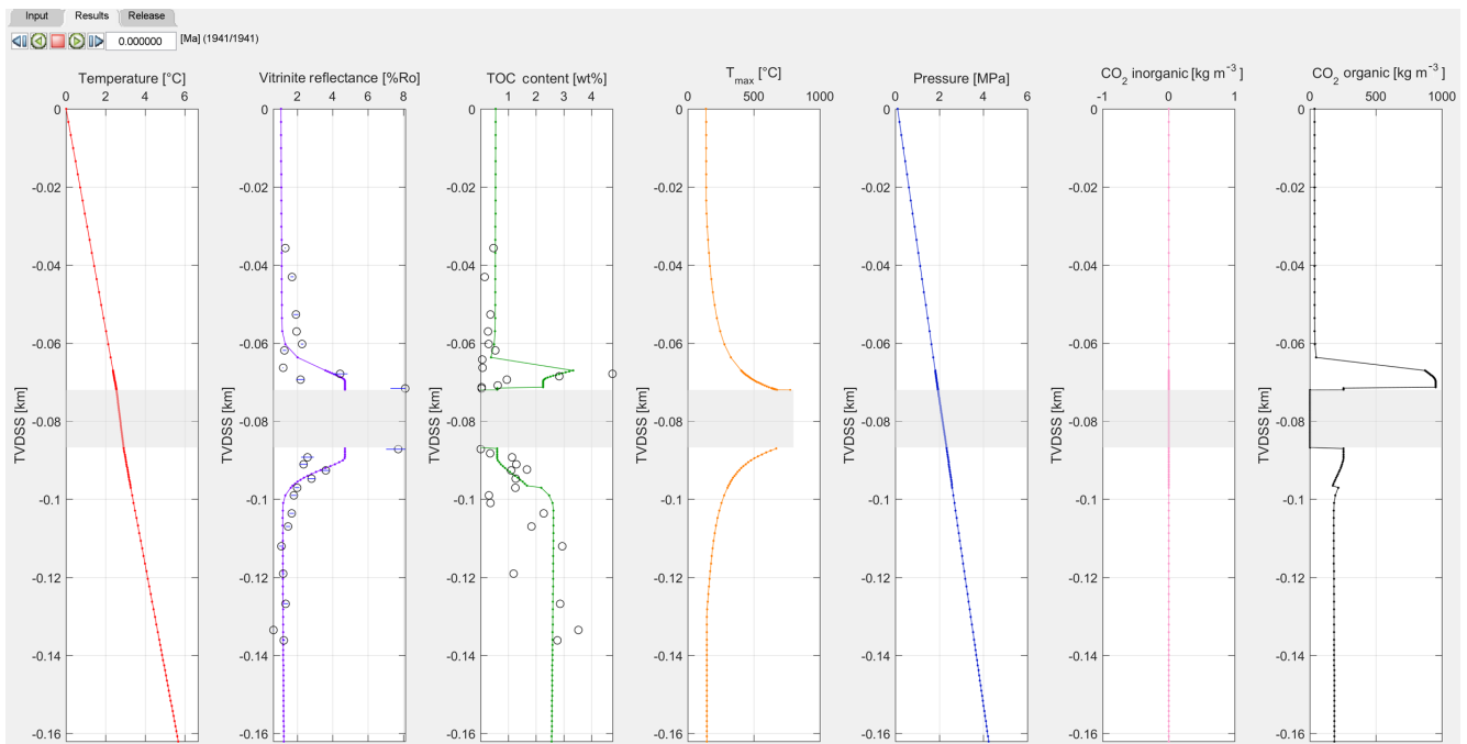
Figure 9. Results tab at the end of the simulation time for KL1/78 shows a good match to present-day TOC and VR values.
