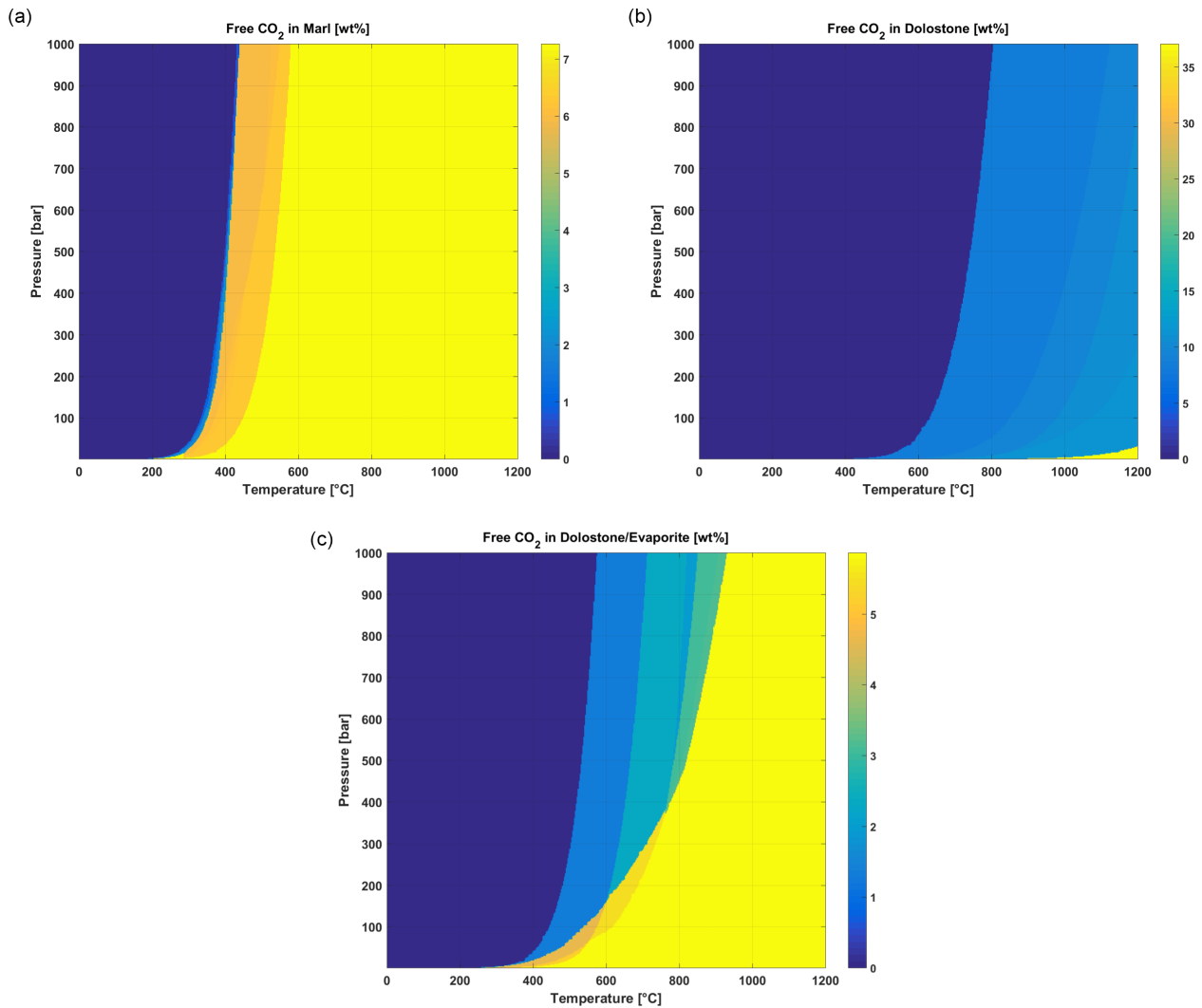
Figure 1. Phase diagrams generated by Perple_X showing the amounts of inorganic CO 2 liberated with respect to temperature and pressure for marl (a), dolostone (b) and dolostone/evaporite (c).
