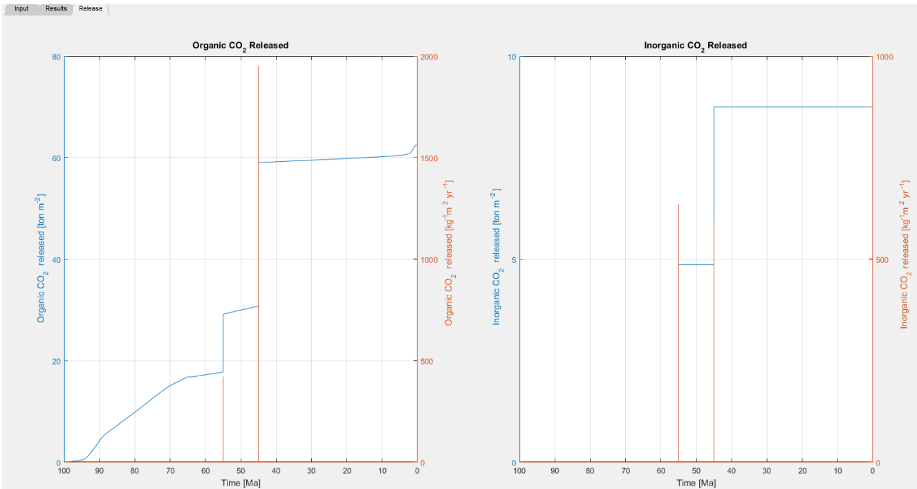
Figure 4. Snapshot of the release tab generated for a hypothetical sedimentary column with two sill intrusions and three eroded layers. Right-clicking any curve allows the user to copy curve data.
