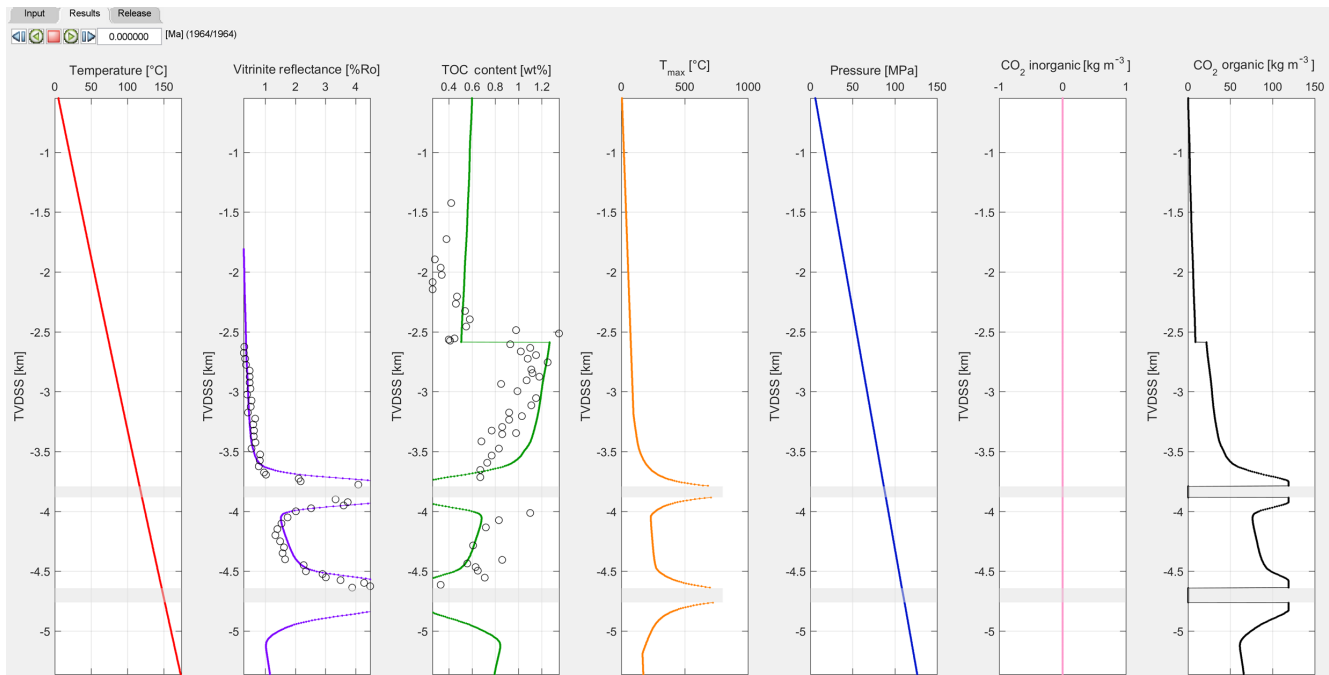
Figure 7. Results tab at the end of the simulation time for the Utgard High example. The present-day VR and TOC values (circles) show a good match with the model results.
