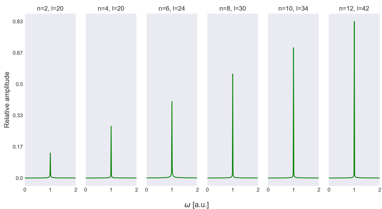
Figure 10.4: Fourier transform of expected value of dipole moment for a one-dimensional quantum dot with different number of electrons n = \{2, 4, 6, 8, 10\} with respective number of spin-orbitals l = \{20, 20, 24, 30, 34, 42\} . The intensity of the spectral lines are computed relative to the largest system ( n = 12 ), and are dimensionless.
