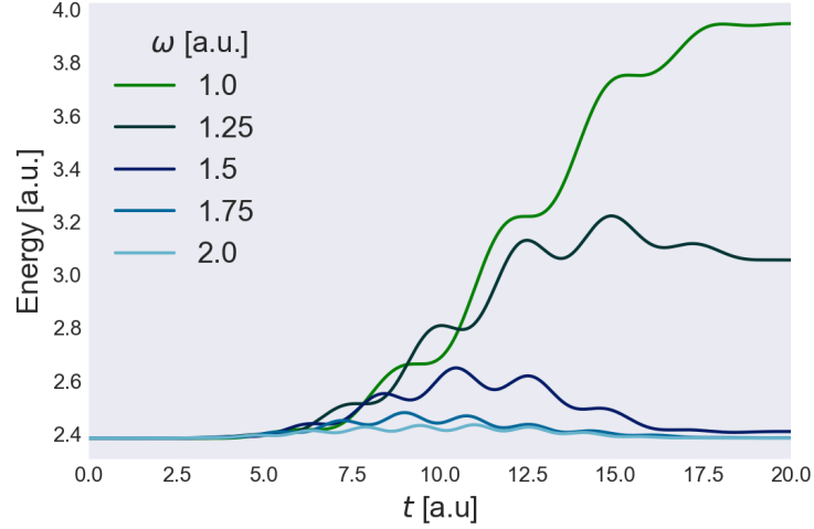
Figure 10.5: Time-dependent energy of a one-dimensional quantum dot with oscillator frequency \Omega = 1 a.u. and n = 2 electrons. The quantum dot is influenced by an oscillating field of different frequencies \omega \in \{1.0, 1.25, 1.5, 1.75, 2.0\} in atomic units with a maximum intensity of E_{\max} = 0.25 a.u.
