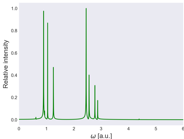
Figure 9.4: Dipole spectrum of helium computed with OATDCCD. The intensity of the spectral lines is in relative dimensionless units. The ground state of the system is excited by an oscillating field with strength E_{\max} = 10 a.u. and frequency \omega = 2.8736 a.u. for t_d = 5 a.u. The system is developed in time for a total of T = 1500 a.u. A cc-pVDZ basis set has been used in the simulation.
