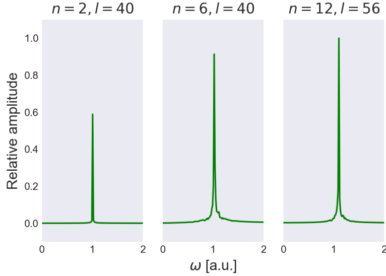
Figure 10.10: Fourier transform of the expected value of the dipole moment for a two-dimensional quantum dot with different number of electrons n = \{2, 6, 12\} and respective number of spin-orbitals l = \{40, 40, 56\} . The intensity of the spectra is computed relative to the largest system with n = 12 electrons.
