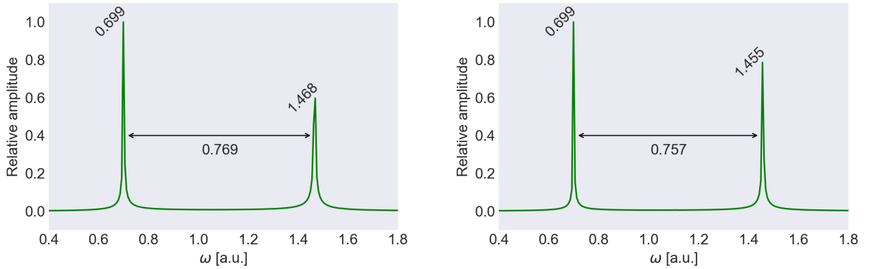
Figure A.13: Dipole spectrum of a quantum dot with n = 2 (left), and n = 4 electrons subjected to a magnetic field with Larmor frequency \omega_c = 0.75 a.u.. Both systems have base oscillator frequency \omega_0 = 1 a.u. and have been excited with an oscillating field with frequency \omega = 1 a.u. and intensity E_{\max} = 0.1 a.u.. The oscillating field had a period of t_d = 6\pi/\omega a.u. and the system was developed in time for a total of T = 1000 a.u..
