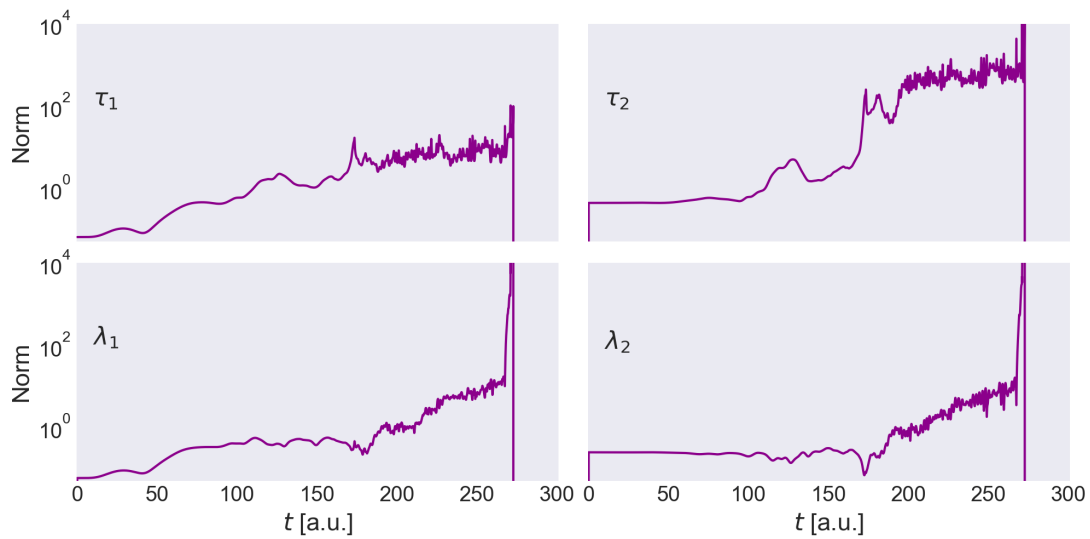
Figure 9.6: Norm of the amplitudes over time in the 1D beryllium atom, computed with TDCCSD. We see unreasonably high amplitude norms.
