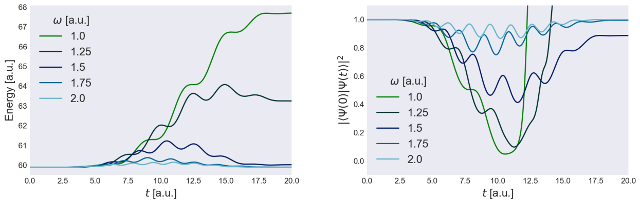
Figure A.8: Time-dependent energy (left) and ground state probability (right) of a one-dimensional harmonic oscillator with \Omega = 1 a.u. and n = 8 electrons under the influence of a oscillating electric field of different frequencies \omega \in \{1.0, 1.25, 1.5, 1.75, 2.0\} in atomic units with maximum field strength E_{\max} = 0.25 a.u. and l = 40 spin-orbitals.
