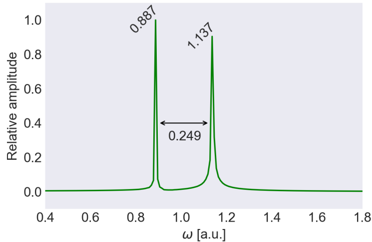
Figure 10.19: Dipole spectrum of a quantum dot with n = 4 electrons and base frequency \omega_0 = 1 a.u., subjected to a magnetic field with the Larmor frequency \omega_c = 0.25 a.u. The system was excited with a laser field with frequency \omega = 1 a.u. and intensity E_{\max} = 0.1 a.u. for t_d = 6\pi/\omega a.u. This simulation broke down after a total time of T \approx 700 a.u., but the data collected up to this point was sufficient get the desired result.
