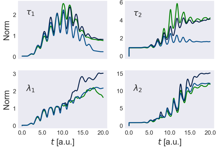
Figure 10.9: Norm of amplitudes, \tau_1 , \tau_2 , \lambda_1 and \lambda_2 (from CCSD, see section B.4) computed with the TDCCSD method in an n = 12 electron two-dimensional quantum dot influenced by an oscillating field with frequency \omega = 2 a.u., and intensity E_{\max} = 1 a.u. The simulation was run for T = 20 a.u., for several number of spin-orbitals l = \{42, 56, 72\} .
