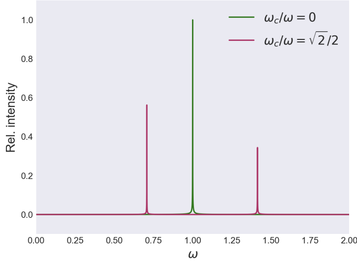
Figure 10.17: Spectrum of a single-electron two-dimensional quantum dot both with and without a magnetic field.
