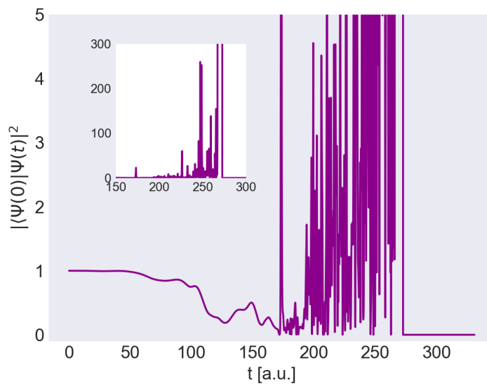
Figure 9.7: Probability of being in the ground state over time |\langle \Psi(0) | \Psi(t) \rangle|^2 , in dimensionless units, for the 1D beryllium atom, computed with TDCCSD. We see unreasonable probabilities.
