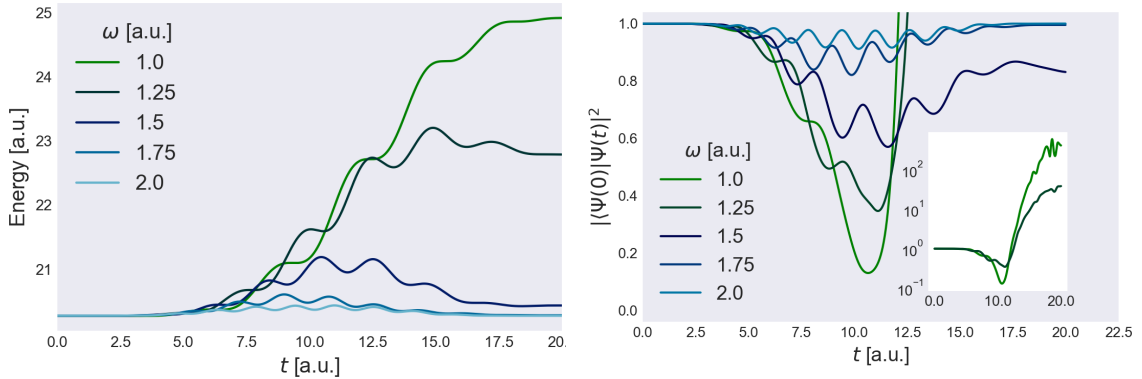
Figure 10.12: Time dependent energy (left) and ground state probability |\langle \Psi(0) | \Psi(t) \rangle|^2 (right) for a two-dimensional quantum dot with n = 6 electrons. The quantum dot is affected by an oscillating field of different frequencies \omega \in \{1.0, 1.25, 1.5, 1.75, 2.0\} in atomic units with a maximum intensity E_{\max} = 0.25 a.u. The confining harmonic potential has frequency \Omega = 1 a.u.
