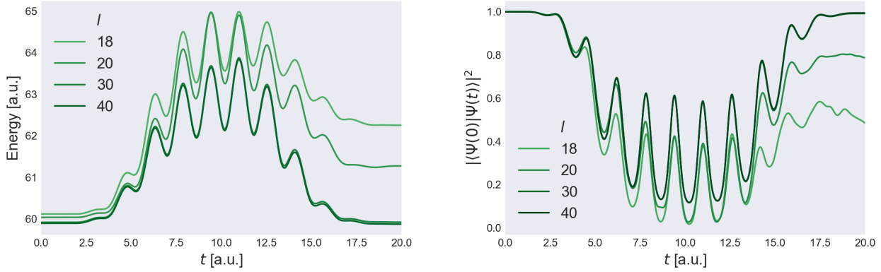
Figure A.7: Time-dependent energy (left) and ground state probability (right) of a one-dimensional harmonic oscillator with \Omega = 1 a.u. and n = 10 electrons under the influence of a oscillating electric field of frequency \omega = 2\Omega = 2 a.u. and field strength E_{\max} = 1 a.u., for different number of spin-orbitals l = \{18, 20, 30, 40\} .
