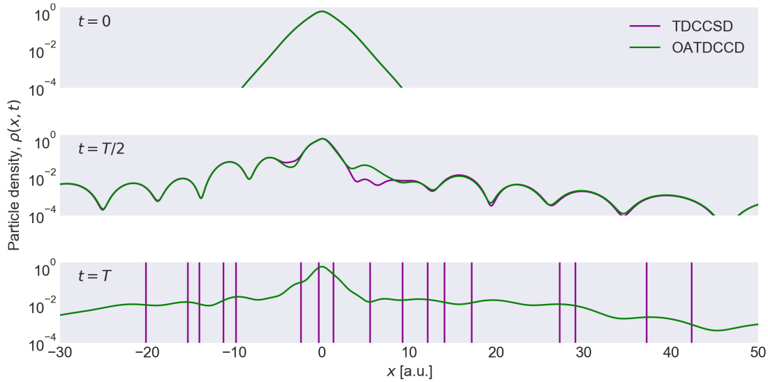
Figure 9.5: Snapshots of the dimensionless electron density \rho(x, t) in the 1D beryllium atom at t = 0 , t = T/2 and T , where T = 331 a.u., computed with TDCCSD and OATDCCD.
