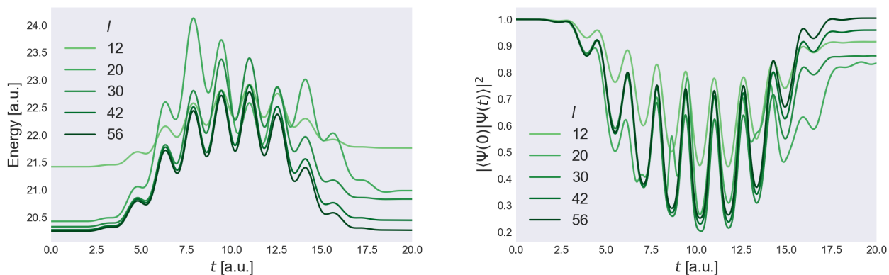
Figure A.11: Time-dependent energy (left) and ground state probability (right) of a two-dimensional harmonic oscillator with \Omega = 1 a.u. and n = 6 electrons under the influence of a oscillating electric field of frequency \omega = 2\Omega = 2 a.u. and field strength E_{\max} = 1 a.u., for different number of spin-orbitals l = \{12, 20, 30, 42, 56\} .
