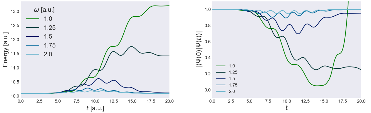
Figure A.2: Time-dependent energy (left) and ground state probability (right) of a one-dimensional harmonic oscillator with \Omega = 1 a.u. and n = 4 electrons under the influence of a oscillating electric field of different frequencies \omega \in \{1.0, 1.25, 1.5, 1.75, 2.0\} in atomic units with maximum field strength E_{\max} = 0.25 a.u. and l = 30 spin-orbitals.
