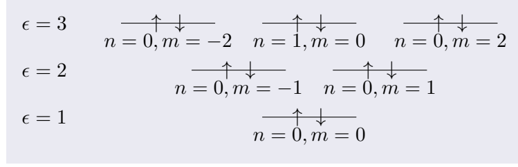
Figure 7.2: The lowest three energy levels in the two-dimensional quantum dot. Each arrow represents a spin up or a spin down state with the quantum numbers n and m as listed below. This pattern goes on indefinitely with the addition of one bar (two oscillators) per level.
