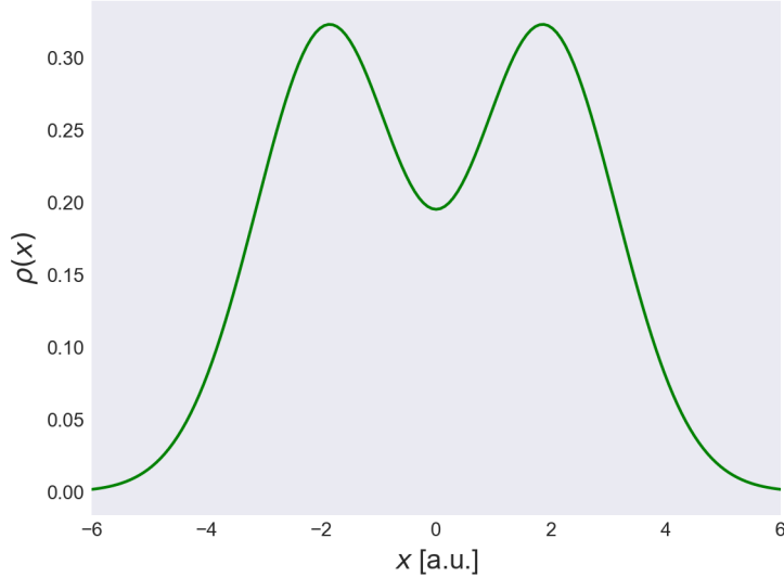
Figure 9.2: Electron density \rho(x) in dimensionless units for the ground state wavefunction of a quantum dot with n = 2 electrons and l = 20 spin-orbitals in the basis set computed with CCSD. This plot corresponds precisely to figure 1 of Zanghellini et al. [93].
