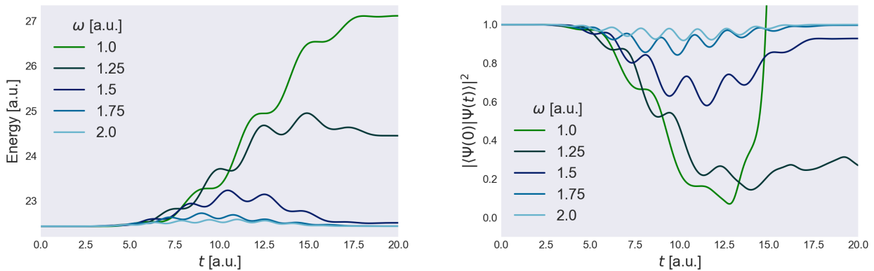
Figure A.4: Time-dependent energy (left) and ground state probability (right) of a one-dimensional harmonic oscillator with \Omega = 1 a.u. and n = 6 electrons under the influence of a oscillating electric field of different frequencies \omega \in \{1.0, 1.25, 1.5, 1.75, 2.0\} in atomic units with maximum field strength E_{\max} = 0.25 a.u. and l = 30 spin-orbitals.
