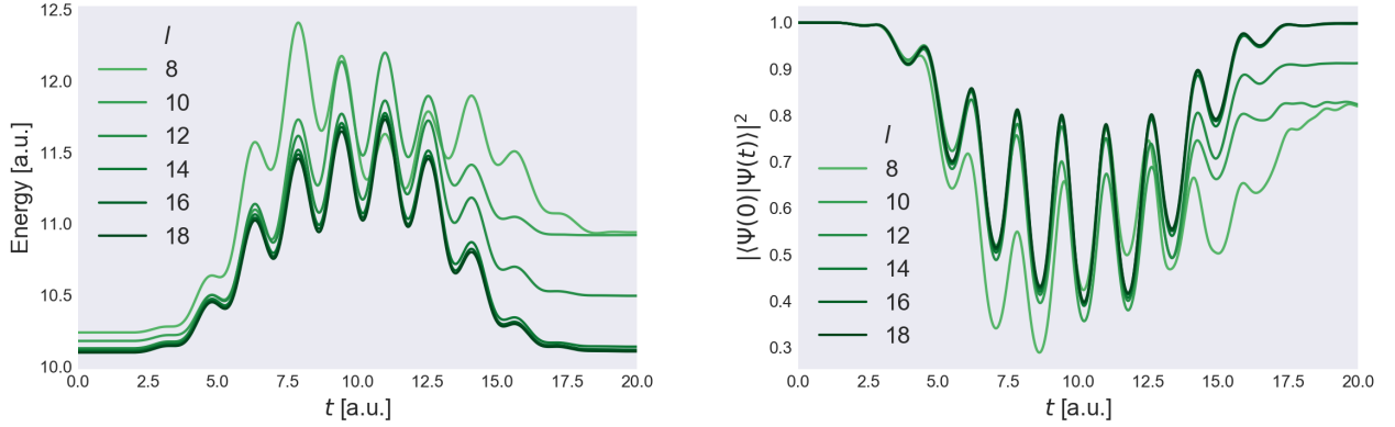
Figure A.1: Time-dependent energy (left) and ground state probability (right) of a one-dimensional harmonic oscillator with \Omega = 1 a.u. and n = 4 electrons under the influence of a oscillating electric field of frequency \omega = 2\Omega = 2 a.u. and field strength E_{\max} = 1 a.u., for different number of spin-orbitals l = \{8, 10, 12, 14, 16, 18\} .
