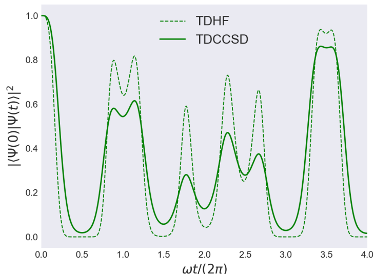
Figure 9.3: Probability of being in the ground state |\langle \Psi(0) | \Psi(t) \rangle|^2 using both TDHF and TDCCSD, for a one-dimensional quantum dot with n = 2 particles and l = 20 spin-orbitals. The ground state probability and the derived frequency units \omega t / (2\pi) are dimensionless. This plot corresponds precisely to figure 2 of Zanghellini et al. [93].
