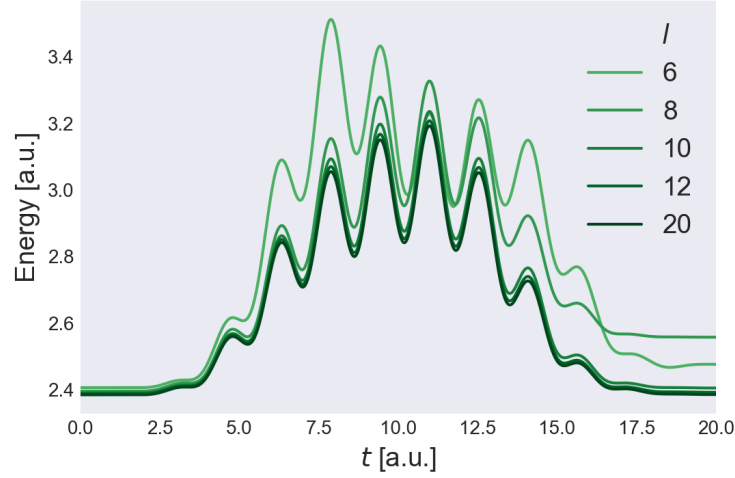
Figure 10.1: Time-dependent energy of a one-dimensional harmonic oscillator with n = 2 electrons under the influence of a laser field with maximum intensity E_{\max} = 1 a.u. and frequency \omega = 2 a.u., for different number of spin-orbitals l \in \{6, 8, 10, 12, 20\} . The oscillator frequency of the system is set to \Omega = 1 a.u.
