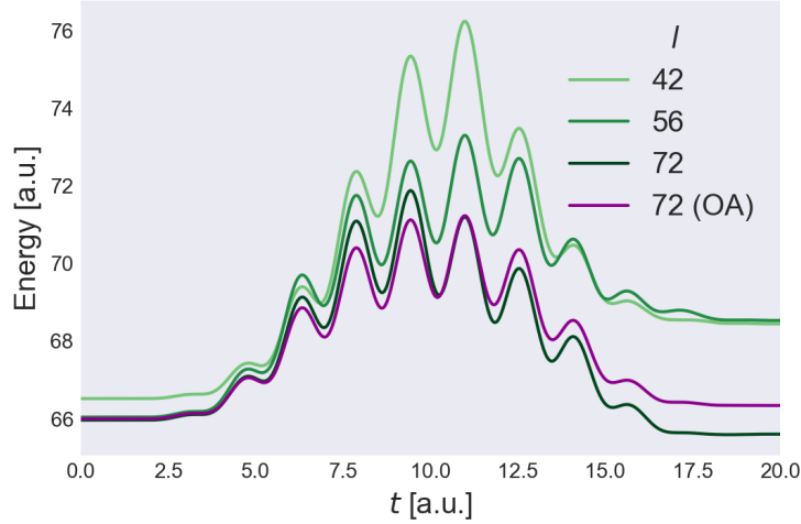
Figure 10.7: Time-dependent energy of a two-dimensional harmonic oscillator with n = 12 electrons under the influence of a laser field for different spin-orbitals l \in \{42, 56, 72\} .
