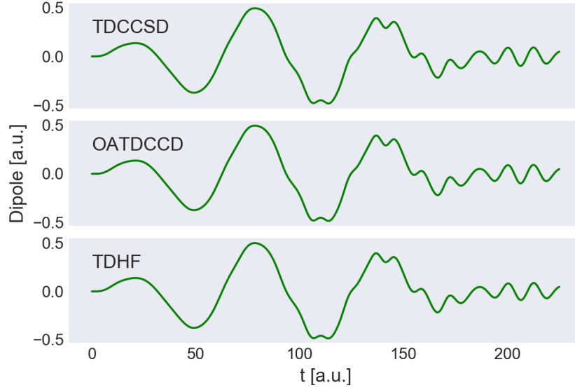
Figure 9.1: Instantaneous dipole for H_2 in an oscillating electric field of intensity E_{\max} = 0.07 a.u. and frequency \omega = 0.1 a.u., corresponding to 1.72 \times 10^{14} W cm ^{-2} and 456 nm, respectively. The 6-311++G(d,p) basis set has been used.
