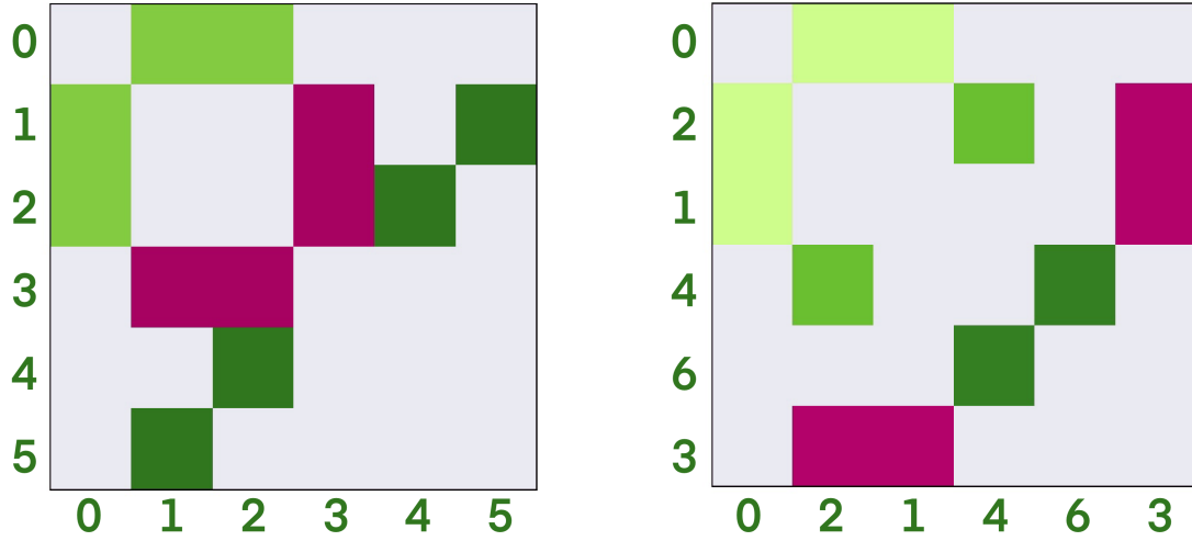
Figure 10.16: Transition matrix for a two-dimensional harmonic quantum dot with (left) and without (right) a magnetic field applied. The two systems both have a base oscillator frequency of \omega_0 = 1 a.u., while the right figure has a magnetic field applied with Larmor frequency \omega_c = \sqrt{2}/2 a.u. The effective confining potential is \Omega = 1 a.u. for the system represented in the left figure and \Omega \approx 1.118 a.u. for the system represented in the right figure.
