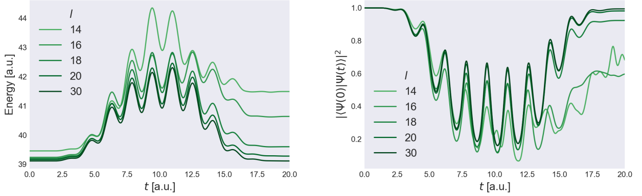
Figure A.5: Time-dependent energy (left) and ground state probability (right) of a one-dimensional harmonic oscillator with \Omega = 1 a.u. and n = 8 electrons under the influence of a oscillating electric field of frequency \omega = 2\Omega = 2 a.u. and field strength E_{\max} = 1 a.u., for different number of spin-orbitals l = \{14, 16, 18, 20, 30\} .
