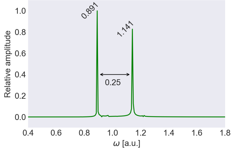
Figure 10.18: Dipole spectrum of a quantum dot with n = 2 electrons and base frequency \omega_0 = 1 a.u., subjected to a magnetic field with Larmor frequency \omega_c = 0.25 a.u. The system was excited with a laser field with frequency \omega = 1 a.u. and intensity E_{\max} = 0.1 a.u. for t_d = 6\pi/\omega a.u. then allowed to propagate in time for a total of T = 1000 a.u.
