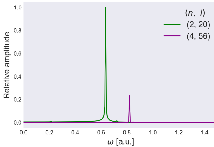
Figure 10.14: Dipole spectrum of two-dimensional double dot system with n = \{2, 4\} electrons and l = \{20, 56\} spin-orbitals. The double well systems have been subject to a laser pulse with frequency \omega = 0.43 a.u. and intensity E_{\max} = 0.1 a.u. The amplitudes have been computed relative to the highest amplitude value of the two systems.
