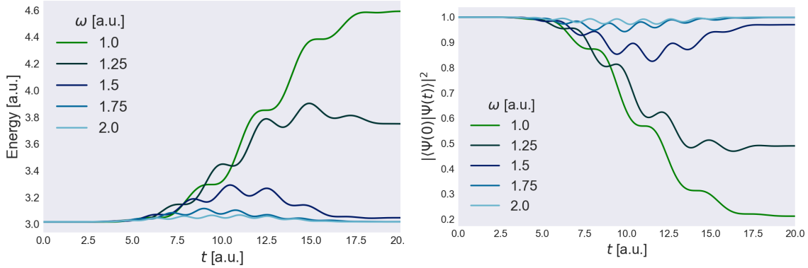
Figure 10.11: Time dependent energy (left) and ground state probability |\langle \Psi(0) | \Psi(t) \rangle|^2 (right) for a two-dimensional quantum dot with n = 2 electrons. The quantum dot is affected by an oscillating field of different frequencies \omega \in \{1.0, 1.25, 1.5, 1.75, 2.0\} in atomic units with a maximum intensity E_{\max} = 0.25 a.u. The confining harmonic potential has frequency \Omega = 1 a.u.
