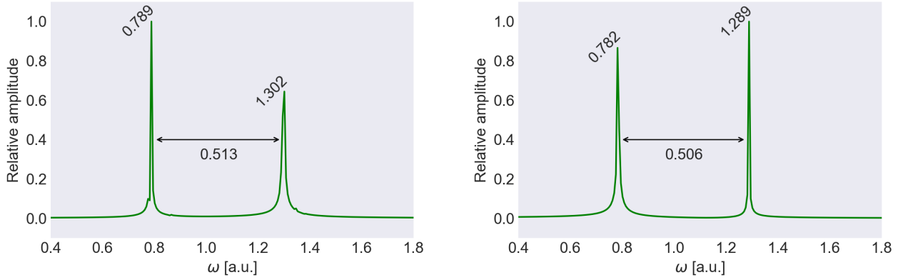
Figure A.12: Dipole spectrum of a quantum dot with n = 2 (left), and n = 4 electron subjected to a magnetic field with Larmor frequency \omega_c = 0.50 a.u.. Both systems have base oscillator frequency \omega_0 = 1 a.u. and have been excited with an oscillating field with frequency \omega = 1 a.u. and intensity E_{\max} = 0.1 a.u.. The oscillating field had a period of t_d = 6\pi/\omega a.u. and the system was developed in time for a total of T = 1000 a.u..
