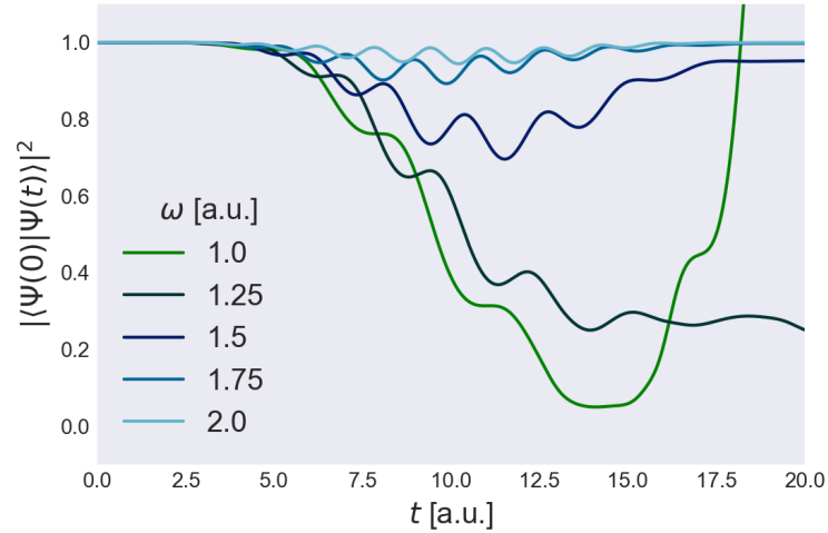
Figure 10.6: Time-dependent ground state probability |\langle\Psi(0)|\Psi(t)\rangle|^2 of a one-dimensional quantum dot with oscillator frequency \Omega = 1 a.u. and n = 2 electrons. The quantum dot is influenced by an oscillating field of different frequencies \omega \in \{1.0, 1.25, 1.5, 1.75, 2.0\} with a maximum intensity of E_{\max} = 0.25 a.u.
