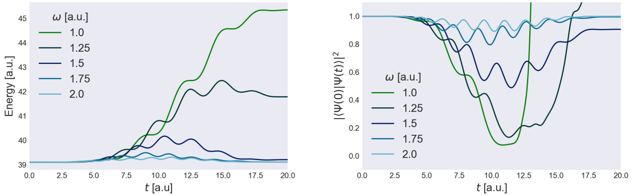
Figure A.6: Time-dependent energy (left) and ground state probability (right) of a one-dimensional harmonic oscillator with \Omega = 1 a.u. and n = 8 electrons under the influence of a oscillating electric field of different frequencies \omega \in \{1.0, 1.25, 1.5, 1.75, 2.0\} in atomic orbitals with maximum field strength E_{\max} = 0.25 a.u. and l = 36 spin-orbitals.
