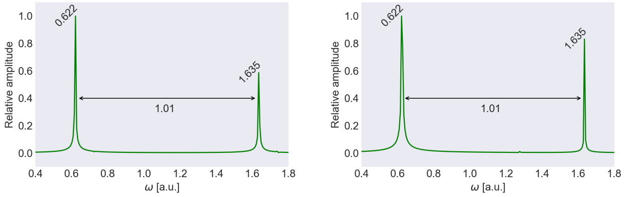
Figure A.14: Dipole spectrum of a quantum dot with n = 2 (left), and n = 4 electrons subjected to a magnetic field with Larmor frequency \omega_c = 1.0 a.u.. Both systems have base oscillator frequency \omega_0 = 1 a.u. and have been excited with an oscillating field with frequency \omega = 1 a.u. and intensity E_{\max} = 0.1 a.u.. The oscillating field had a period of t_d = 6\pi/\omega a.u. and the system was developed in time for a total of T = 1000 a.u..
