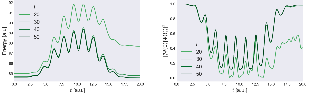
Figure A.9: Time-dependent energy (left) and ground state probability (right) of a one-dimensional harmonic oscillator with \Omega = 1 a.u. and n = 12 electrons under the influence of a oscillating electric field of frequency \omega = 2\Omega = 2 a.u. and field strength E_{\max} = 1 a.u., for different number of spin-orbitals l = \{20, 30, 40, 50\} .
