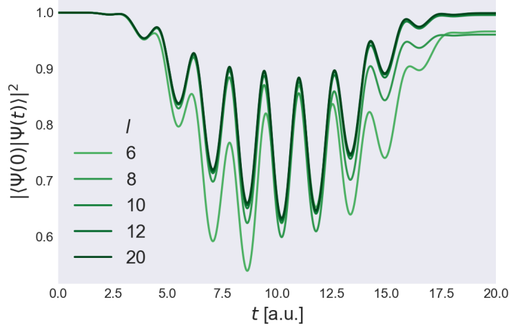
Figure 10.2: Dimensionless probability of being in the ground state |\langle \Psi(0) | \Psi(t) \rangle|^2 for a one-dimensional quantum dot with n = 2 electrons under the influence of a laser field with maximum intensity E_{\max} = 1 a.u. and frequency \omega = 2 a.u., for different number of spin-orbitals l \in \{6, 8, 10, 12, 20\} . The oscillator frequency of the system is set to \Omega = 1 a.u.
