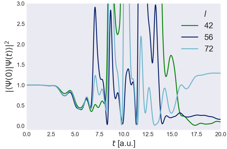
Figure 10.8: Dimensionless ground state probability |\langle\Psi(0)|\Psi(t)\rangle|^2 for a two-dimensional quantum dot with n = 12 electrons under the influence of a laser field for different number of spin-orbitals l = \{42, 56, 72\} .
