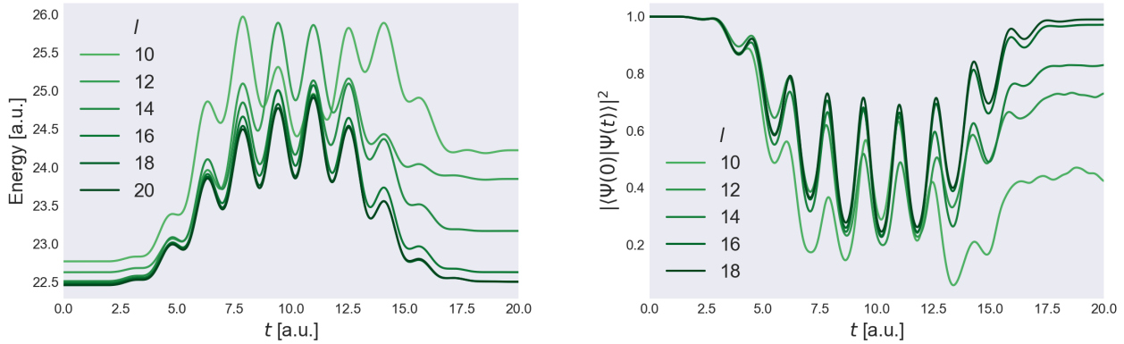
Figure A.3: Time-dependent energy (left) and ground state probability (right) of a one-dimensional harmonic oscillator with \Omega = 1 a.u. and n = 6 electrons under the influence of a oscillating electric field of frequency \omega = 2\Omega = 2 a.u. and field strength E_{\max} = 1 a.u., for different number of spin-orbitals l = \{10, 12, 14, 16, 18, 20\} .
