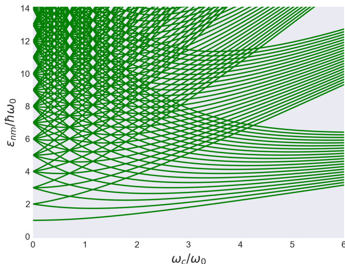
Figure 7.3: A few of the lowest eigenvalues \epsilon_{nm} for a two-dimensional quantum dot for transverse magnetic field of increasing strength. This plot of the single-particle energies form the Fock-Darwin spectrum. Some states for very high values of m are omitted to make the formation of Landau bands in strong fields more visible.
