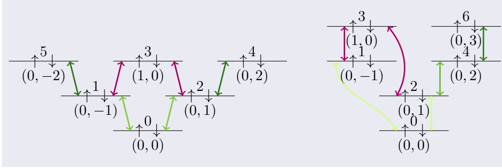
Figure 10.15: Shell structure of six lowest orbitals before (left), and after (right) a magnetic field is applied to a 2D quantum dot.
