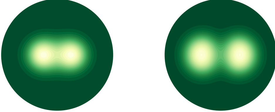
Figure 10.13: Ground state one-electron density for n = 2 electrons (left) and n = 4 electrons (right) for a double quantum dot. The number of spin-orbitals used in the two systems are l = 20 and l = 56 , respectively. The oscillator frequency of the systems is set to \Omega = 1 a.u., with a barrier strength of 2 and a harmonic oscillator mapping ratio of 2.
