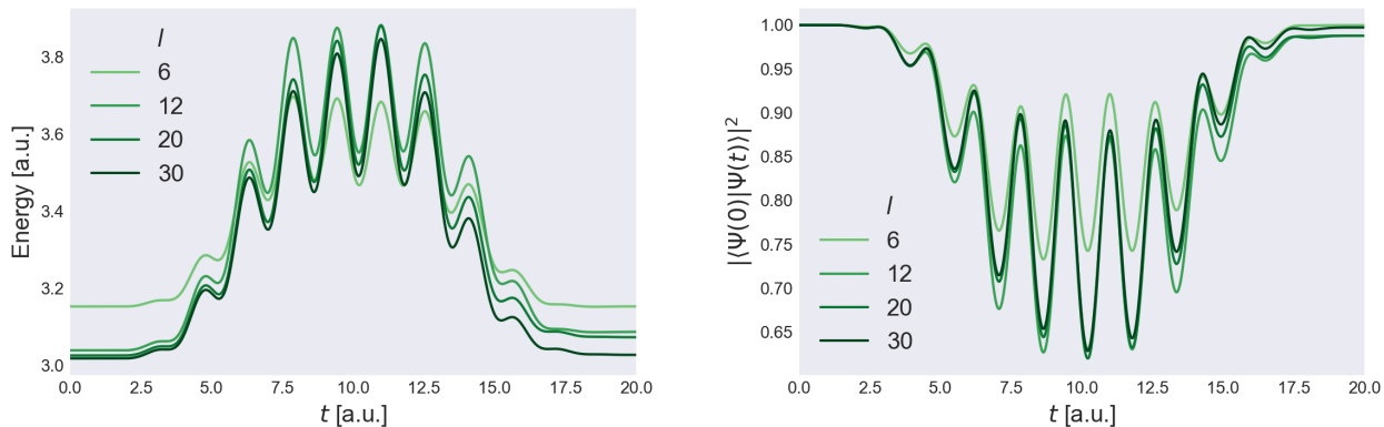
Figure A.10: Time-dependent energy (left) and ground state probability (right) of a two-dimensional harmonic oscillator with \Omega = 1 a.u. and n = 2 electrons under the influence of a oscillating electric field of frequency \omega = 2\Omega = 2 a.u. and field strength E_{\max} = 1 a.u., for different number of spin-orbitals l = \{6, 12, 20, 30\} .
