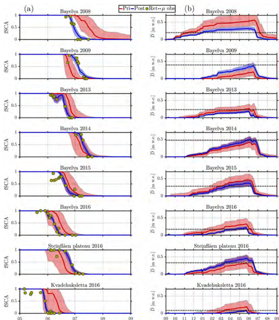
Figure 4. Time evolution of the prior (red) and ES-MDA ( N_a = 4 , N_e = 10^2 ) posterior (blue) fSCA (column a) and mean SWE ( \bar{D} ; column b); shading: 90th-percentile range; solid lines: ensemble median; yellow dots: assimilated MODIS and Sentinel-2 fSCA retrievals; dotted black line: independently observed peak mean SWE ( \mu ) from snow surveys (Sect. 2.2); x axis: months. These results are from a single run.
