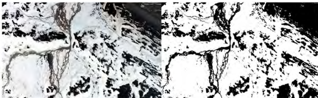
Figure 3.2: Left: Orthorectified true color time-lapse photograph over the Bayelva catchment on the 14.06.2017. Right: Resulting reference snow-cover map (black=bare, white=snow).
