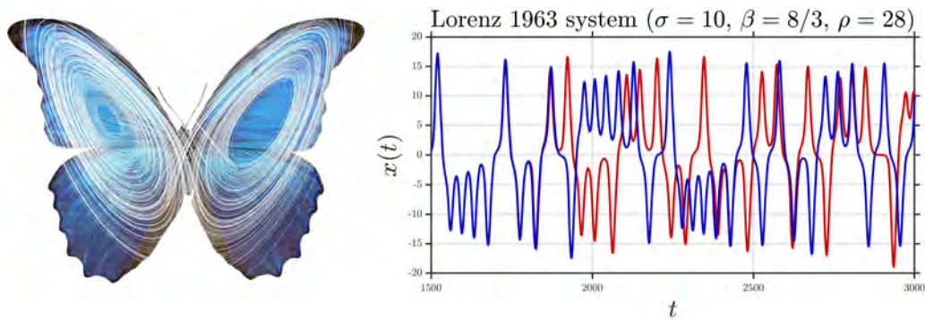
Figure 1.13: An illustration of the 'butterfly effect'. Left: Trajectory of the solution to the Lorenz (1963) system of equations in the x-z plane (white) overlaid on a Morpho didius butterfly. Right: The x -component of two solutions to the same system that vary by only 10^{-9} in the initial condition, they start to diverge after around 2000 time steps.
