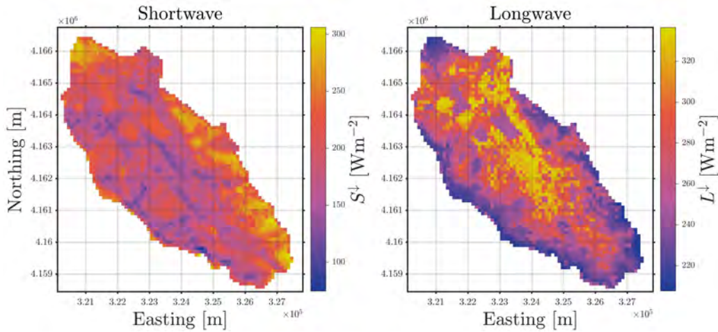
Figure 2.2: Topographically downscaled incoming shortwave radiation (left) and longwave radiation (right) averaged over for the 2018 snow season (October 2017 - September 2018) at the Mammoth Lakes basin in the Californian Sierra Nevada at 100 m resolution. The original coarse-scale fields were obtained from the ERA5 meteorological reanalysis. This high elevation basin is flanked by steep slopes on almost all sides and contains a relatively dense canopy in its center.
