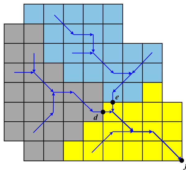
Figure 4. Discretization of catchment into sub-catchments and grids, and also delineation of streamflow routing (represented by blue lines) in the DEM-based rainfall-runoff model (DDRM). d, e, f represent the outlet of sub-catchments 1 (grey-shaded), 2 (light blue-shaded) and 3 (yellow-shaded), respectively.
