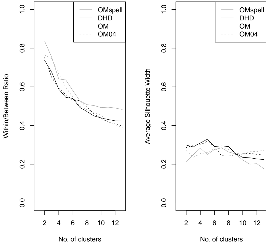
Fig. A.2: Within-between ratio (left panel) and Average Silhouette Width (right panel) for different sequencing techniques and cluster solutions.
