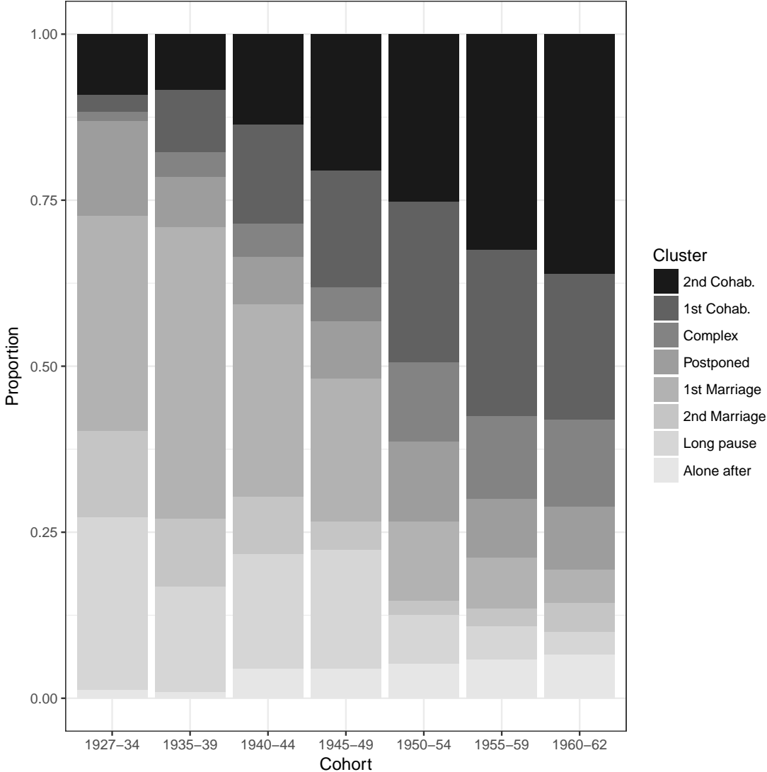
Fig. A.1: Distribution on cluster by cohort.
