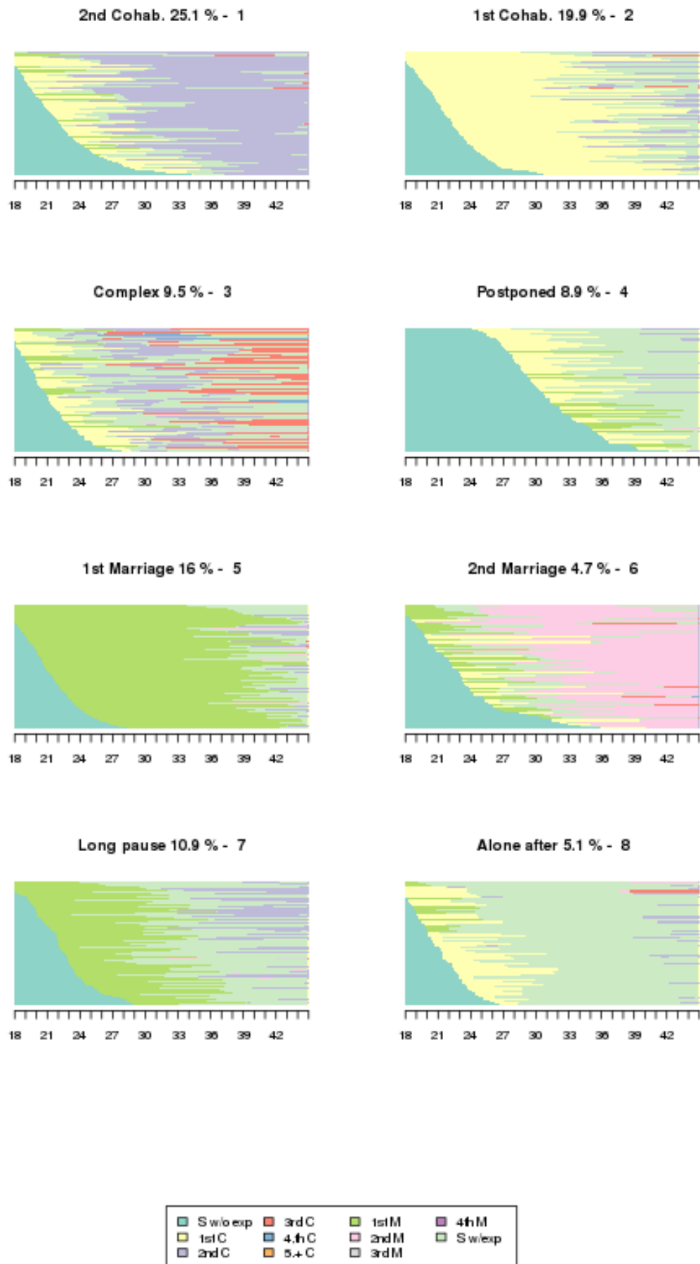
Fig. 1: Sequence Index Plot by cluster. 8-cluster solution obtained by OMspell. Results calculated and displayed for men and women jointly. The x-axis shows age in years. The y-axis shows proportions in each state in the current month.
