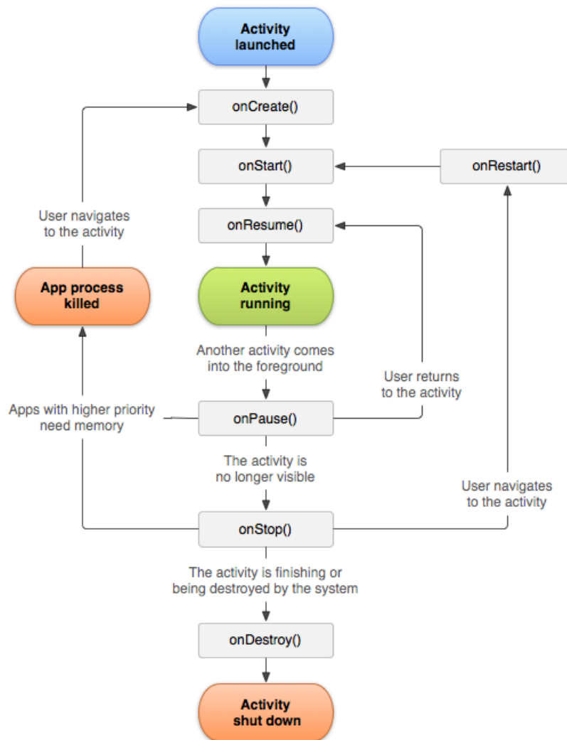
Figure 2.5: Android activity lifecycle [2].
