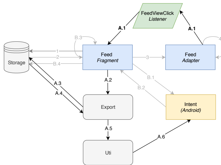
Figure 5.6: Implementation of the sharing action (A): exporting one or all records.
