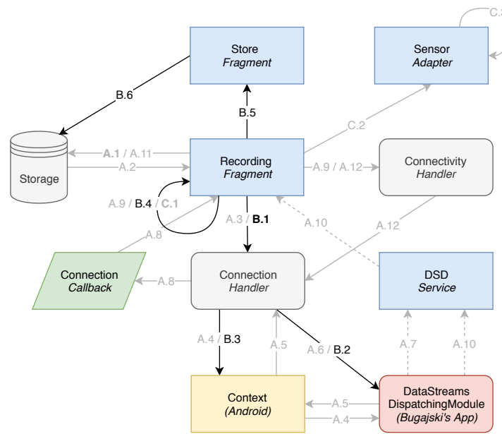
Figure 5.4: Implementation of the recording action (B): stop recording.
