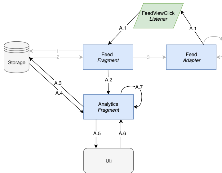
Figure 5.10: Implementation of the analytics action (A): display a graph for a single record.
