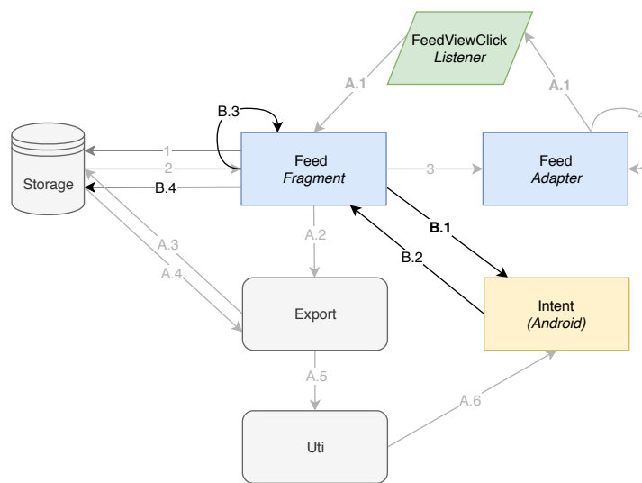
Figure 5.7: Implementation of the sharing action (B): import a record from the device.
