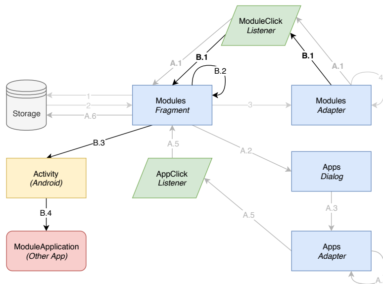
Figure 5.9: Implementation of the module action (B): launch a module.
