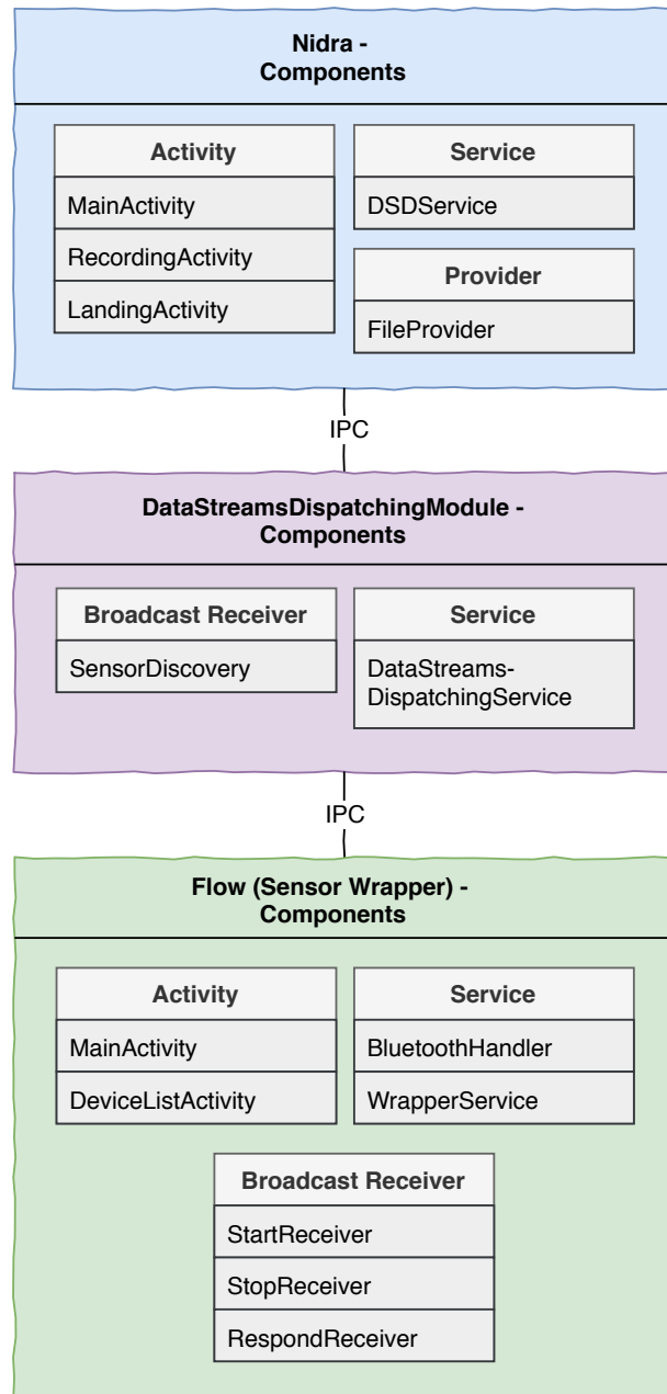
Figure 5.1: Applications components for the three individual Android applications in the project and IPC connection between them.
