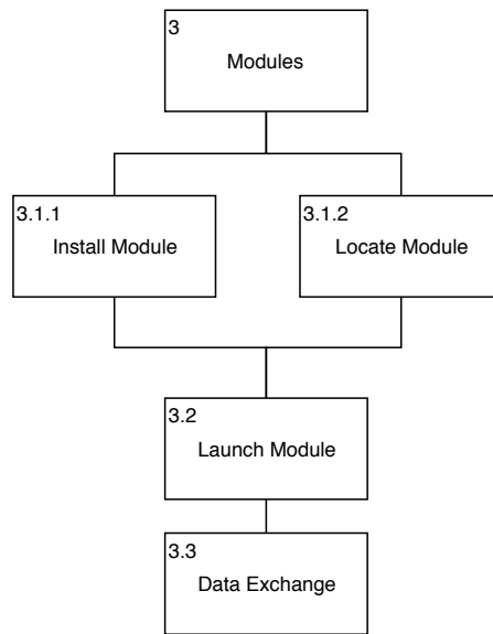
Figure 4.4: A design proposal for the structure of the modules concern.
