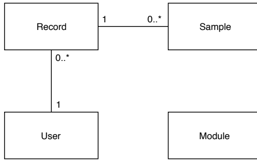
Figure 4.8: The data model and relationship for the entities in the application: a record has zero to many samples, while a sample only can have one record. A record can have one user, while a user can have many records. A module has no relationship with the other entities.
