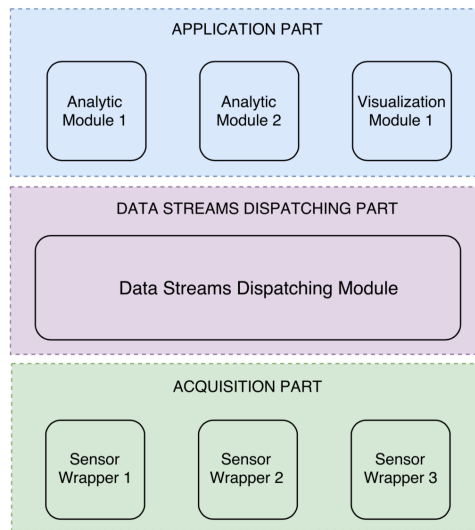
Figure 2.1: Structure of the CESAR project, separating functionality into three independent parts [12].
