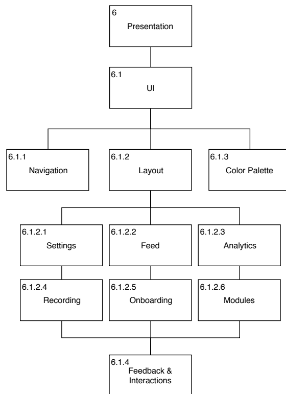
Figure 4.7: A design proposal for the structure of the presentation concern.
