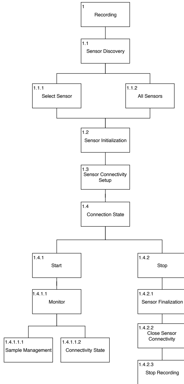
Figure 4.2: A design proposal for the structure of the recording concern.
