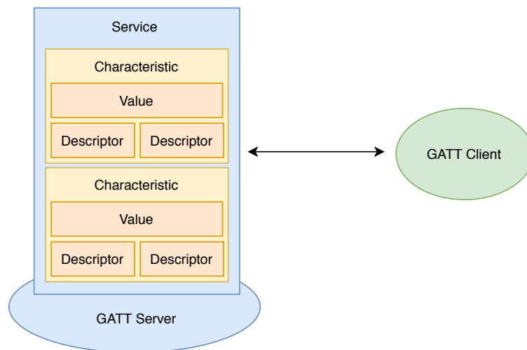
Figure 2.7: The structure of Bluetooth Low Energy; illustrating the GATT Server with a service containing many characteristics and its value, and the GATT client connecting with the GATT server.
