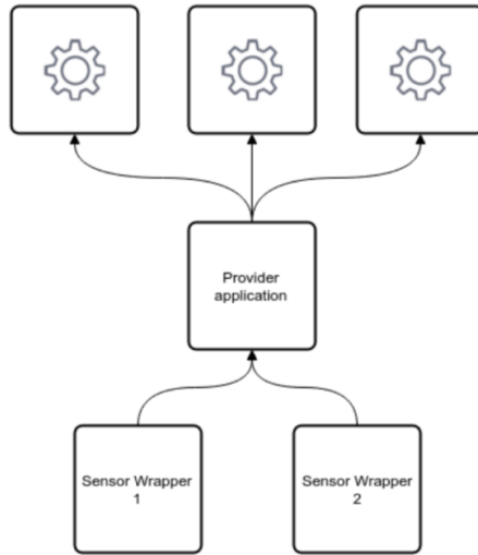
Figure 2.2: Sharing the collected data between multiple applications [25].
