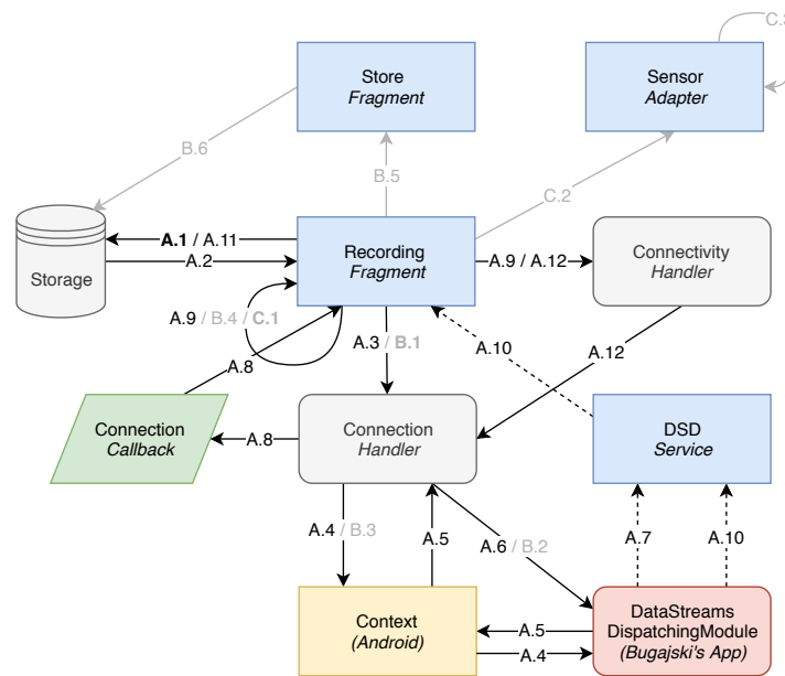
Figure 5.3: Implementation of the recording action (A): start recording.
