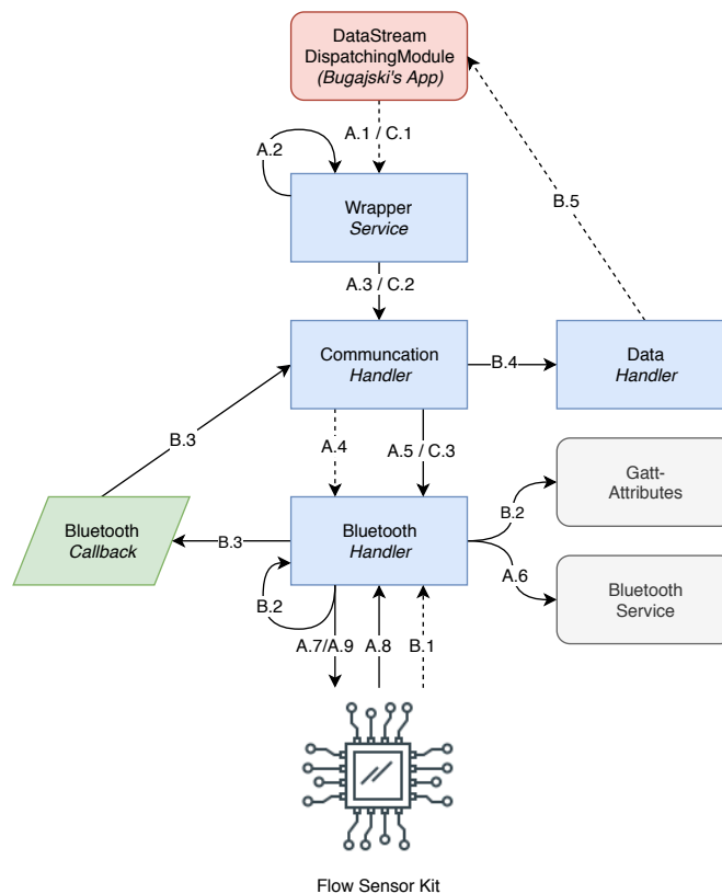
Figure D.2: Implementation of Flow sensor wrapper with the actions of: (A) start the data acquisition, (B) handle the samples from the sensor; (C) stop the data acquisition.
