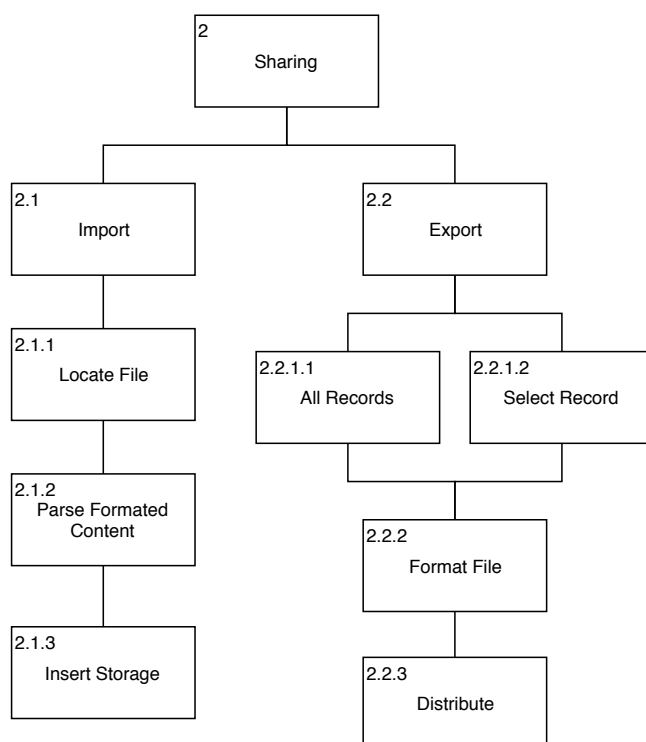
Figure 4.3: A design proposal for the structure of the sharing concern.
