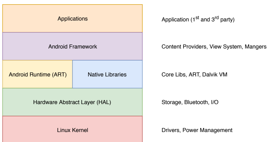
Figure 2.4: Android architecture stack, containing six major components.
