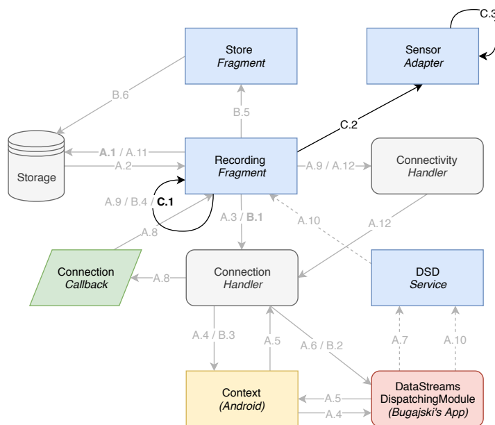
Figure 5.5: Implementation of the recording action (C): display recording statistics.
