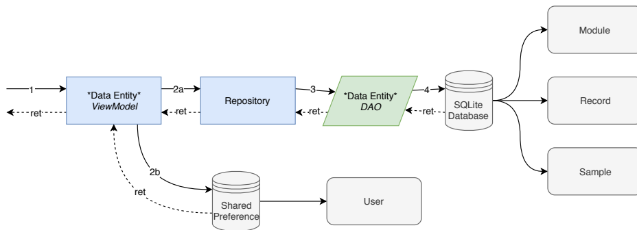
Figure 5.11: Implementation of the storage concern.
