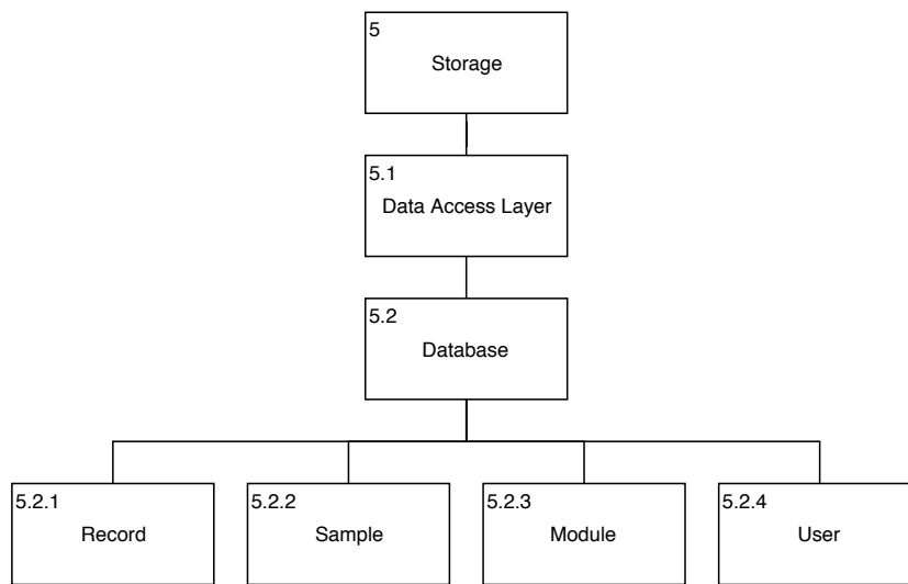
Figure 4.6: A design proposal for the structure of the storage concern.
