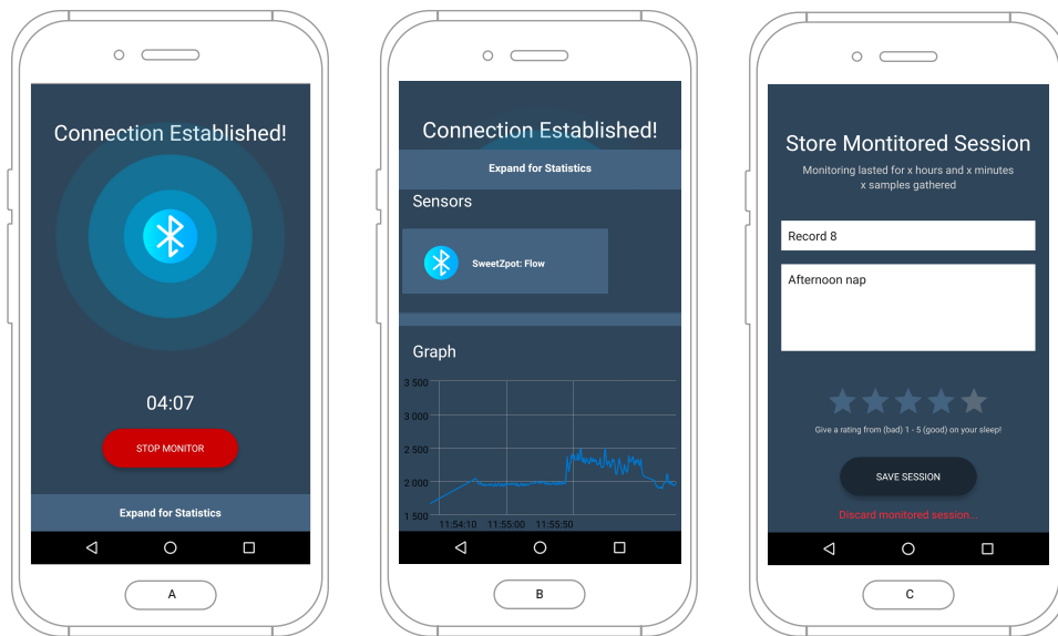
Figure 5.12: The recording screen displayed to the user: (A) during a recording, (B) statistics interface, and (C) stopping the recording.
