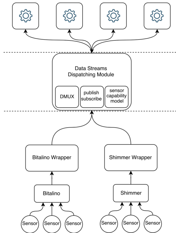
Figure 2.3: Sharing the collected data between multiple applications [12].
