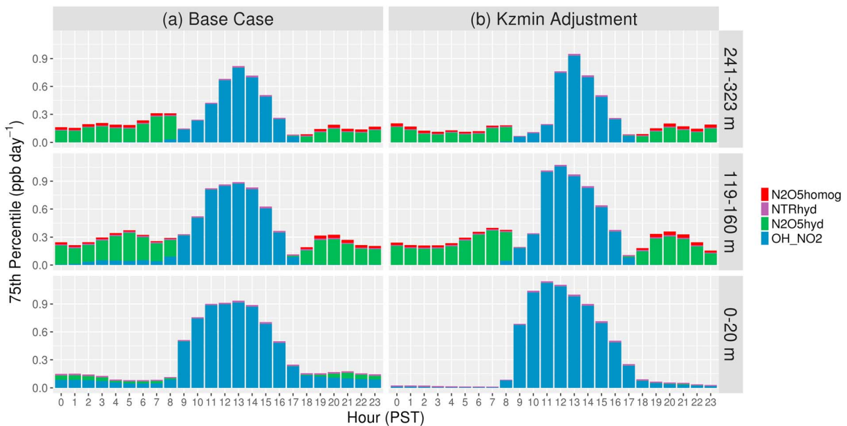
Figure 11. Hourly 75th percentile \text{HNO}_3 production rates by chemical pathway over Fresno for the (a) base simulation and (b) simulation with K_{z,\min} = 0.01 \text{ m}^2/\text{s} for model layers 1, 5, and 7 during January 17–22. \text{N}_2\text{O}_5\text{homog} : homogeneous gas phase reaction of \text{N}_2\text{O}_5 + \text{H}_2\text{O} ; \text{NTRhyd} : heterogeneous hydrolysis of organic nitrates; \text{N}_2\text{O}_5\text{hyd} : heterogeneous hydrolysis of \text{N}_2\text{O}_5 ; and \text{OH\_NO}_2 : reaction of \text{OH} + \text{NO}_2 .
