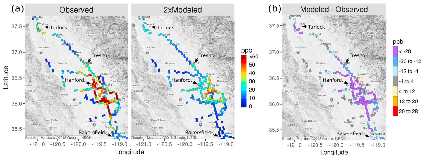
Figure 2. (a) Median observed and 2x median modeled NH 3 mixing ratio by CMAQ grid cell over all mobile ground laboratory sampling transects and (b) difference in median values. See text for description of grid cell median calculations.
