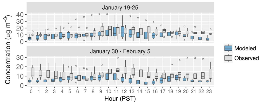
Figure 9. Hourly average modeled and measured \text{NO}_3^- distributions at Fresno ground site during two periods of interest. Boxes bracket the IQR, lines within the boxes represent the median, whiskers represent 1.5 times the IQR from either end of the box, and circles represent individual values less than and greater than the range of the whiskers.
