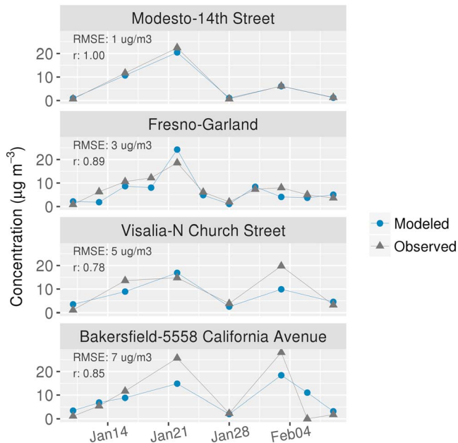
Figure 7. Comparison of 24-hr average PM_{2.5} NO_3^- predictions of CMAQ with routine monitoring measurements at sites shown in Figure 4b.
