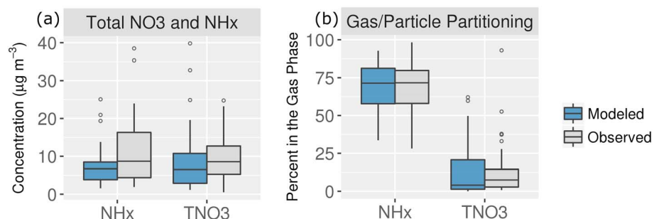
Figure 10. Modeled and measured concentrations of (a) TNO3 and \text{NH}_x and (b) percentage of total in the gas phase during 19–31 January at the Fresno ground site.
