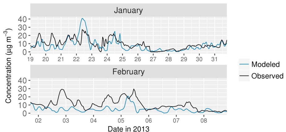
Figure 8. Comparison of model predictions of fine particle NO_3^- with PILS-IC measurements at the Fresno-Garland ground site.
