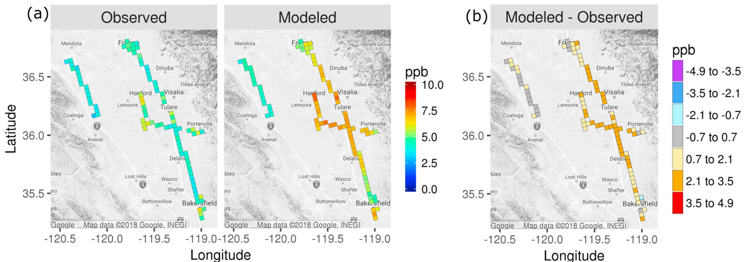
Figure 6. (a) Average modeled and measured TNO 3 within the modeled PBL by model grid cell over P-3B flights in January and February 2013 and (b) difference between modeled and measured TNO 3 .
