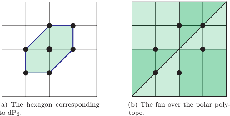
Figure 3.1: Toric description of \mathrm{dP}_6 .
