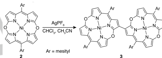
Scheme 2. Synthesis of \beta,\beta -linked dimer 3 .
