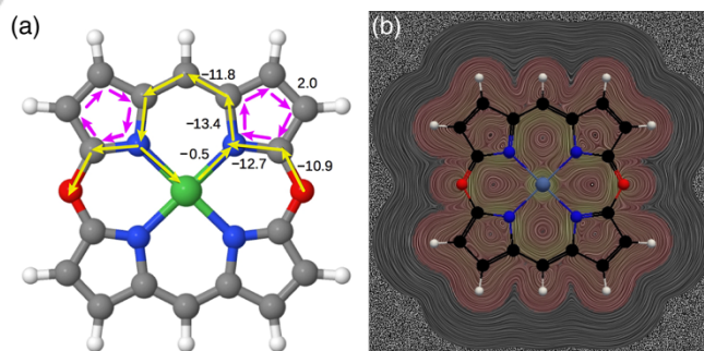
Figure 2. (a) Integrated total current strength susceptibility values obtained for selected bonds are given in nA/T. Diamagnetic currents are assumed to circle clockwise (magenta arrows), whereas paratropic ones circle in the opposite direction (yellow arrows). (b) Streamline visualization of the magnetically induced current density in a plane placed 1 Bohr below the molecular plane.
