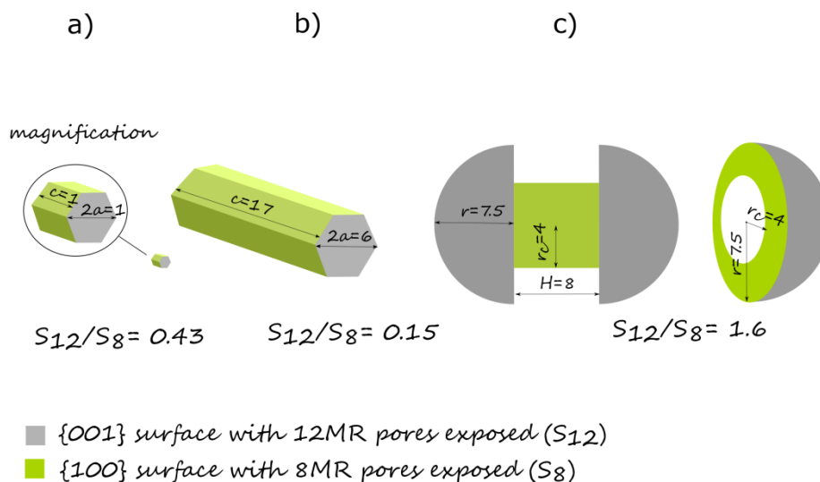
Figure 11. Qualitative model of idealized and simplified shapes of synthesized crystals: (a) OFF-S (b) OFF-O and OFF-H (c) OFF-B, which roughly estimate a contribution of 12MR and 8MR openings ( S_{12}/S_8 ).
