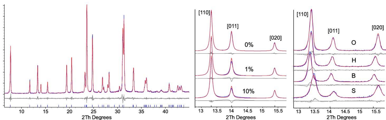
Figure 9. LeBail fit of experimental data (left) showing no anisotropic peak broadening. Full profile fit (performed in TOPAS) of the simulated data containing 0%, 1% and 10% stacking faults (middle). Full profile fit of the four OFF samples showing no evidence of stacking faults (right). Black curves correspond to simulated (middle) or observed data (right). Red and grey curves are the model and the difference curves respectively.
