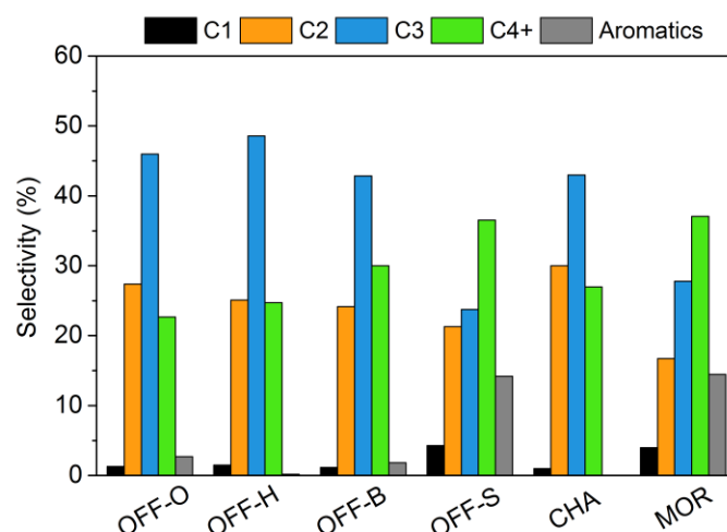
Figure 103. Comparison of product selectivities of four offretite catalysts to CHA (3-dimensional 8MR), and MOR (1-dimensional 12MR)
