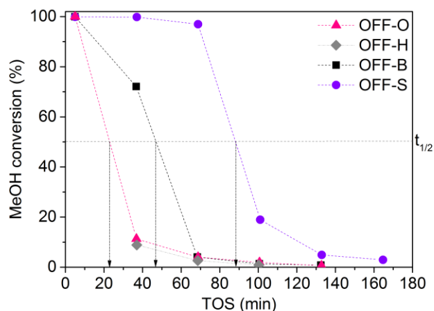
Figure 6. Methanol conversion versus time on stream at 400 °C and WHSV=2 \text{ g}_{\text{MeOH}}\text{g}_{\text{catalyst}}^{-1}\text{h}^{-1} for offretite catalysts with different morphology.
