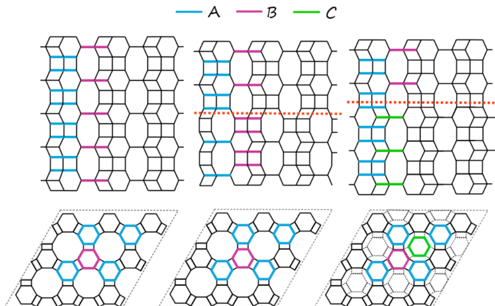
Figure 96. [100] (top row) and [001] (bottom row) projection of offretite framework. (Left column) The layer sequence AABAAB of offretite without twinning (ideal structure). (Middle column) proposed stacking fault leading to two twin domains without blocking the 12 ring channel; (right column) a stacking fault of the type known from OFF- ERI stacking disordered materials leading to two twin domains and a blocked 12 ring channels.
