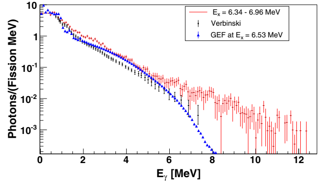
FIG. 10. A comparison of the ^{239}\text{Pu}(d, pf) PFGS measured at E_x \sim S_n (red), the PFGS for thermal-neutron-induced fission ^{239}\text{Pu}(n_{\text{th}}, f) from Verbinski et al. [15] (black points), and the calculations by GEF for J_{\text{rms}} = 8 and E_x = 6.35 (blue).
