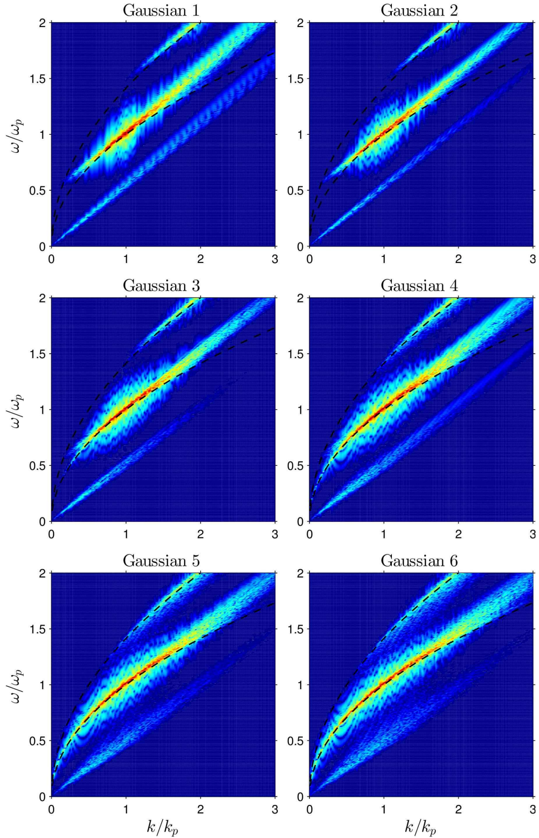
FIGURE 6. Wavenumber-frequency spectra of Gaussian 1–6 from simulations. Colour scale as in figure 4. Lower dashed curve; linear dispersion relation. Upper dashed curve; second harmonic dispersion shell.
