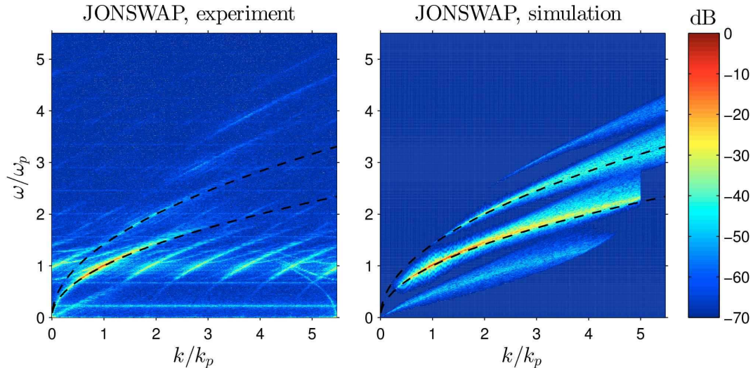
FIGURE 4. Wavenumber-frequency spectra from experiment (left) and simulation (right) with the JONSWAP wave field. Colour scale in dB relative to the peak. Lower dashed curve; linear dispersion relation. Upper dashed curve; second harmonic dispersion shell.
