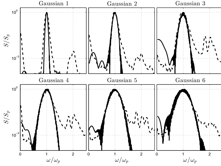
FIGURE 2. Feedback spectra of the actual wave maker motion; —. Frequency spectra measured at the probe closest to the wave maker; ---. Upper left to lower right subplot; Gaussian 1–6.
