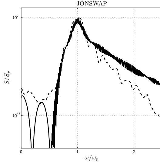
FIGURE 3. JONSWAP feedback spectrum of the actual wave maker motion; —. JONSWAP frequency spectrum measured at the probe closest to the wave maker; ---.
