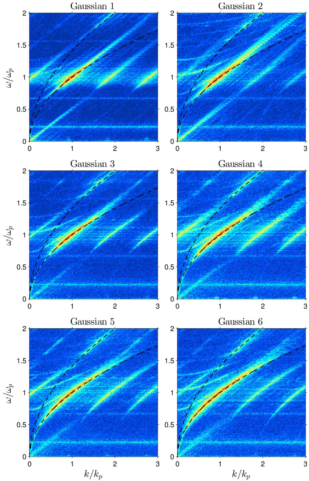
FIGURE 5. Wavenumber-frequency spectra of Gaussian 1–6 from experiments. Colour scale as in figure 4. Lower dashed curve; linear dispersion relation. Upper dashed curve; second harmonic dispersion shell.
