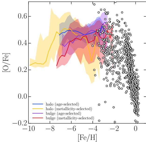
Figure 5. Median \alpha -enhancement [\text{O}/\text{Fe}] of accreted gas by stars in the four samples considered in this paper (solid curves) and 68 per cent scatter around the median (shaded regions). Blue and yellow curves and shaded regions describe properties of halo stars selected by age and metallicity, respectively. Bulge stars selected by age and metallicity are described, respectively, by purple and red curves. Open circles show [\alpha/\text{Fe}] measurements for halo and disc stars from the compilation by Shen et al. (2015). There is a good agreement between the [\alpha/\text{Fe}] for iron-poor stars and the accreted gas in our model.
